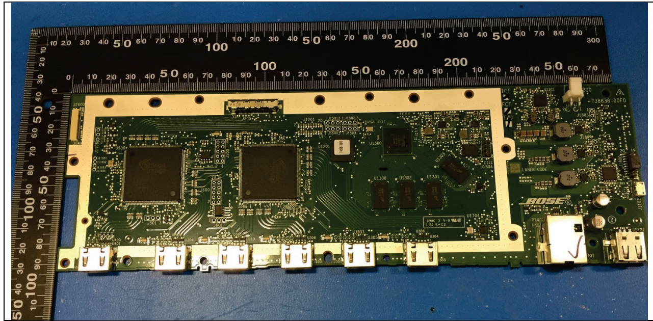
HDMI Board Top
