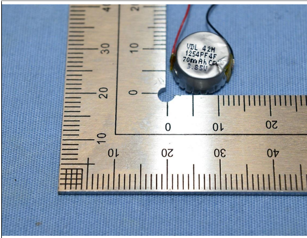
Battery VDL/1254PF4F
