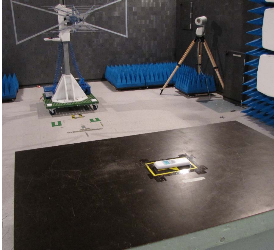
Radiated spurious emission 30-1000 MHz
