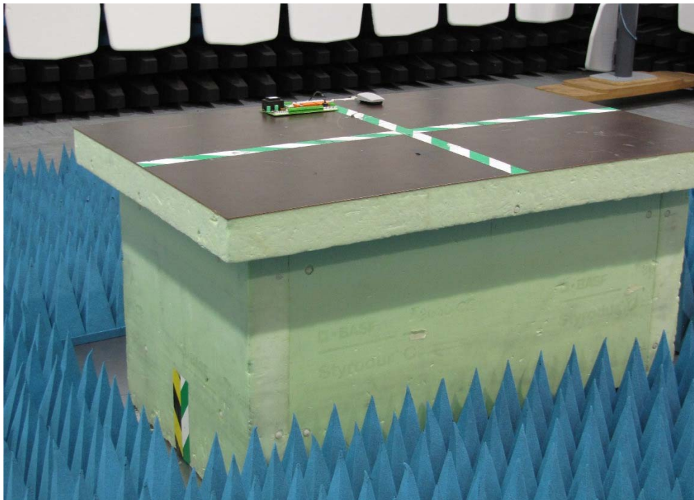
Radiated spurious emission above 1-10 GHz
