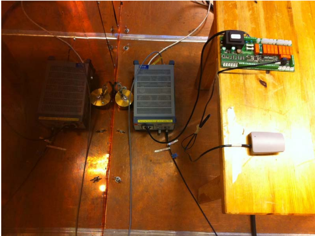
Conducted measurements from AC mains
