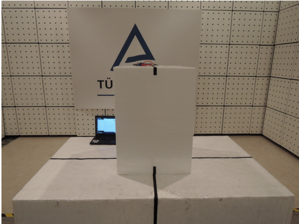
Photograph 5: Set-up for Spurious Emissions - IC (Back View)
