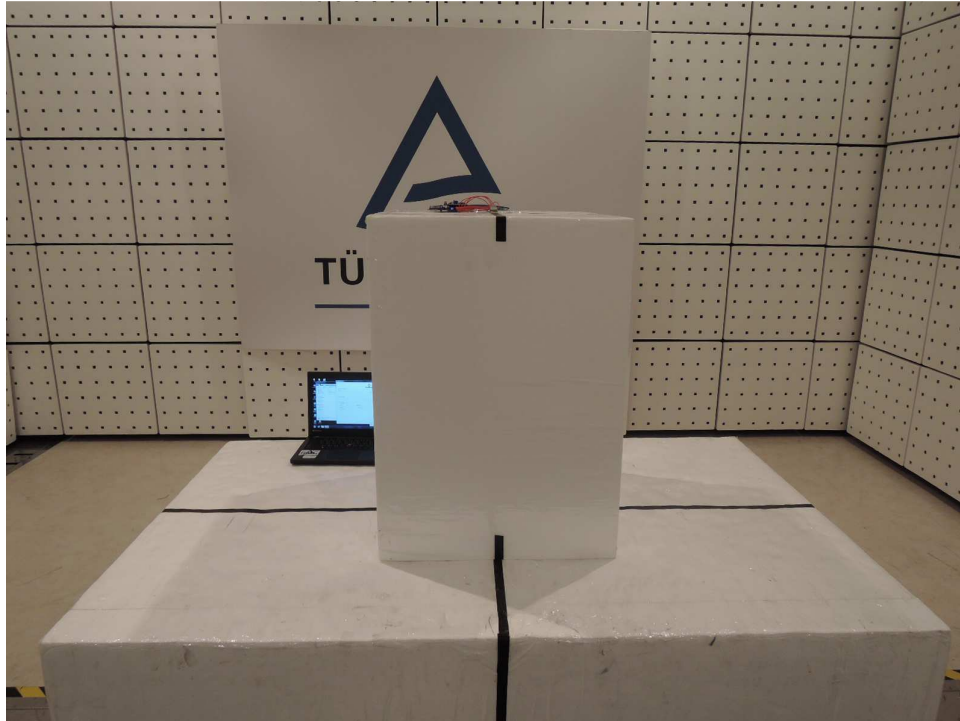
Photograph 5: Set-up for Spurious Emissions - IC (Back View)
