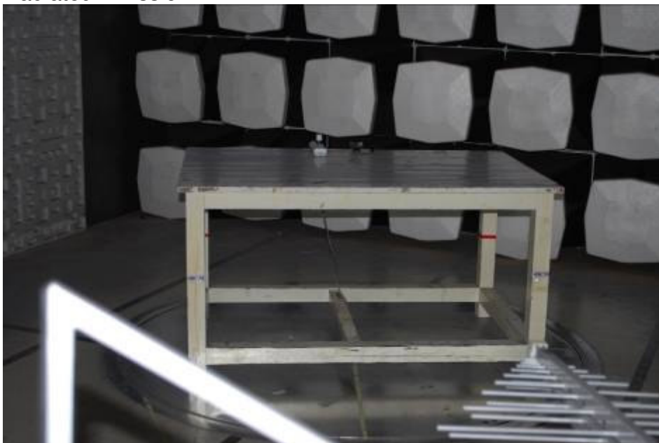
Radiated Emission
