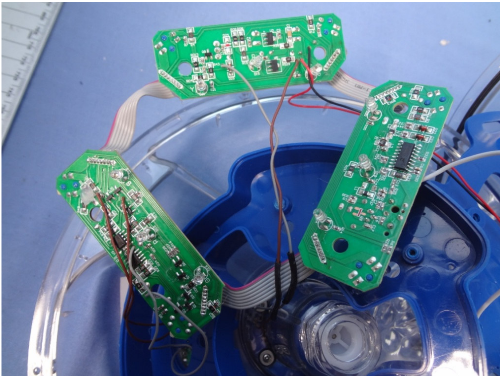
Internal of PCB Front Side
