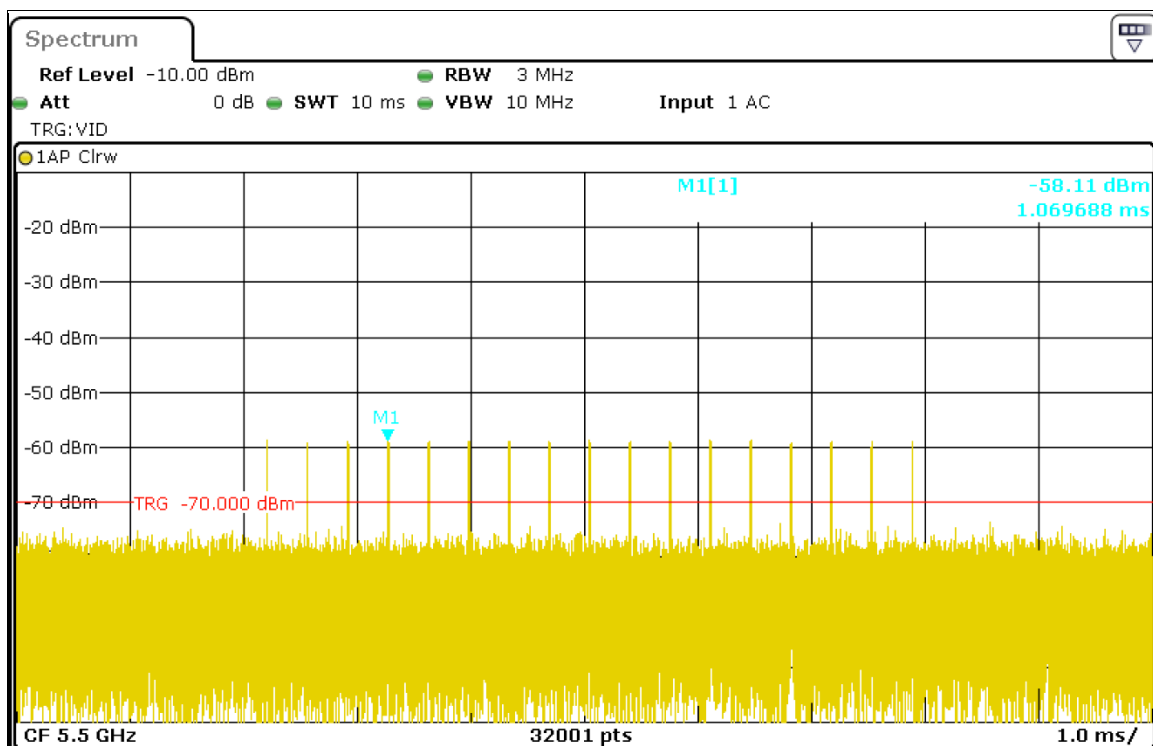
Radar Signal 3
