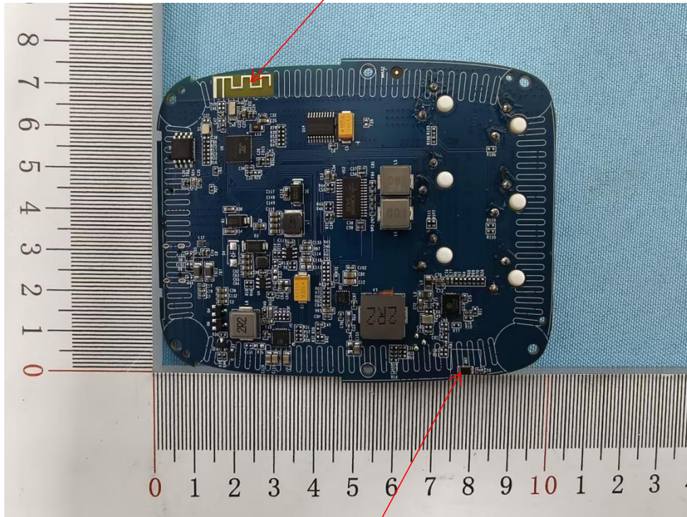
Microphone BT ANT RX
