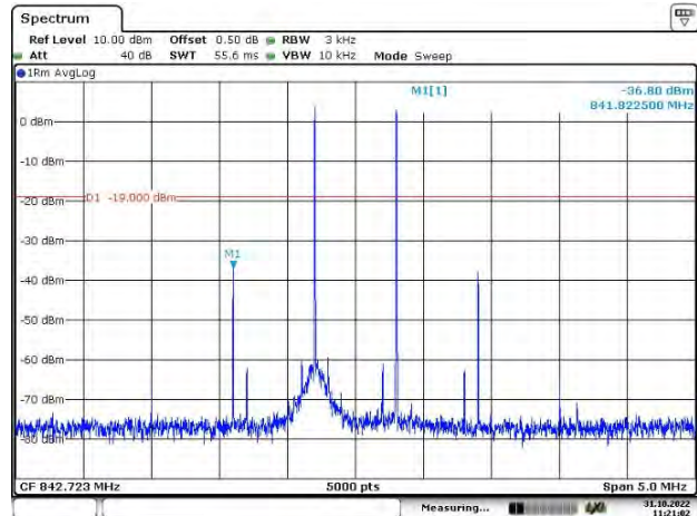
Cellular Band Uplink-Above AGC
