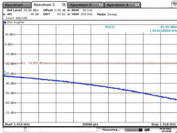
Right Side-WCDMA-Pre AGC
