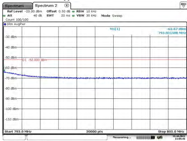
Upper 700 MHz Band-5
