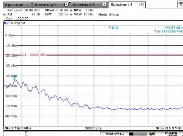
Right Side-GSM-Pre AGC
