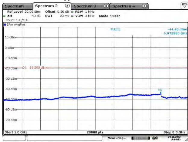
Upper 700 MHz Band-3
