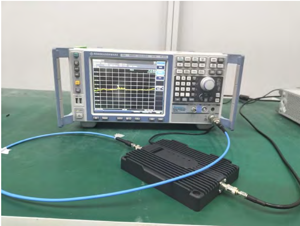
RF Conducted Test View
