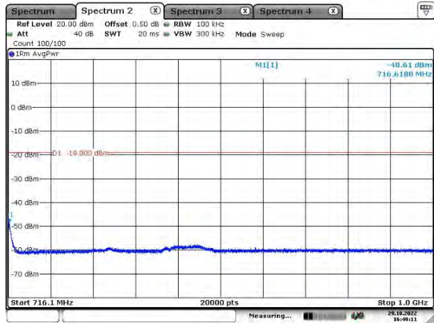
Lower 700 MHz Band-2
