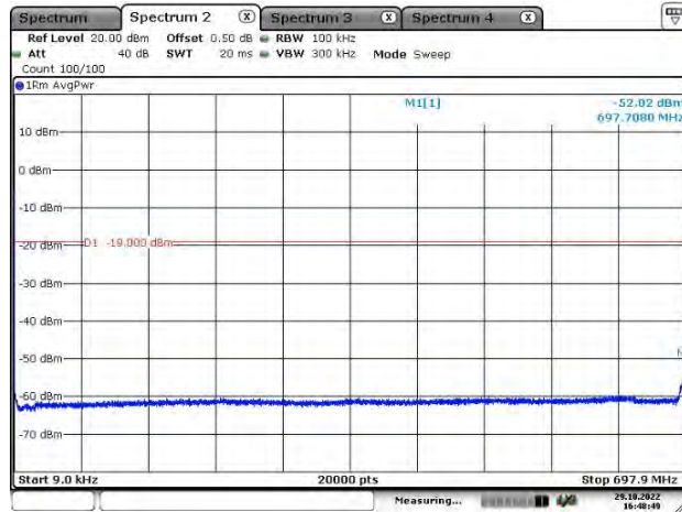
Lower 700 MHz Band-1
