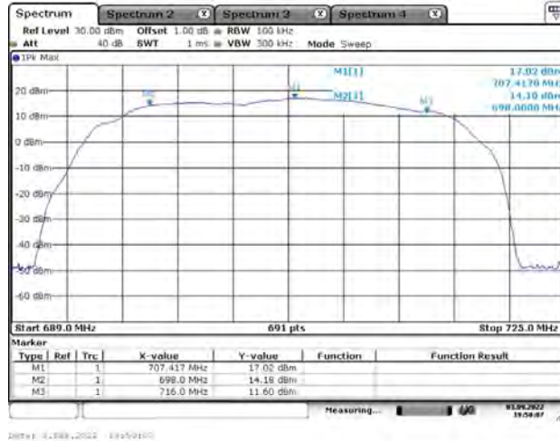
Cellular Band Uplink
