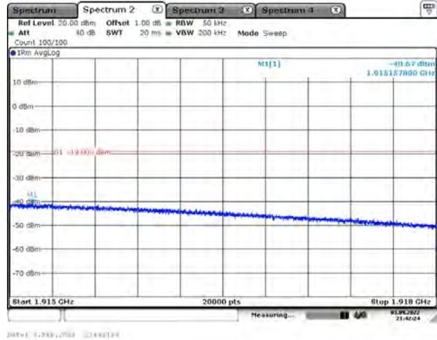
Right Side-WCDMA-Above AGC
