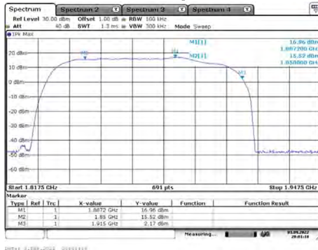
PCS Band Uplink
