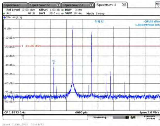
PCS Band Uplink-Pre AGC
