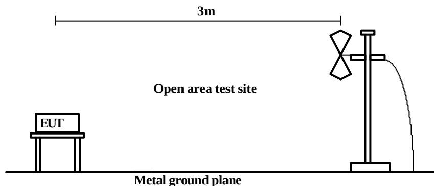
Figure 2. Radiated emission
