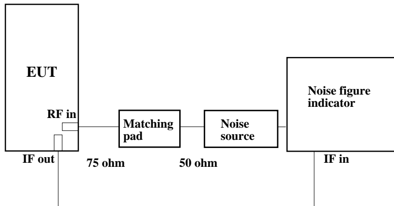
Figure 7. Noise figure
