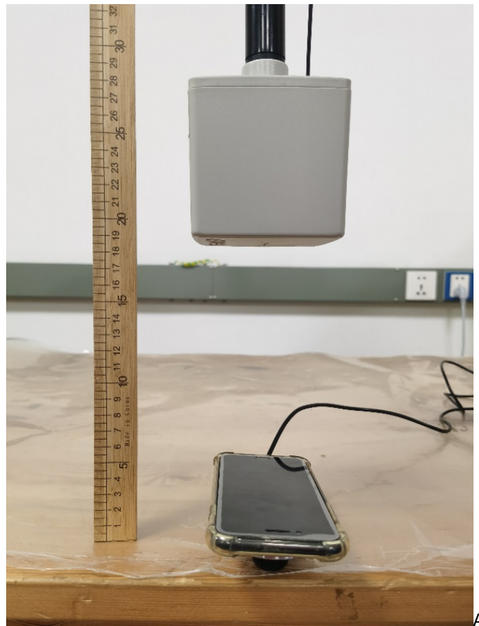
Photograph 3: Set-up photo for RF Exposure
