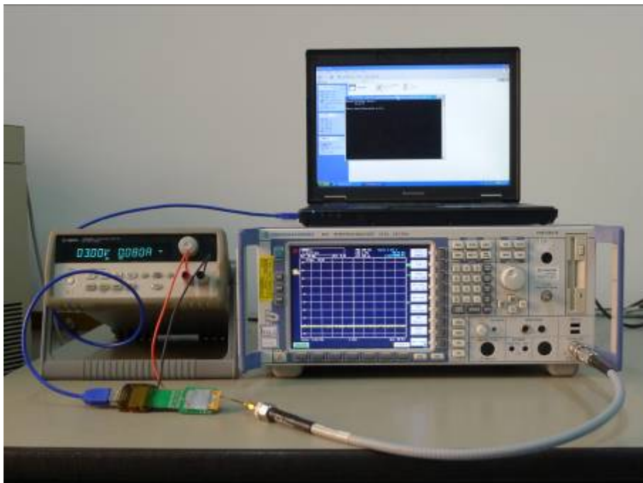
Conducted Spurious Emissions Test setup
