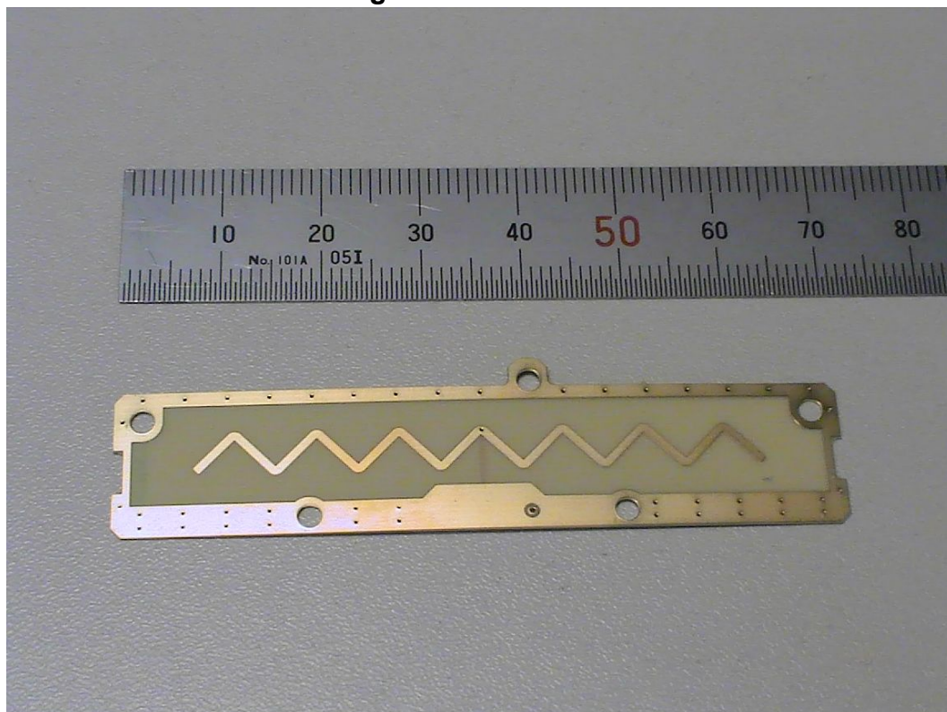
Fig.8 Antenna PCB2
