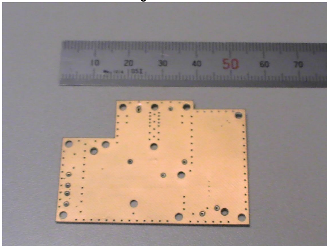
Fig.2 RF PCB2
