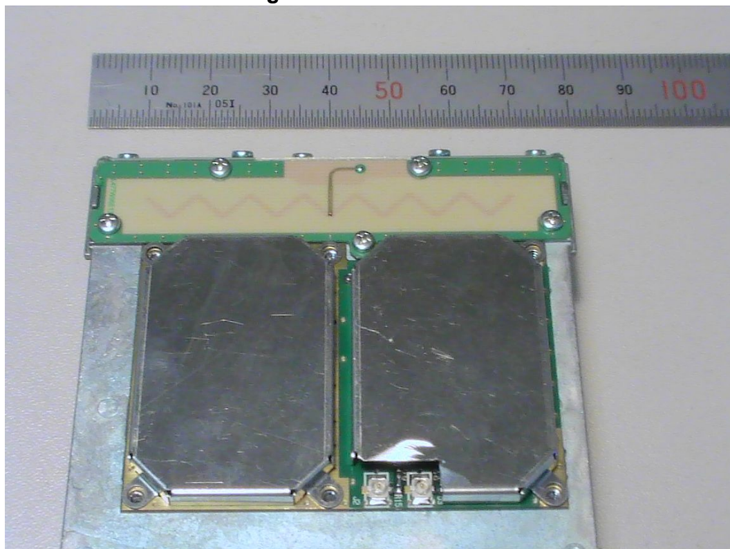
Fig.6 BaseBand Covers
