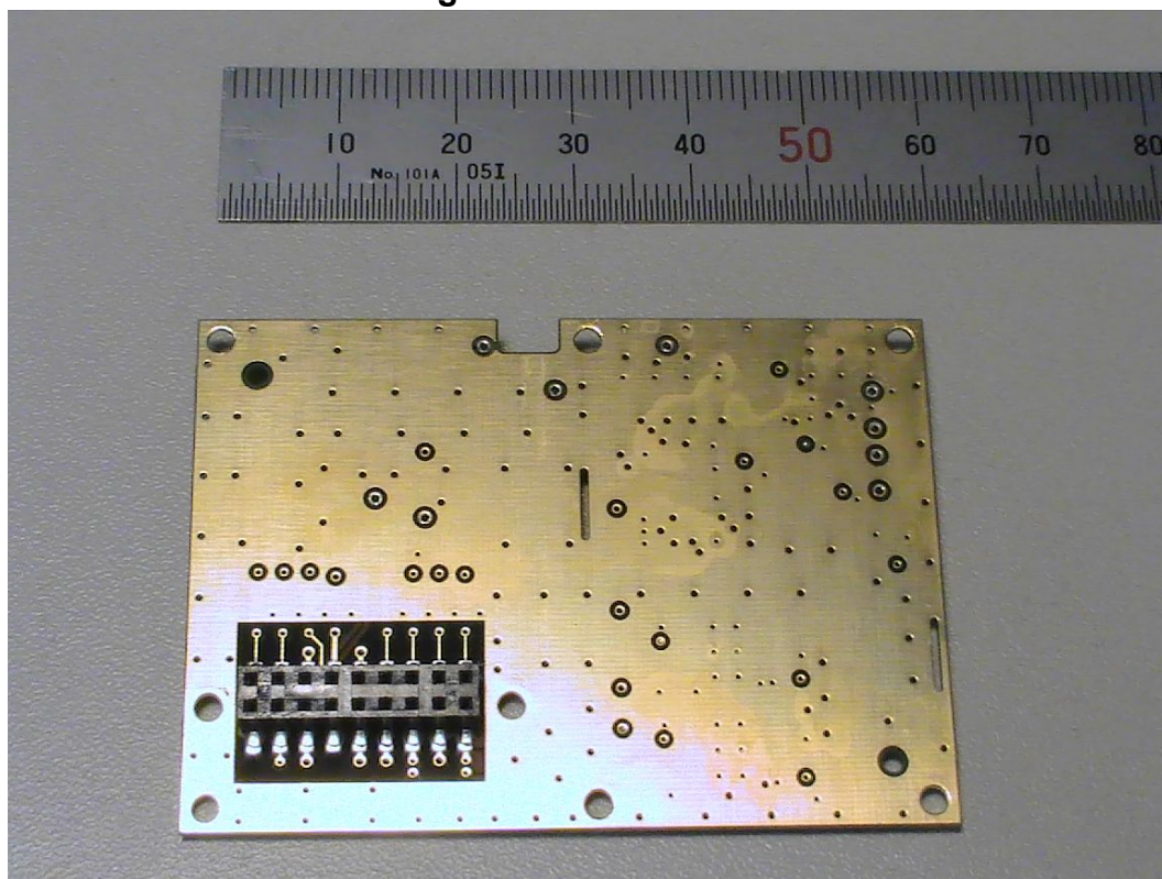
Fig.5 BaseBand PCB2
