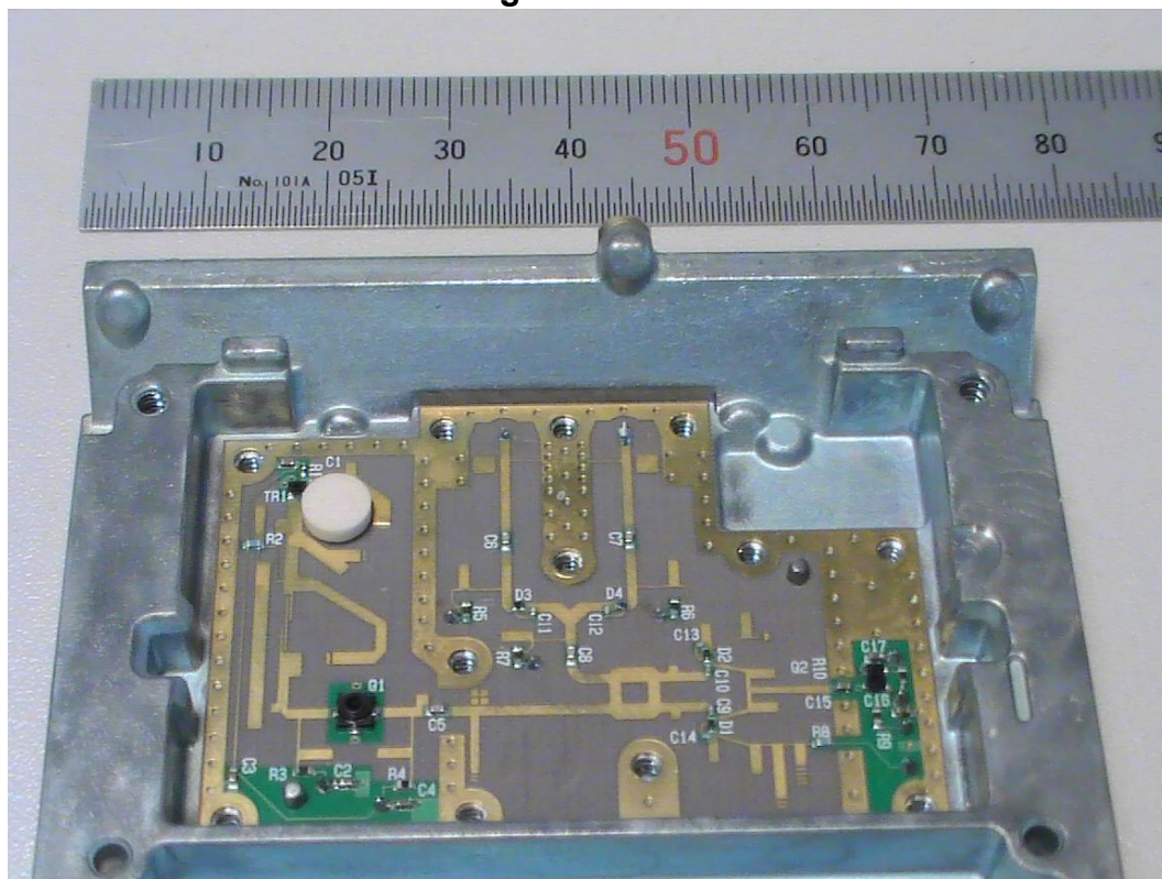
Fig.1 RF PCB1
