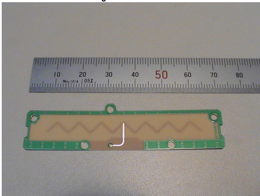
Fig.7 Antenna PCB1
