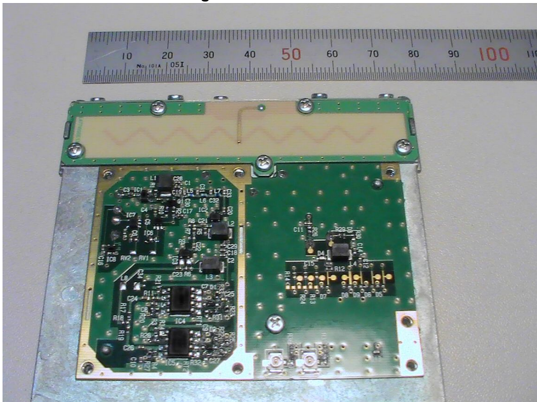
Fig.4 BaseBand PCB1
