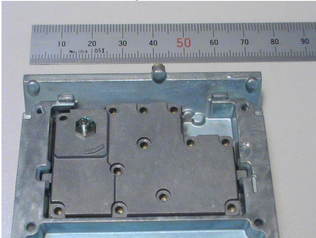
Fig.3 RF Cover
