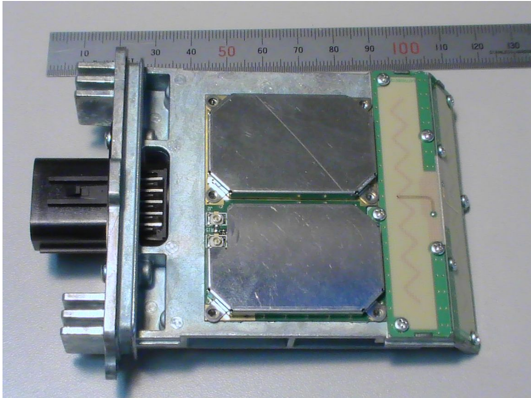
Fig.9 Positions of BaseBand and Antennas
