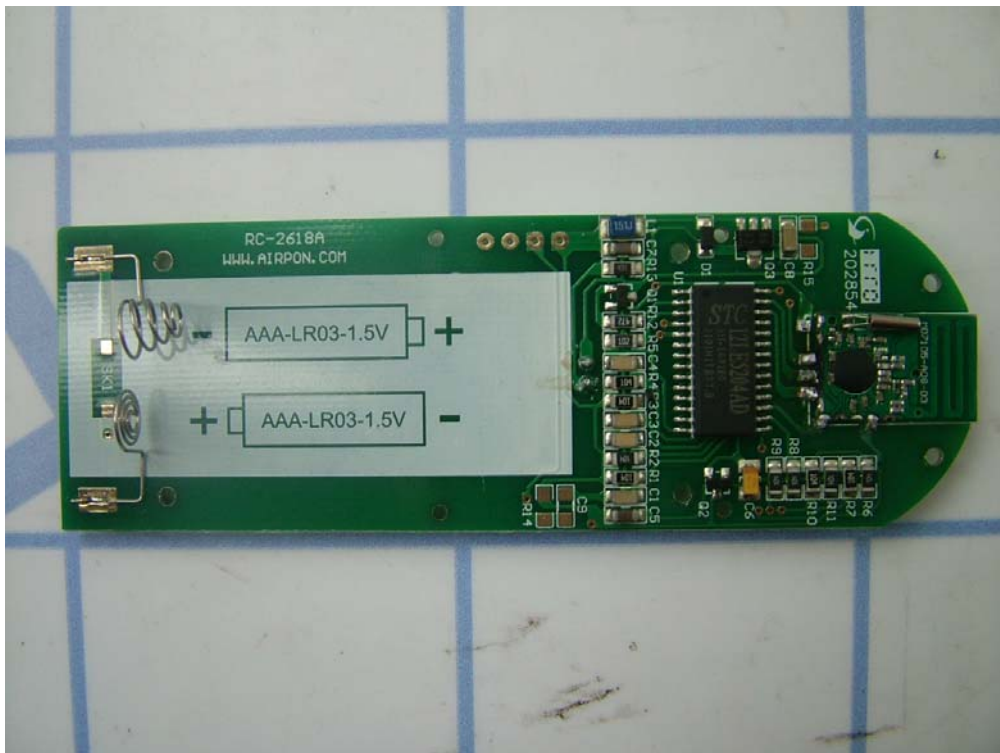
PCB layout-1
