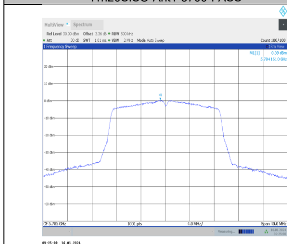
11n20SISO-Ant1-5785-PASS
