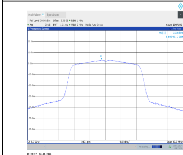
11n20SISO-Ant1-5700-PASS
