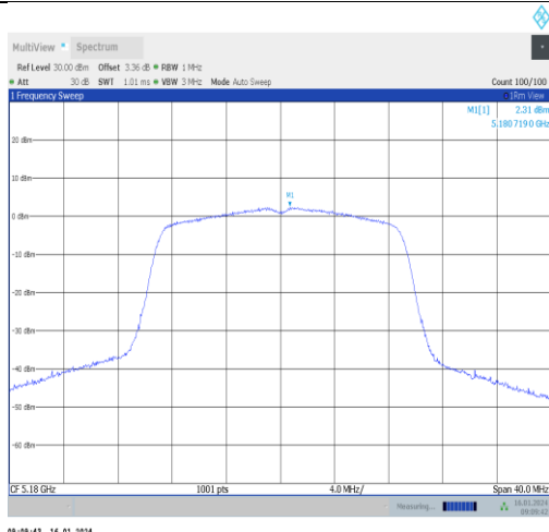
11n20ISO-Ant1-5180-PASS
