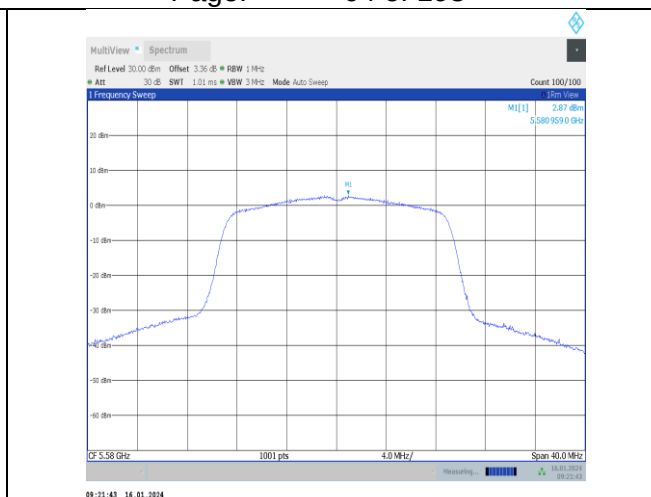
11n20SISO-Ant1-5580-PASS
