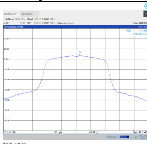
11a-Ant1-5580-PASS
