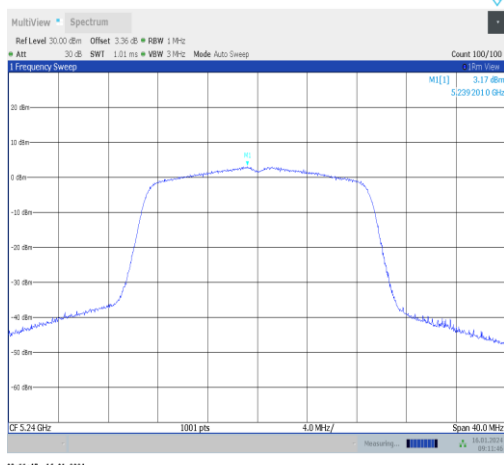
11n20ISO-Ant1-5240-PASS
