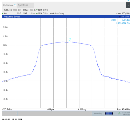
11a-Ant1-5700-PASS
