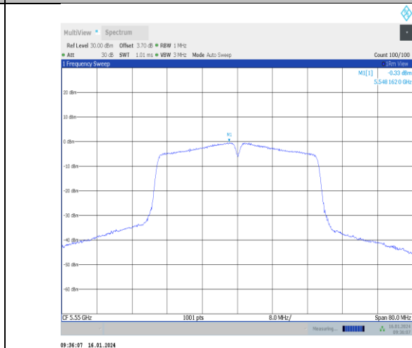
11n40SISO-Ant1-5550-PASS
