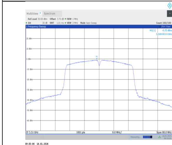
11n40SISO-Ant1-5510-PASS
