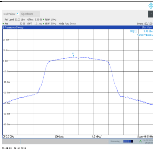
11a-Ant1-5500-PASS
