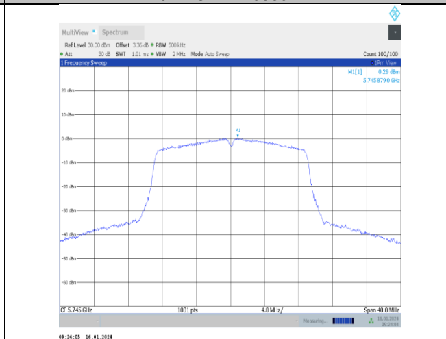
11n20SISO-Ant1-5745-PASS
