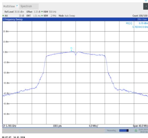
11a-Ant1-5785-PASS
