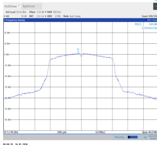
11a-Ant1-5745-PASS
