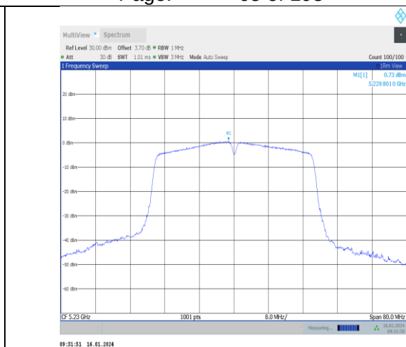
11n40SISO-Ant1-5230-PASS
