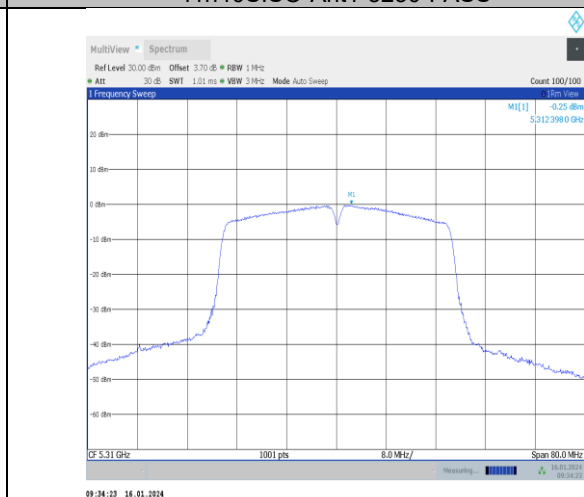
11n40SISO-Ant1-5310-PASS
