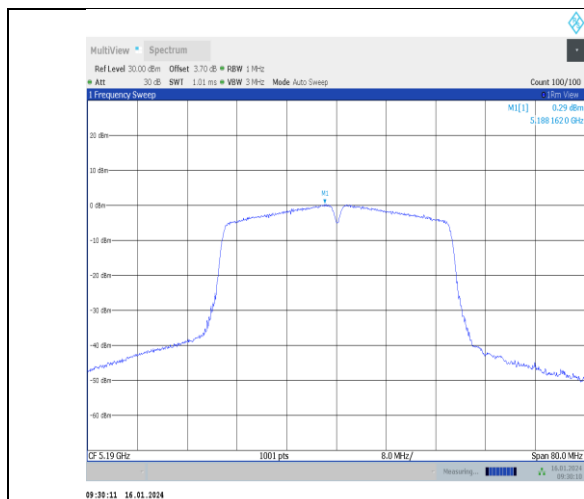
11n40SISO-Ant1-5190-PASS
