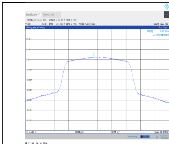
11n20SISO-Ant1-5500-PASS
