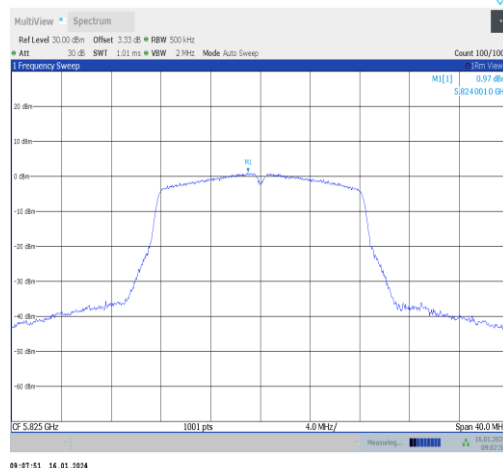
11a-Ant1-5825-PASS
