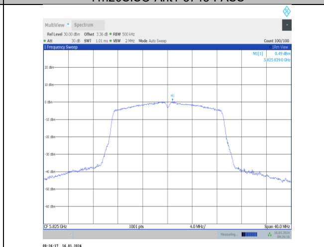
11n20SISO-Ant1-5825-PASS
