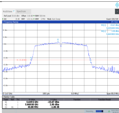
11n40SISO-Ant1-5670
