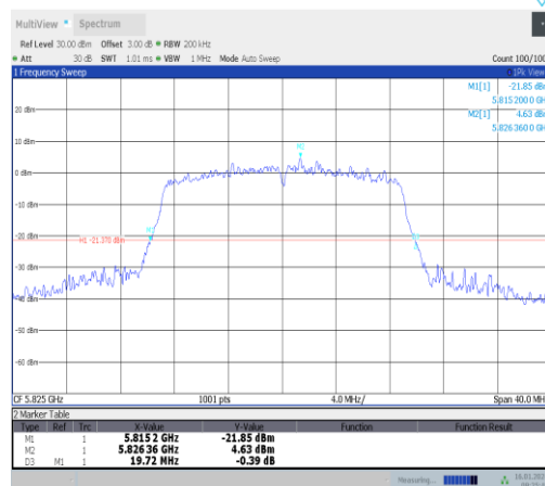
11n20SISO-Ant1-5825
