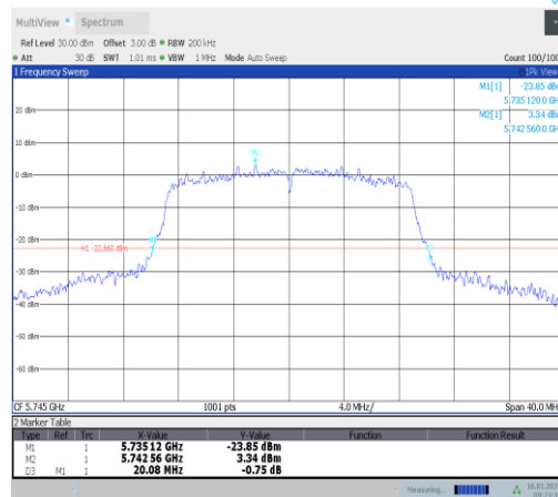
11n20SISO-Ant1-5745
