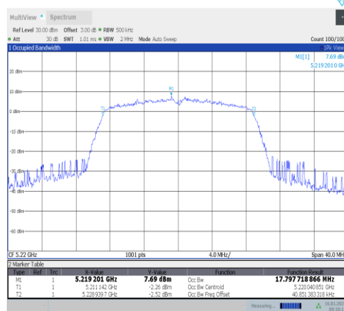
11n20SISO-Ant1-5220
