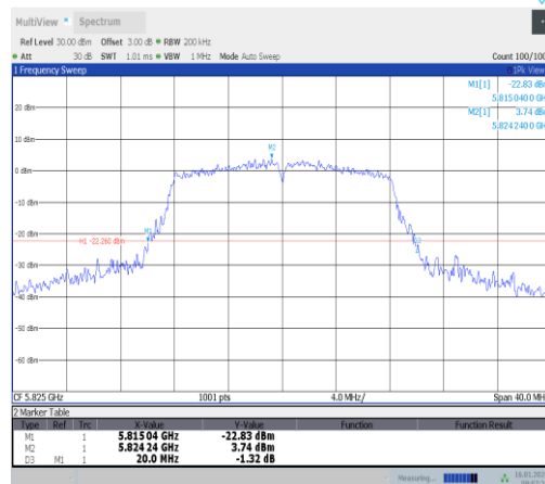
11a-Ant1-5825
