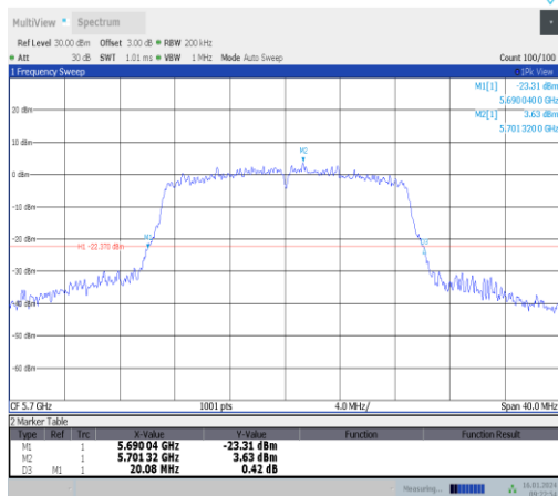
11n20SISO-Ant1-5700
