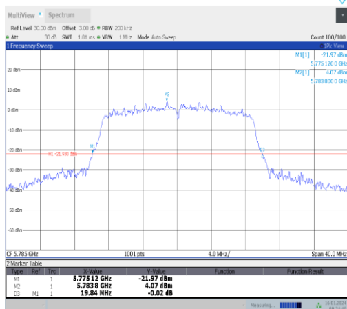
11n20SISO-Ant1-5785
