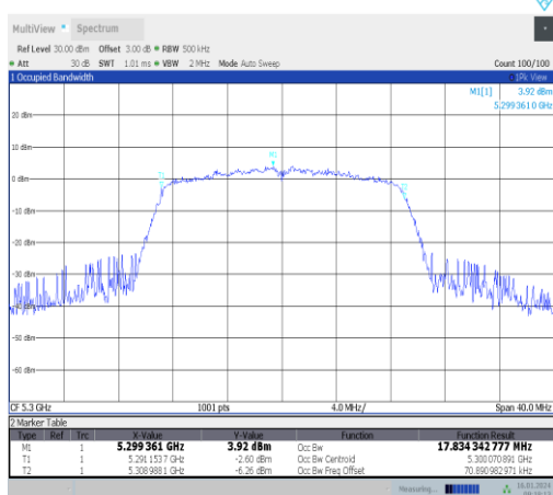
11n20SISO-Ant1-5300
