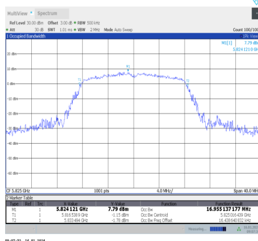
11a-Ant1-5825
