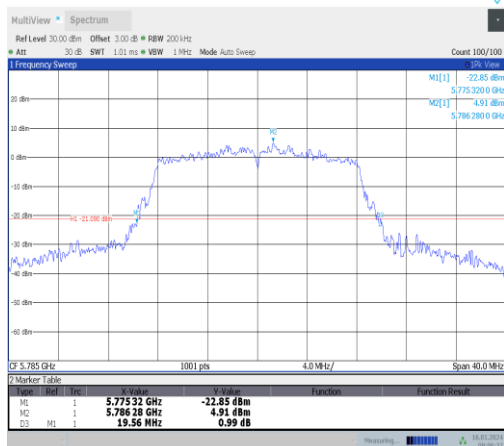
11a-Ant1-5785
