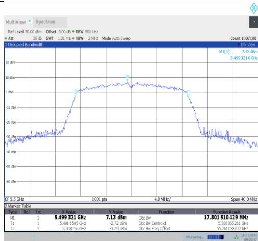
11n20SISO-Ant1-5500
