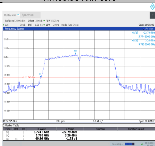
11n40SISO-Ant1-5795
