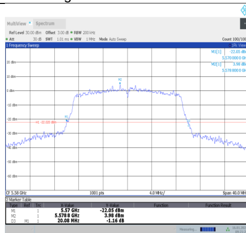
11n20SISO-Ant1-5580
