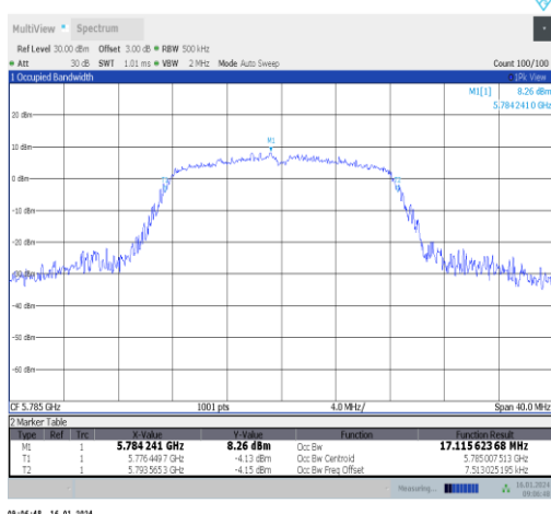
11a-Ant1-5785
