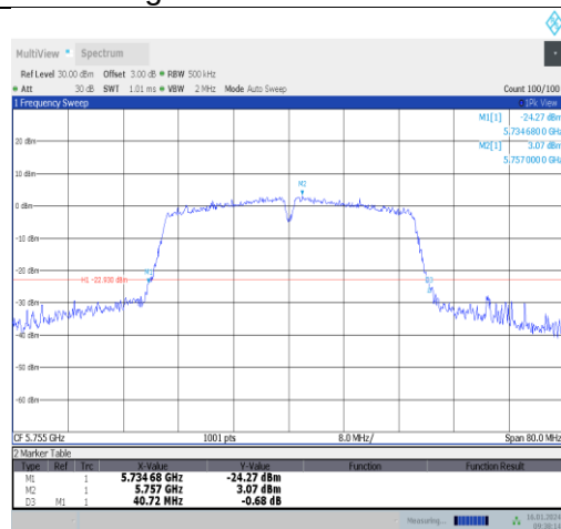
11n40SISO-Ant1-5755
