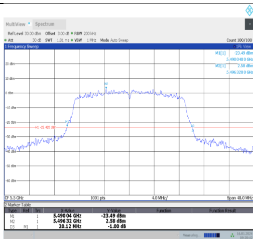
11n20SISO-Ant1-5500
