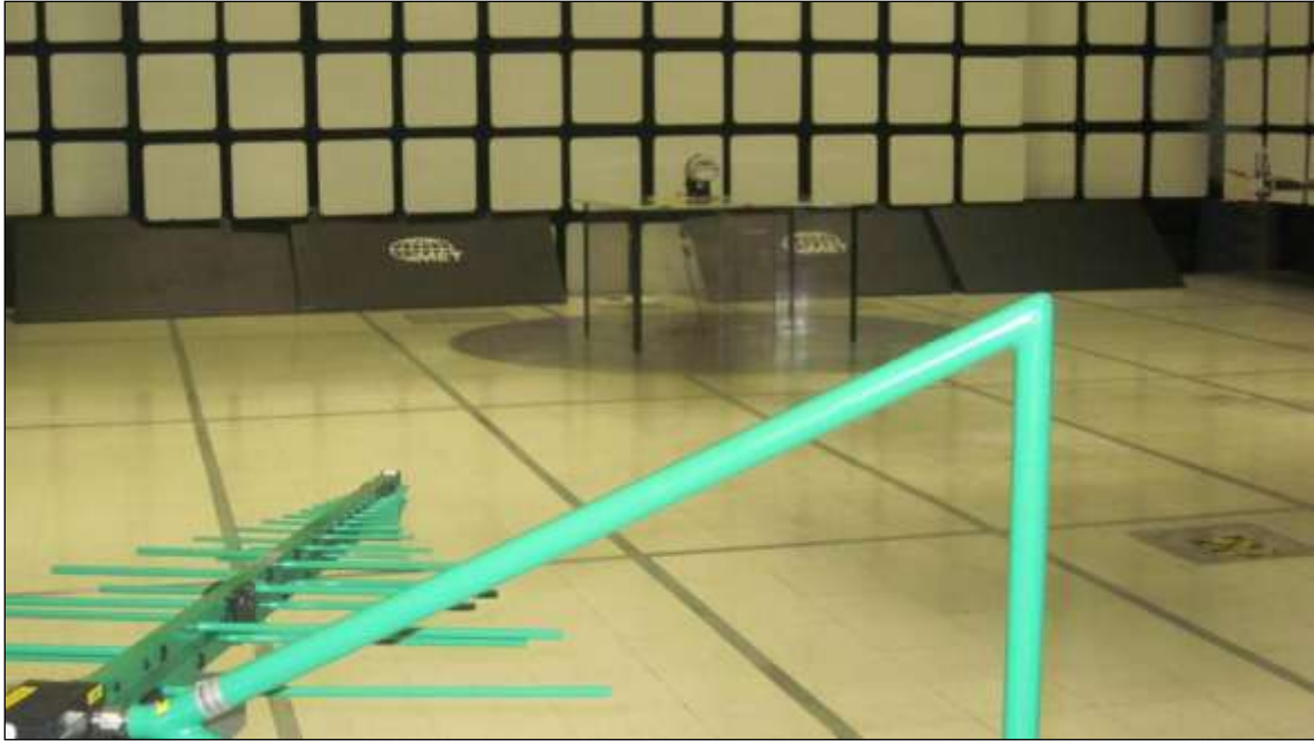
Photograph 3. Radiated Emissions, Test Setup, 30 MHz – 1 GHz
