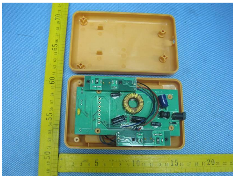
EUT2-Open View
