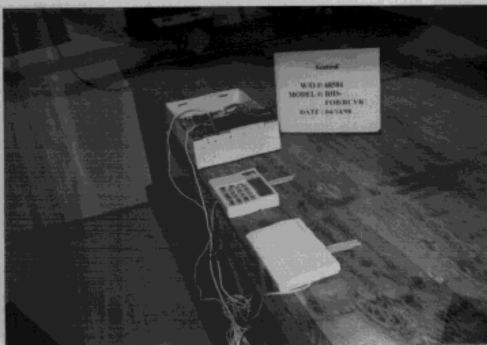
Conducted Emissions - Back View
