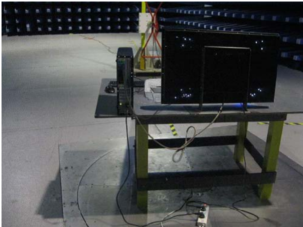
Radiated Emission (30MHz – 1GHz) - Rear View
