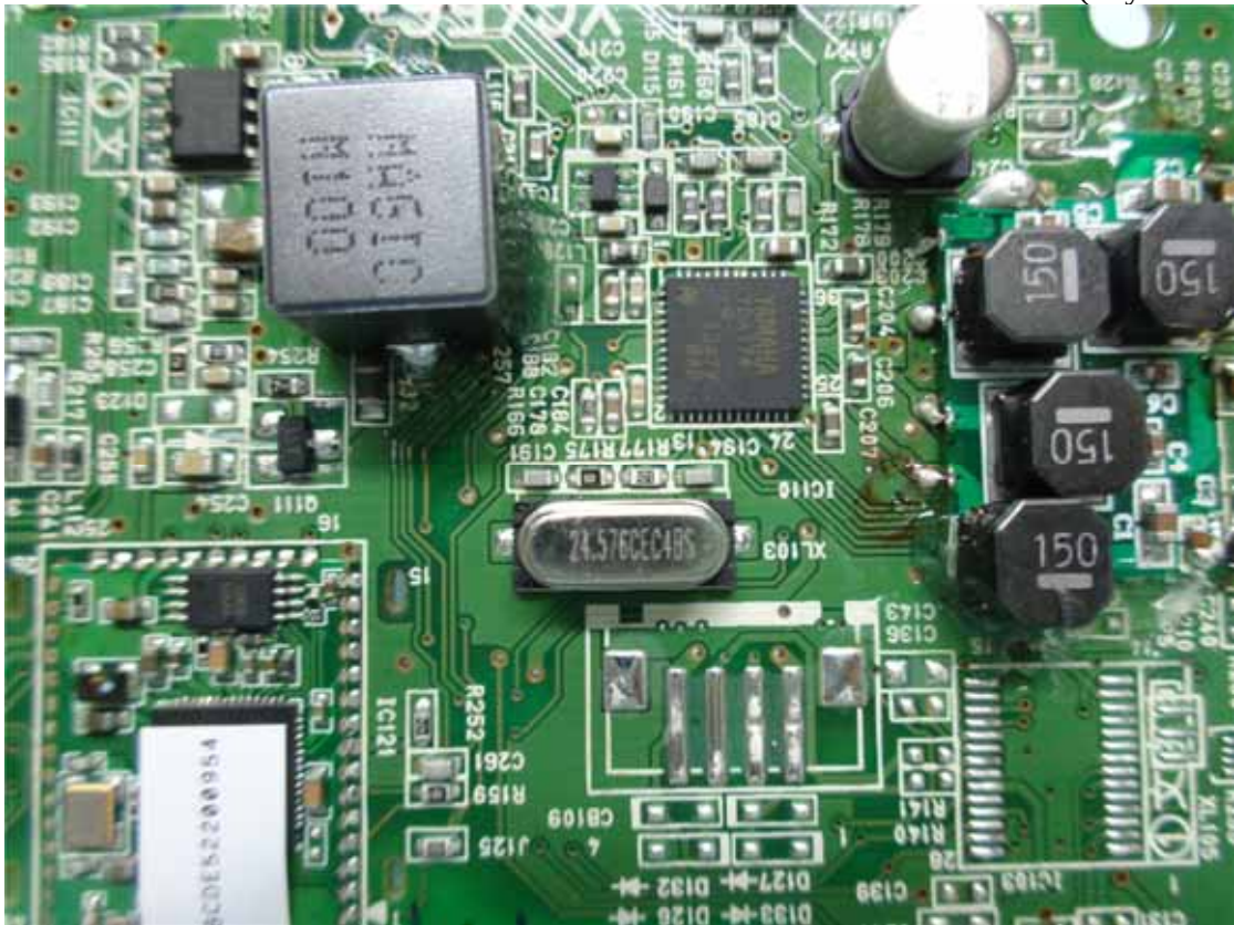
Figure 5 Main Board (Crystal Oscillator)
