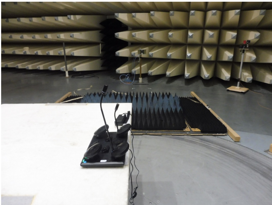
Photo 2: Radiated Emission
