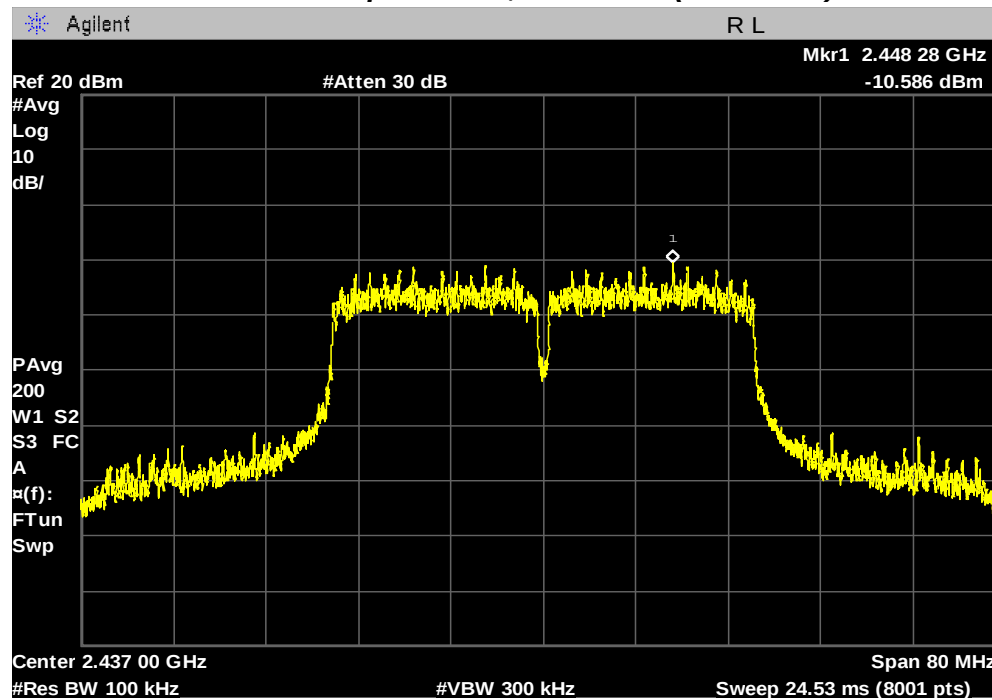
Maximum Conducted Output Power, 6 Channel (2 437 MHz)
