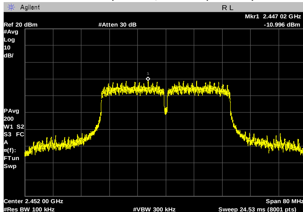
Maximum Conducted Output Power, 9 Channel (2 452 MHz)
