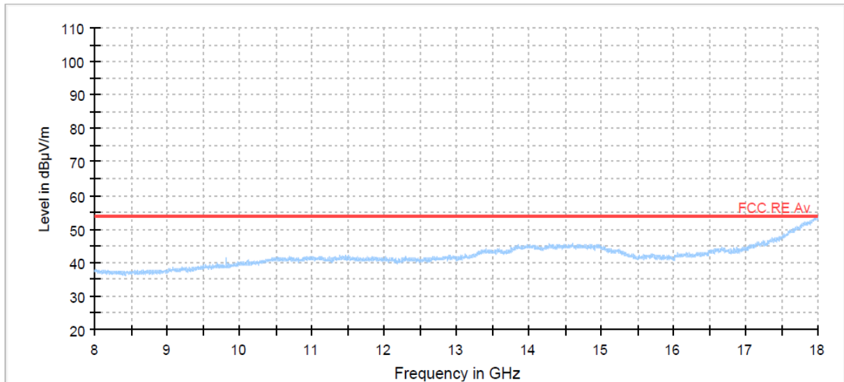
9 channel : 8 GHz to 18 GHz_Average
