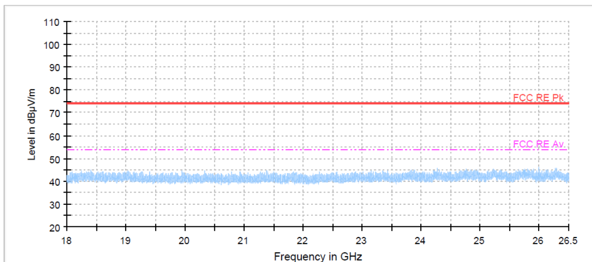
9 channel : 18 GHz to 26.5 GHz_Peak
