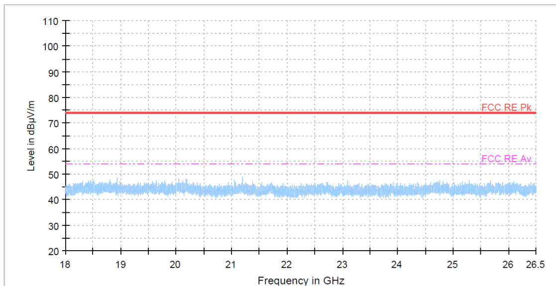
Middle channel : 18 GHz to 26.5 GHz_Peak
