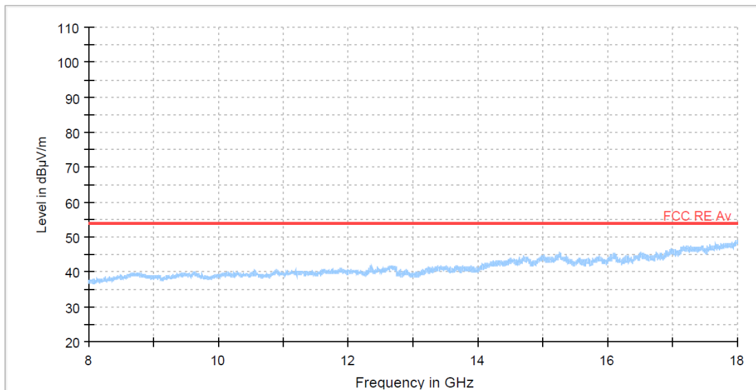
Middle channel : 8 GHz to 18 GHz_Average
