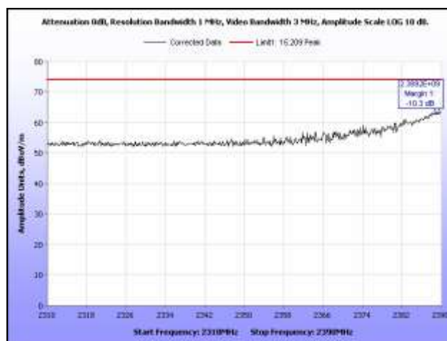
Plot 44. Restricted Band, Low Channel, Peak
