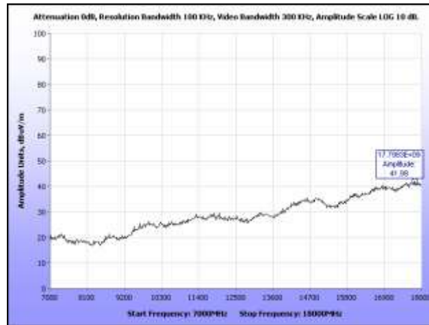
Plot 37. Radiated Harmonics, Mid Channel, 7 GHz – 18 GHz
