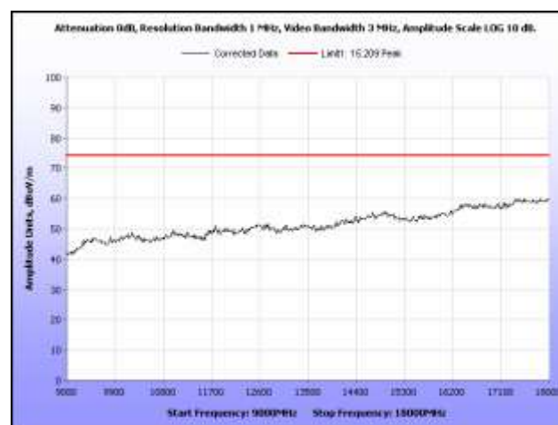
Plot 21. Radiated Spurious Emissions, Mid Channel, 9 GHz – 18 GHz, Peak
