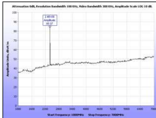
Plot 32. Radiated Harmonics, Low Channel, 1 GHz – 7 GHz
