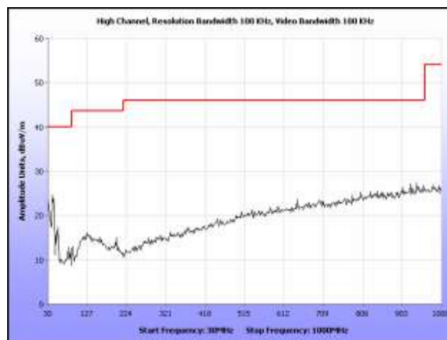
Plot 39. Radiated Harmonics, High Channel, 30 MHz – 1 GHz
