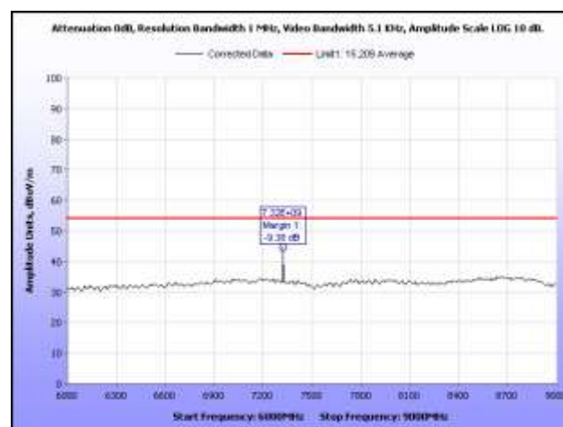
Plot 18. Radiated Spurious Emissions, Mid Channel, 6 GHz – 9 GHz, Average
