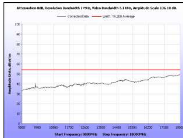
Plot 20. Radiated Spurious Emissions, Mid Channel, 9 GHz – 18 GHz, Average
