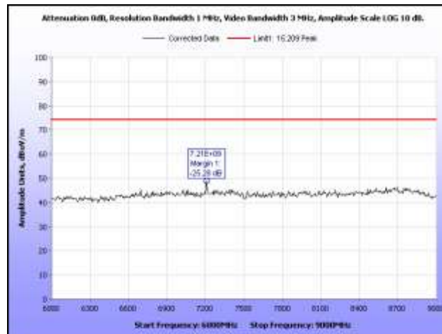
Plot 11. Radiated Spurious Emissions, Low Channel, 6 GHz – 9 GHz, Peak
