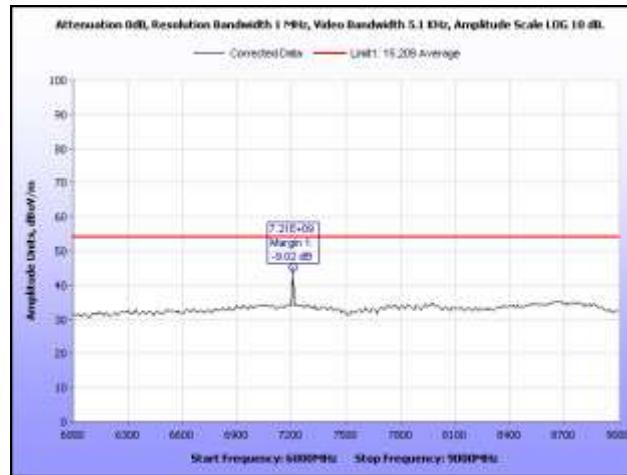
Plot 10. Radiated Spurious Emissions, Low Channel, 6 GHz – 9 GHz, Average
