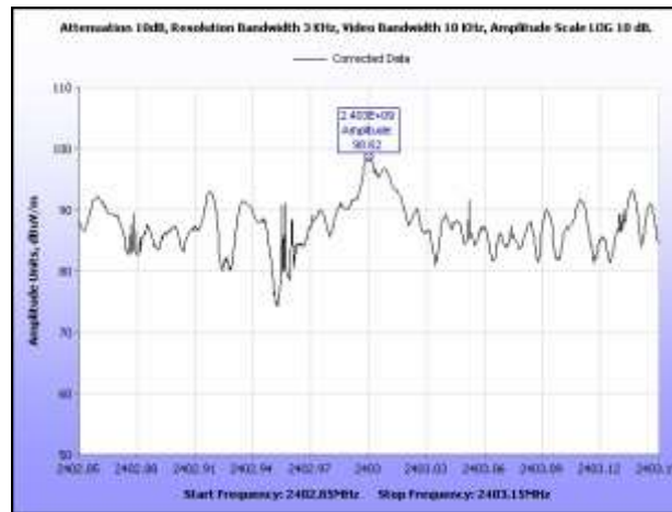
Plot 47. Peak Power Spectral Density, Low Channel @ 1 m
