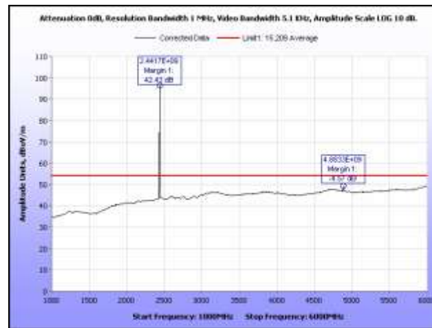
Plot 16. Radiated Spurious Emissions, Mid Channel, 1 GHz – 6 GHz, Average
