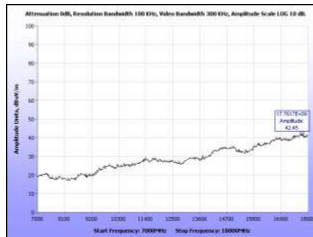
Plot 41. Radiated Harmonics, High Channel, 7 GHz – 18 GHz
