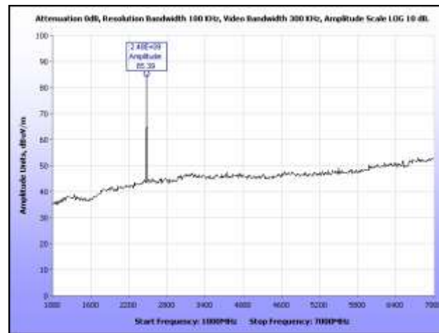
Plot 40. Radiated Harmonics, High Channel, 1 GHz – 7 GHz
