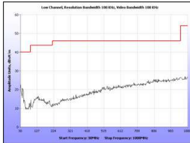
Plot 31. Radiated Harmonics, Low Channel, 30 MHz – 1 GHz
