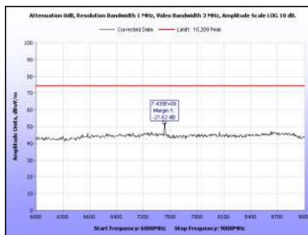
Plot 27. Radiated Spurious Emissions, High Channel, 6 GHz – 9 GHz, Peak
