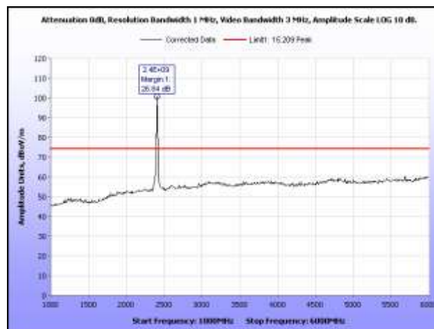
Plot 9. Radiated Spurious Emissions, Low Channel, 1 GHz – 6 GHz, Peak
