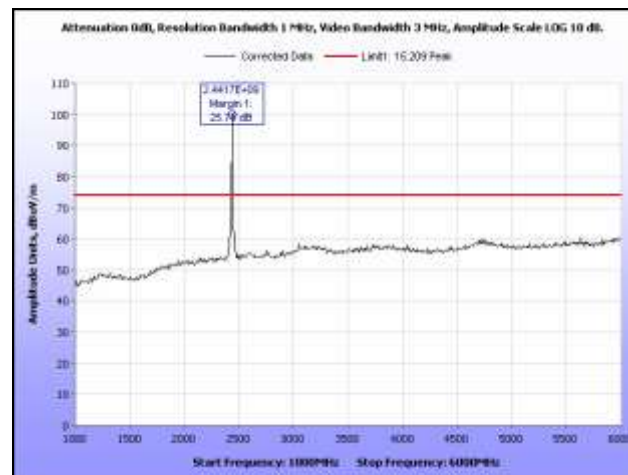
Plot 17. Radiated Spurious Emissions, Mid Channel, 1 GHz – 6 GHz, Peak
