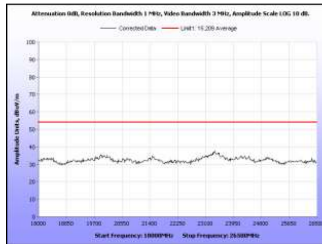
Plot 22. Radiated Spurious Emissions, Mid Channel, 18 GHz – 26.5 GHz, Peak under Average
