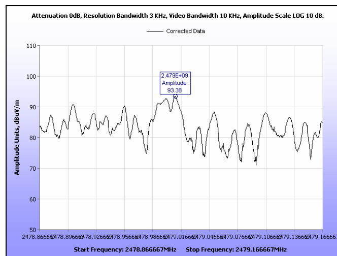
Plot 49. Peak Power Spectral Density, High Channel @ 1 m
