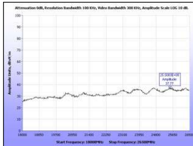
Plot 38. Radiated Harmonics, Mid Channel, 18 GHz – 26.5 GHz
