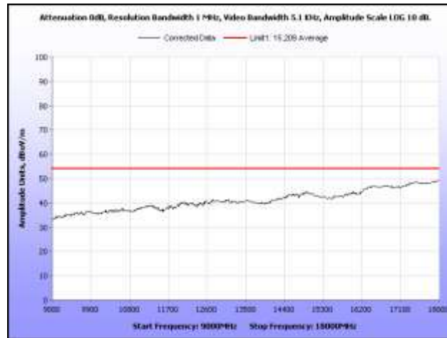
Plot 28. Radiated Spurious Emissions, High Channel, 9 GHz – 18 GHz, Average
