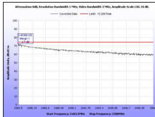
Plot 46. Restricted Band, High Channel, Peak
