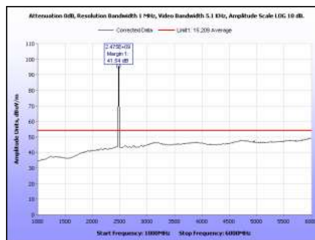
Plot 24. Radiated Spurious Emissions, High Channel, 1 GHz – 6 GHz, Average
