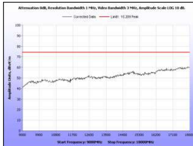
Plot 29. Radiated Spurious Emissions, High Channel, 9 GHz – 18 GHz, Peak
