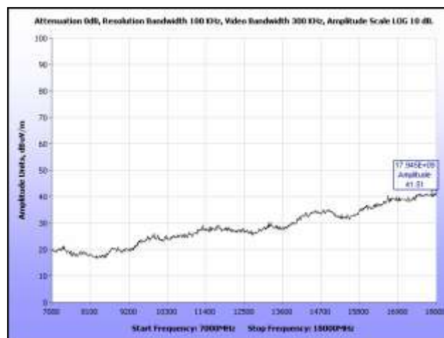
Plot 33. Radiated Harmonics, Low Channel, 7 GHz – 18 GHz
