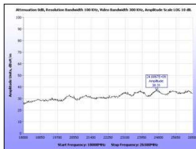
Plot 42. Radiated Harmonics, High Channel, 18 GHz – 26.5 GHz
