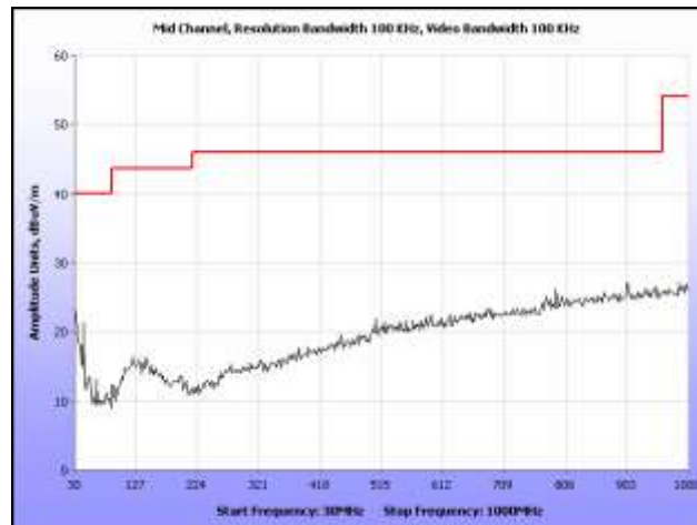
Plot 35. Radiated Harmonics, Mid Channel, 30 MHz – 1 GHz
