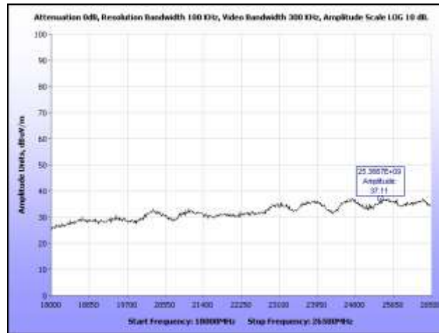
Plot 34. Radiated Harmonics, Low Channel, 18 GHz – 26.5 GHz
