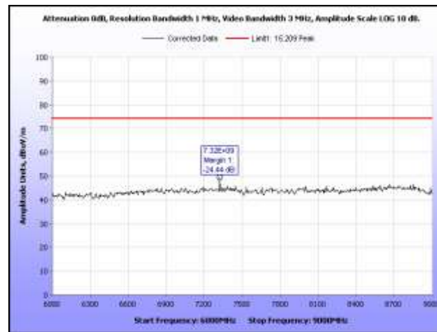
Plot 19. Radiated Spurious Emissions, Mid Channel, 6 GHz – 9 GHz, Peak
