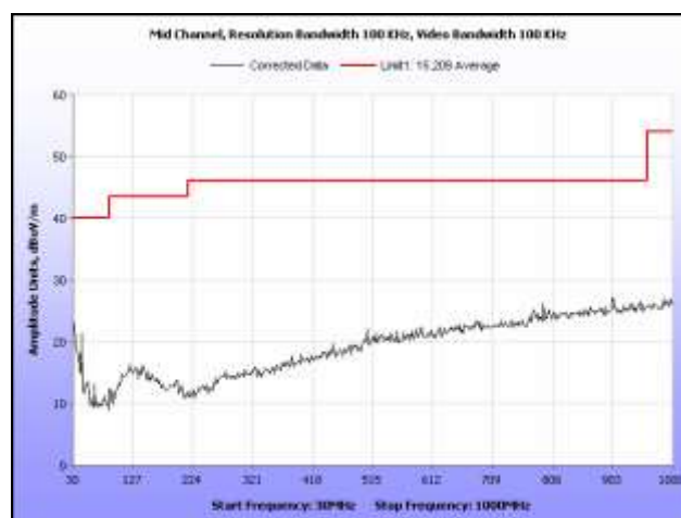
Plot 15. Radiated Spurious Emissions, Mid Channel, 30 MHz – 1 GHz
