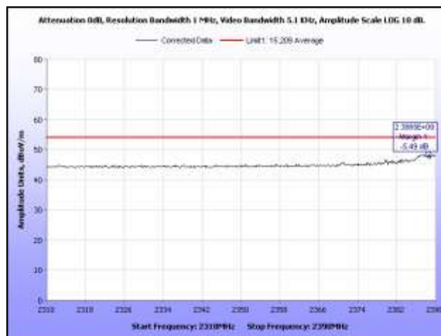
Plot 43. Restricted Band, Low Channel, Average
