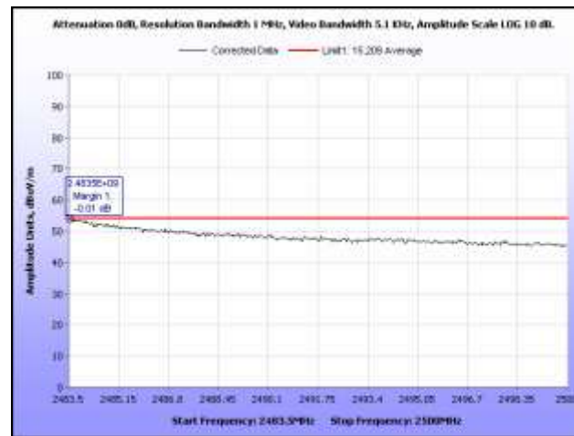
Plot 45. Restricted Band, High Channel, Average
