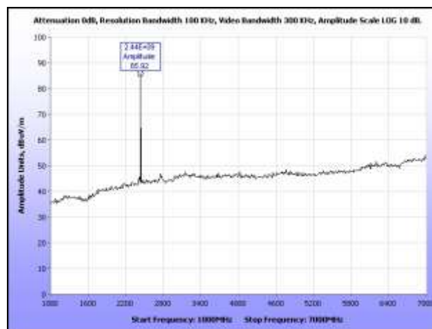
Plot 36. Radiated Harmonics, Mid Channel, 1 GHz – 7 GHz
