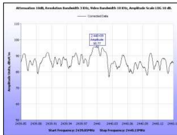
Plot 48. Peak Power Spectral Density, Mid Channel @ 1 m
