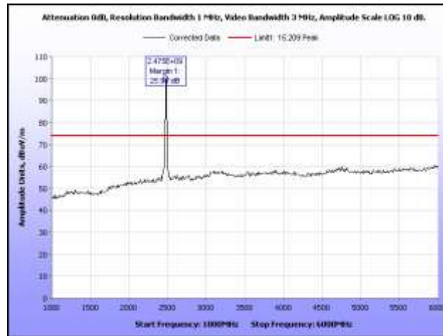
Plot 25. Radiated Spurious Emissions, High Channel, 1 GHz – 6 GHz, Peak
