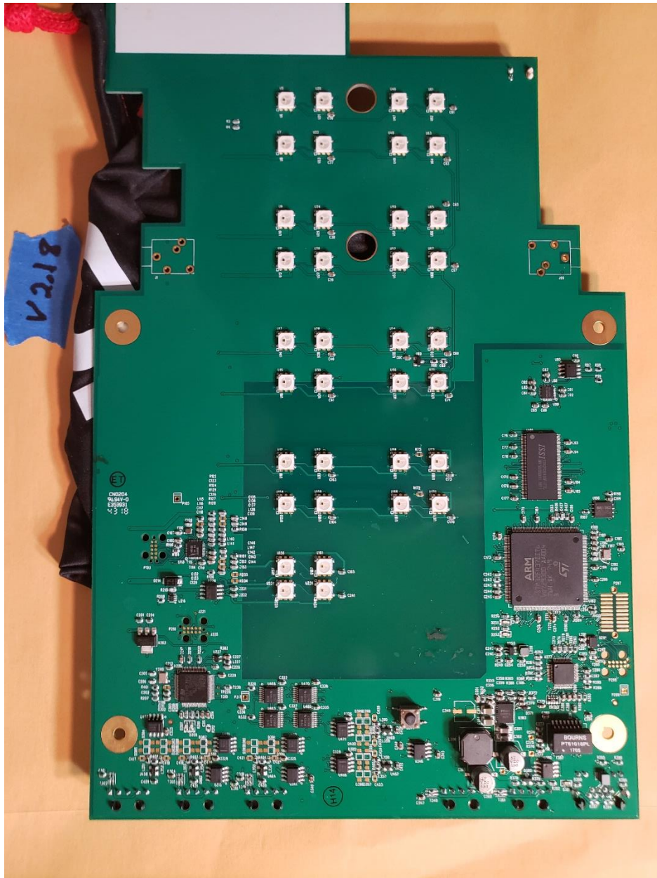
Main Control Board Detail Component Side
