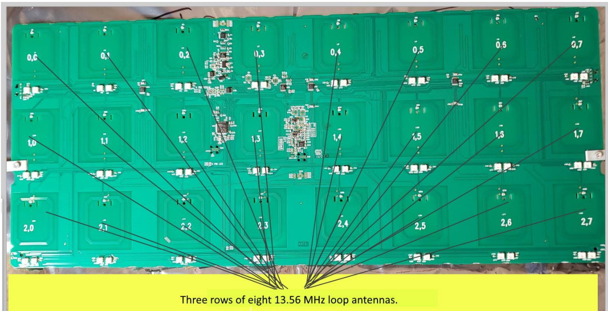
Antenna Board with 24 13.56 MHz Antennas.
