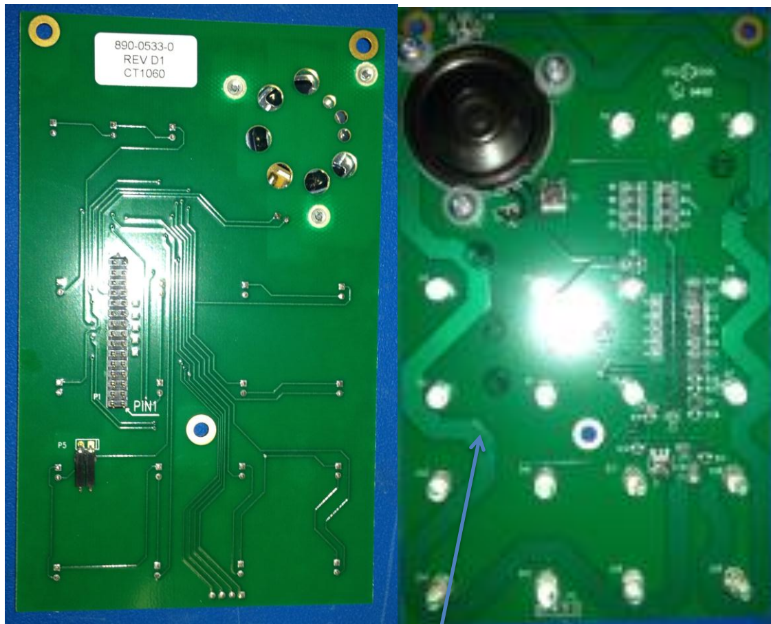
Loop Antenna
