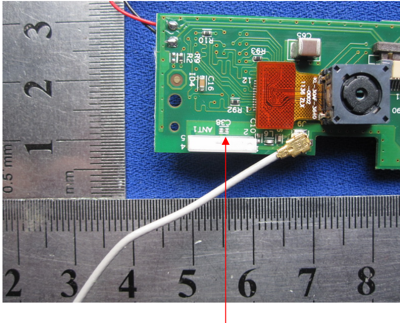
Wifi and BT Antenna
