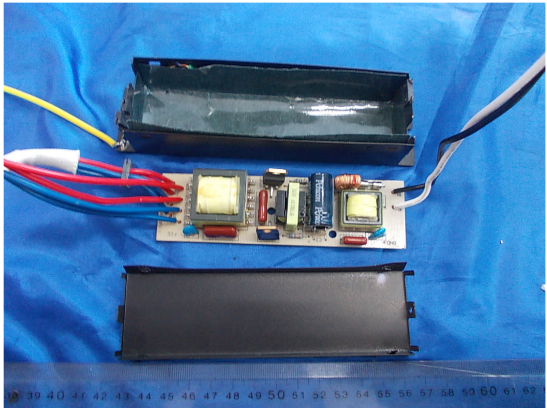
FIGURE 1 FLUORESCENT LAMP BALLAST (M/N: BEB/120/40+32/1) COVER REMOVED
