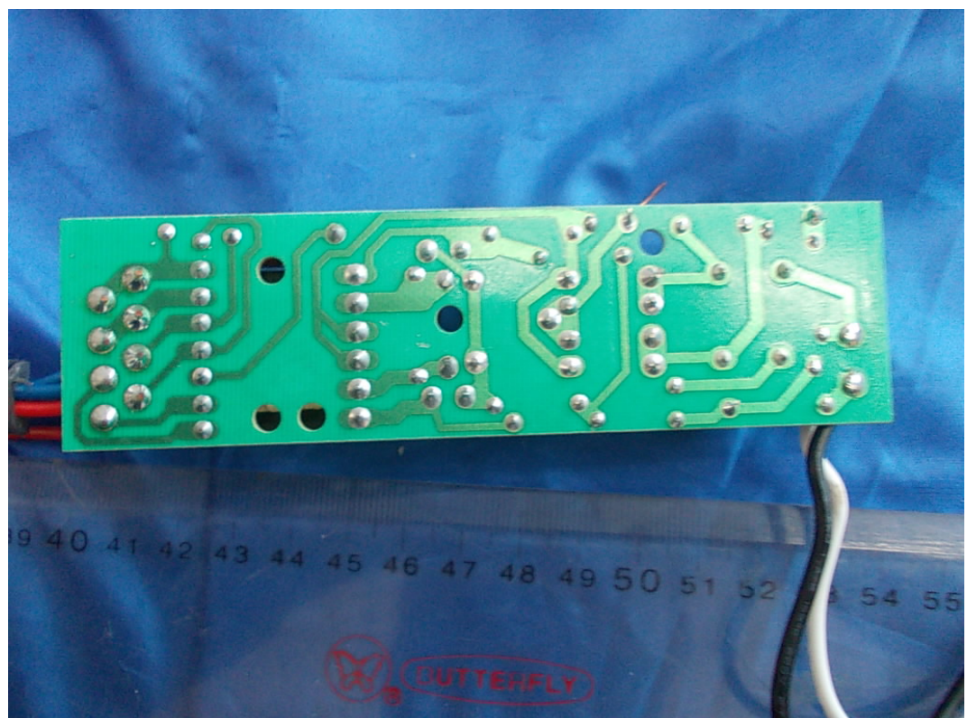
FIGURE 6 FLUORESCENT LAMP BALLAST (M/N: BEB/120/32+22/1) MAIN BOARD (SOLDERED SIDE)
