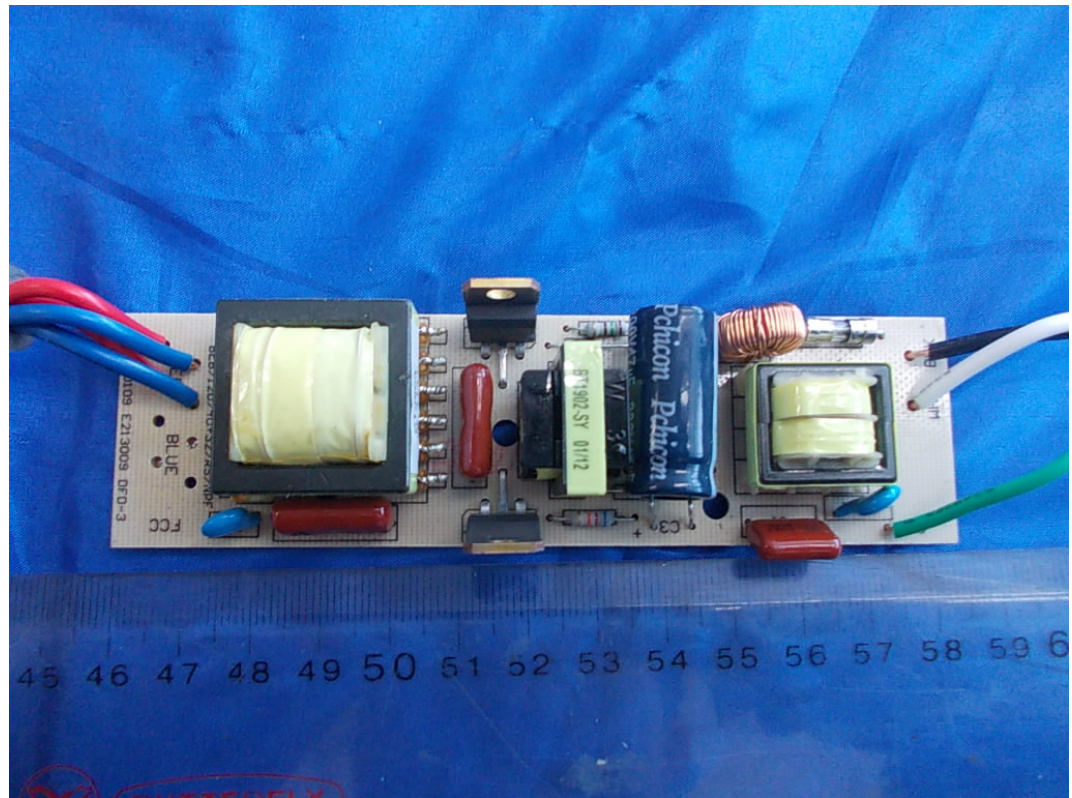
FIGURE 8 FLUORESCENT LAMP BALLAST (M/N: BEB/120/22) MAIN BOARD (COMPONENT SIDE)
