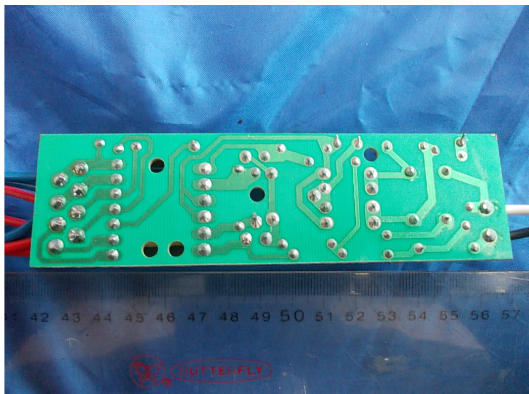
FIGURE 3 FLUORESCENT LAMP BALLAST (M/N: BEB/120/40+32/1) MAIN BOARD (SOLDERED SIDE)
