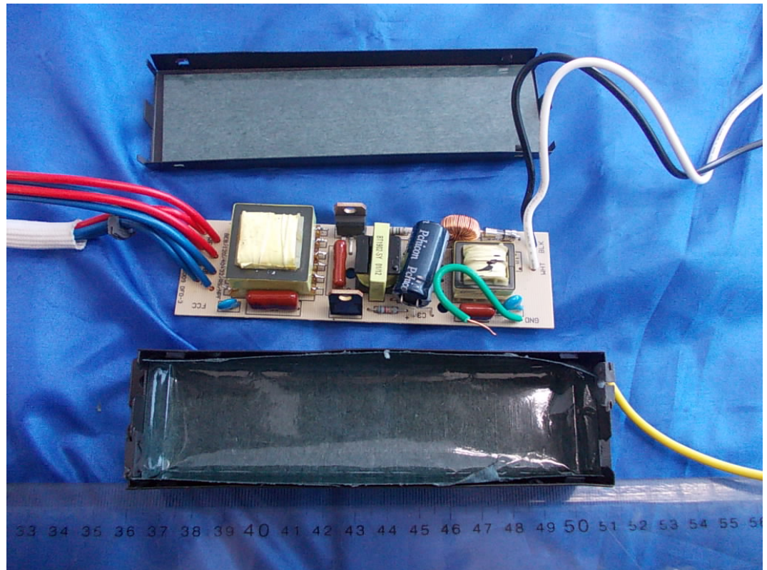
FIGURE 4 FLUORESCENT LAMP BALLAST (M/N: BEB/120/32+22/1) COVER REMOVED
