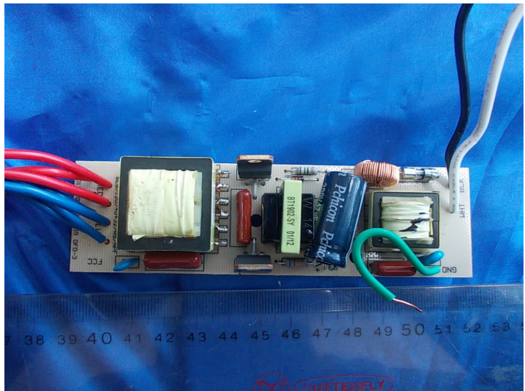
FIGURE 5 FLUORESCENT LAMP BALLAST (M/N: BEB/120/32+22/1) MAIN BOARD (COMPONENT SIDE)
