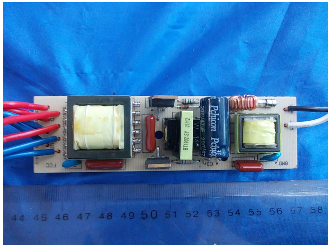
FIGURE 2 FLUORESCENT LAMP BALLAST (M/N: BEB/120/40+32/1) MAIN BOARD (COMPONENT SIDE)
