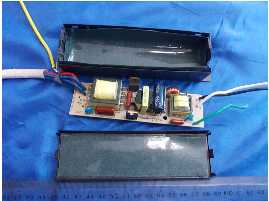
FIGURE 7 FLUORESCENT LAMP BALLAST (M/N: BEB/120/22) COVER REMOVED
