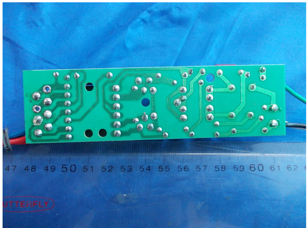
FIGURE 9 FLUORESCENT LAMP BALLAST (M/N: BEB/120/22) MAIN BOARD (SOLDERED SIDE)
