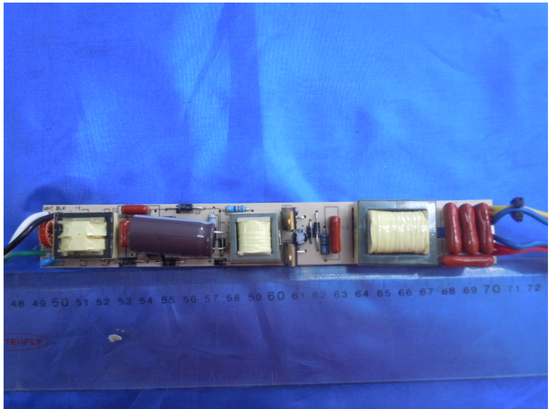
FIGURE 2 FLUORESCENT LAMP BALLAST (M/N: BEB/120/432) MAIN BOARD (COMPONENT SIDE)
