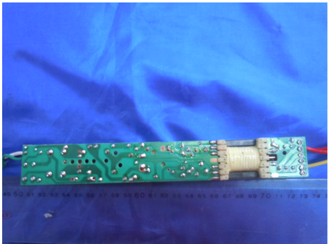
FIGURE 3 FLUORESCENT LAMP BALLAST (M/N: BEB/120/432) MAIN BOARD (SOLDERED SIDE)
