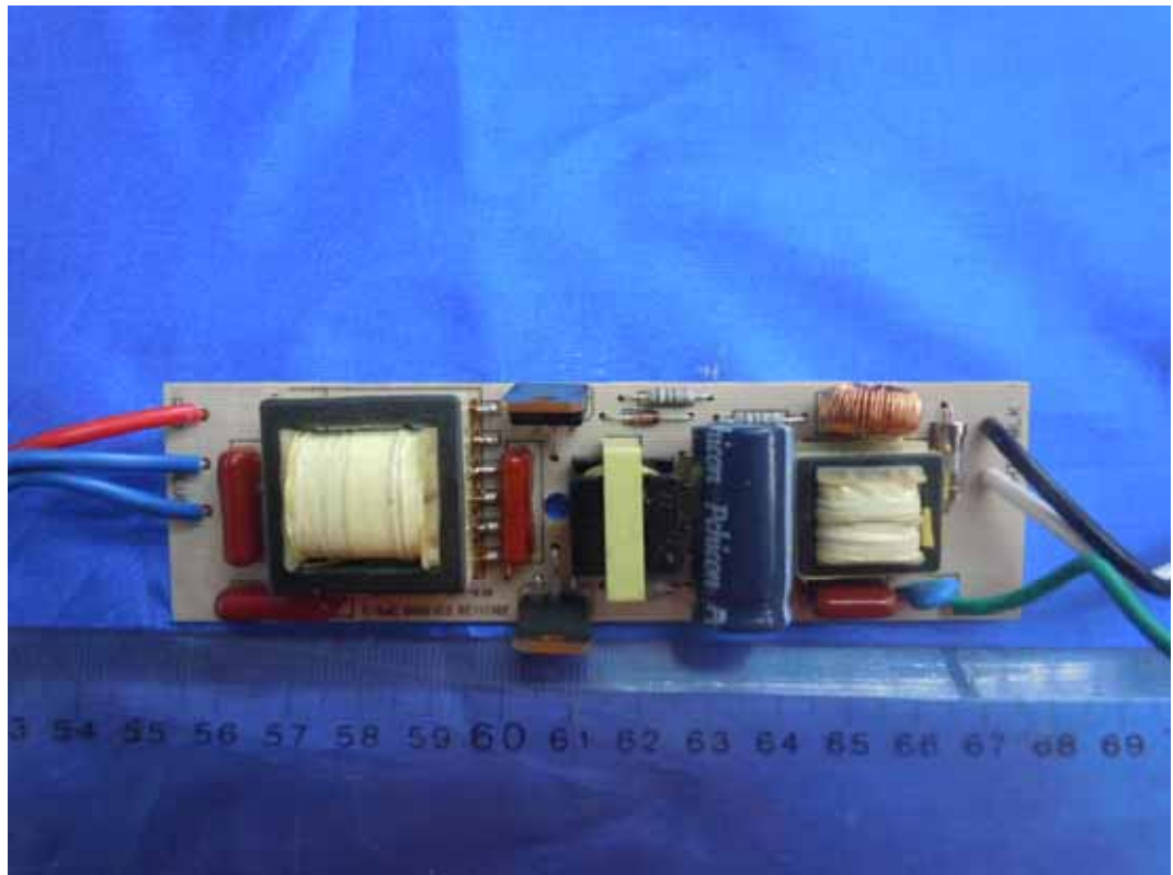
FIGURE 2 FLUORESCENT LAMP BALLAST (M/N: BEB/120/232) MAIN BOARD (COMPONENT SIDE)
