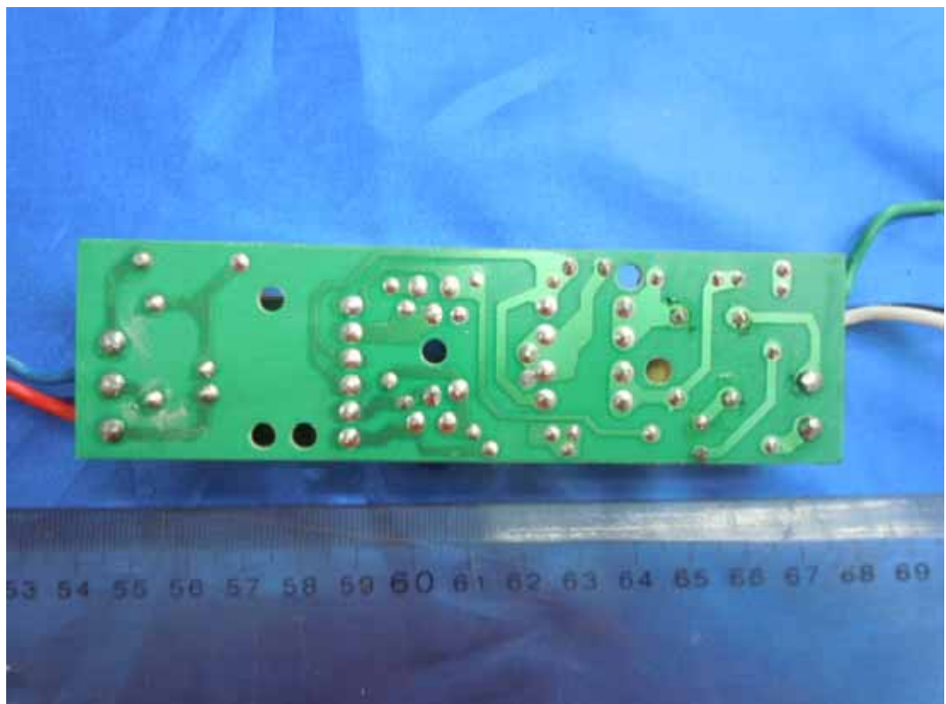
FIGURE 3 FLUORESCENT LAMP BALLAST (M/N: BEB/120/232) MAIN BOARD (SOLDERED SIDE)
