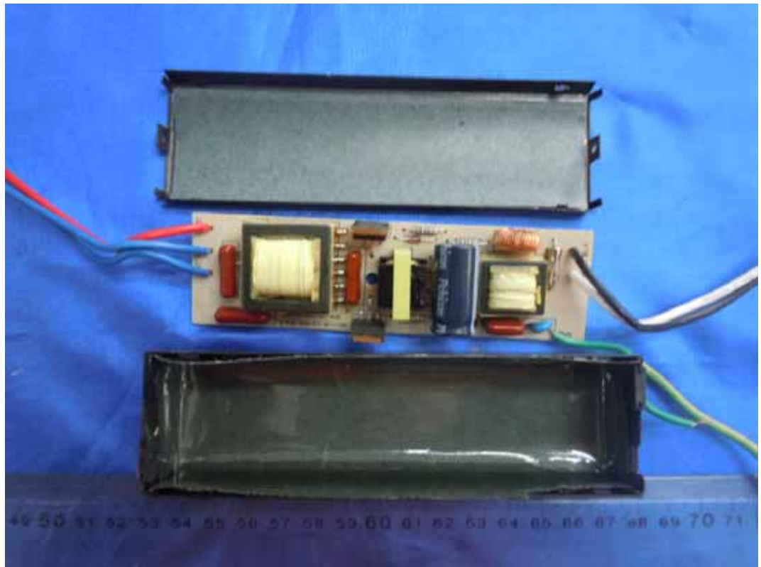
FIGURE 1 FLUORESCENT LAMP BALLAST (M/N: BEB/120/232) COVER REMOVED
