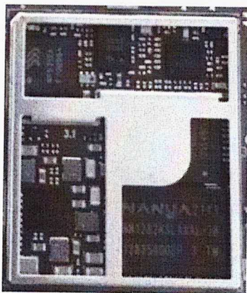
Figure 1: Module shield alternative 1
