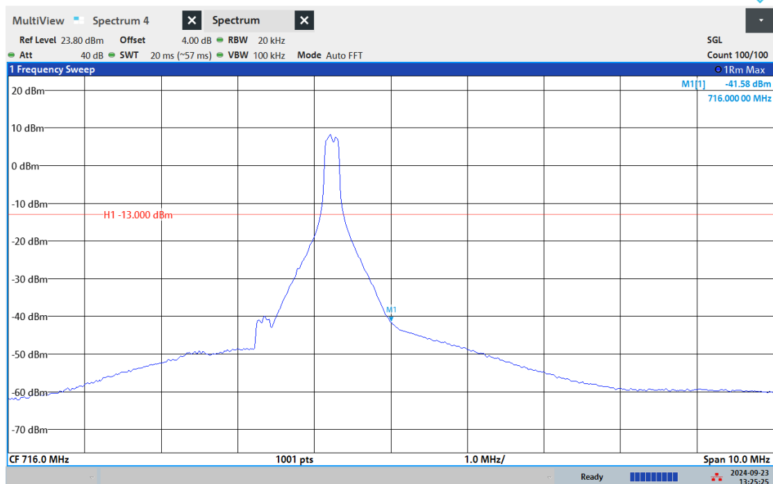
Band12-10MHz-QPSK-23130-6RB#0
