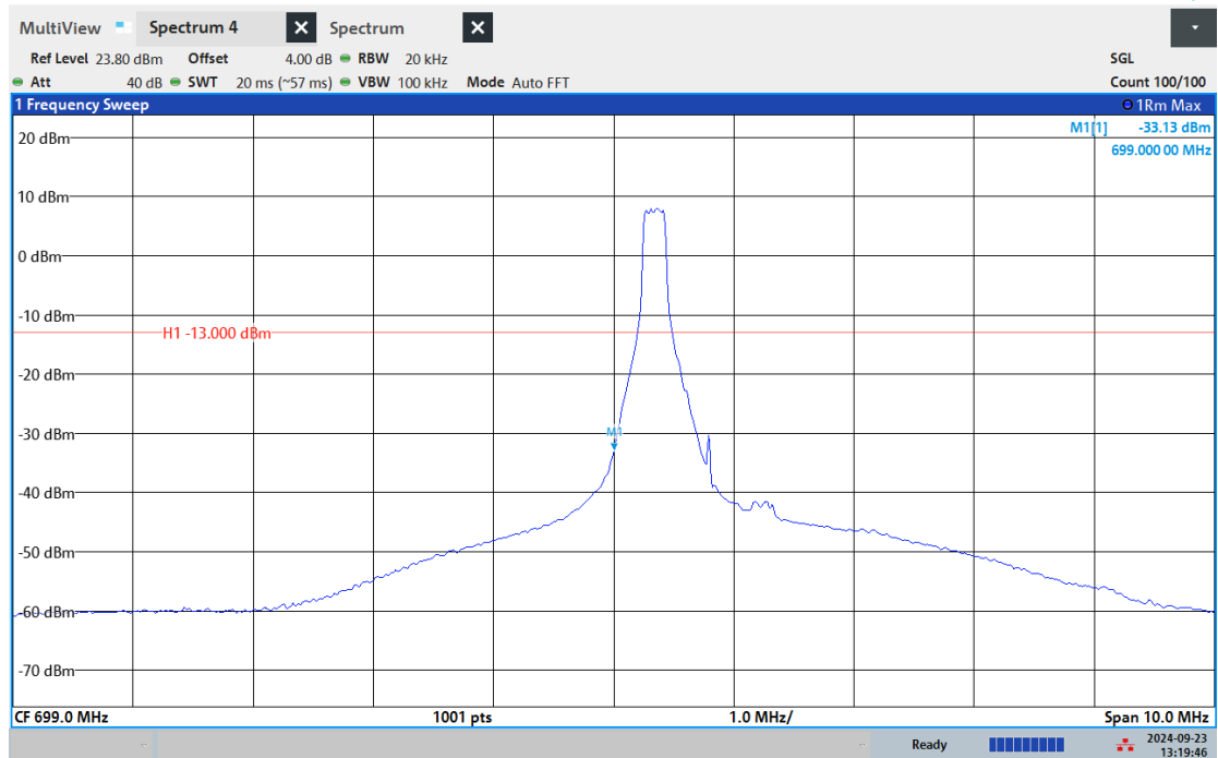
Band12-5MHz-16QAM-23035-6RB#0
