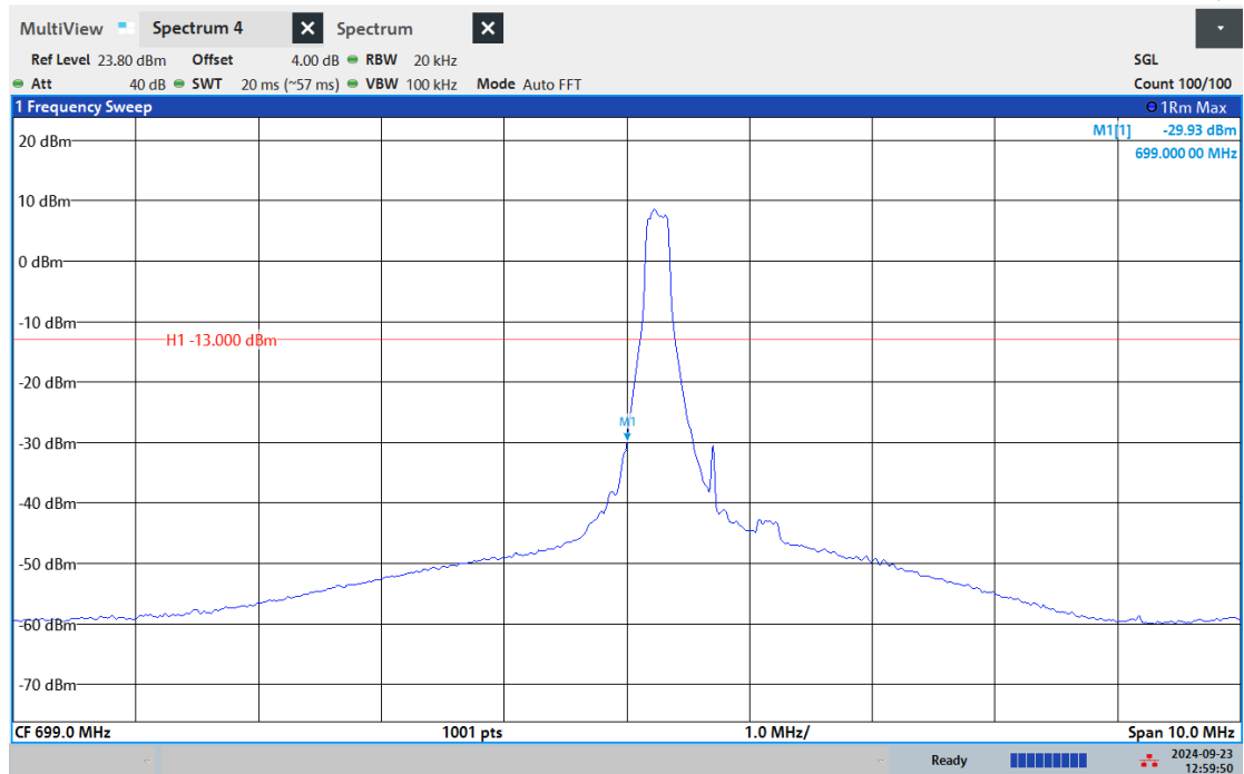
Band12-1.4MHz-QPSK-23017-6RB#0
