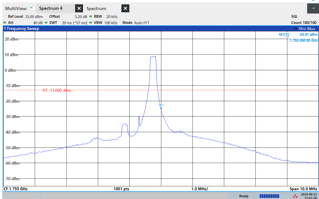
Band4-1.4MHz-16QAM-20393-6RB#0
