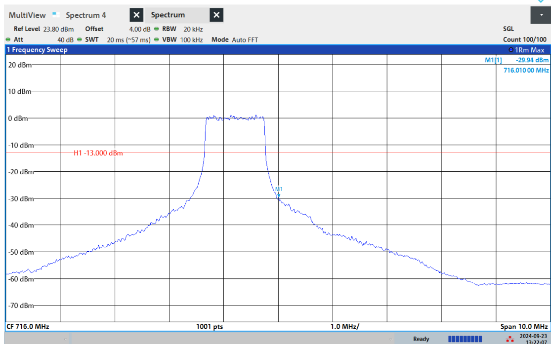
Band12-10MHz-QPSK-23060-1RB#0
