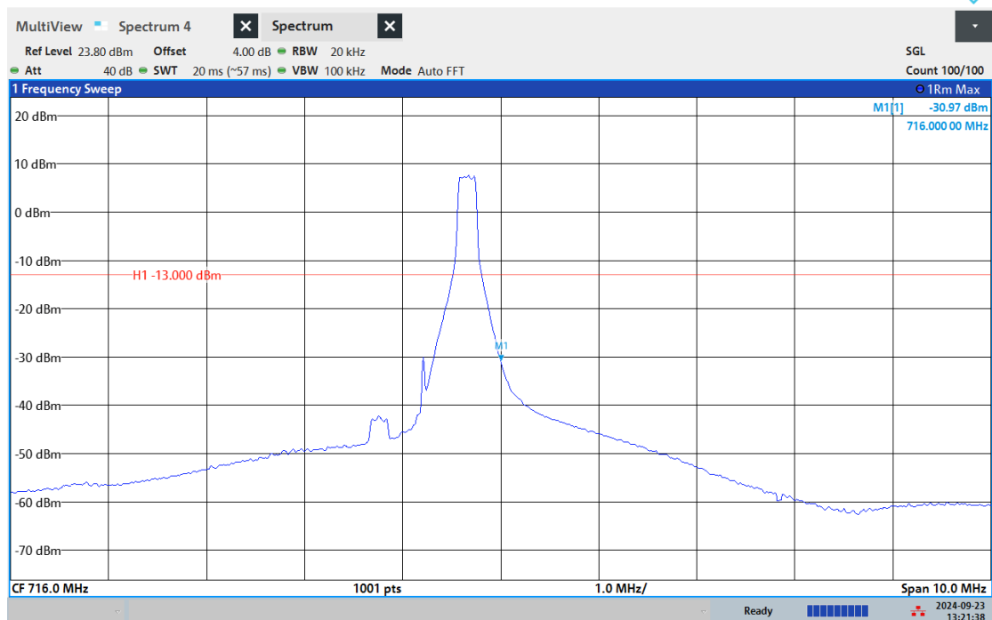
Band12-5MHz-16QAM-23155-6RB#0
