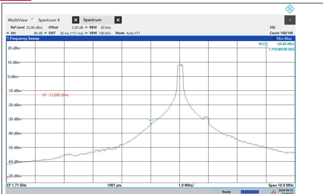
Band4-15MHz-QPSK-20025-6RB#0
