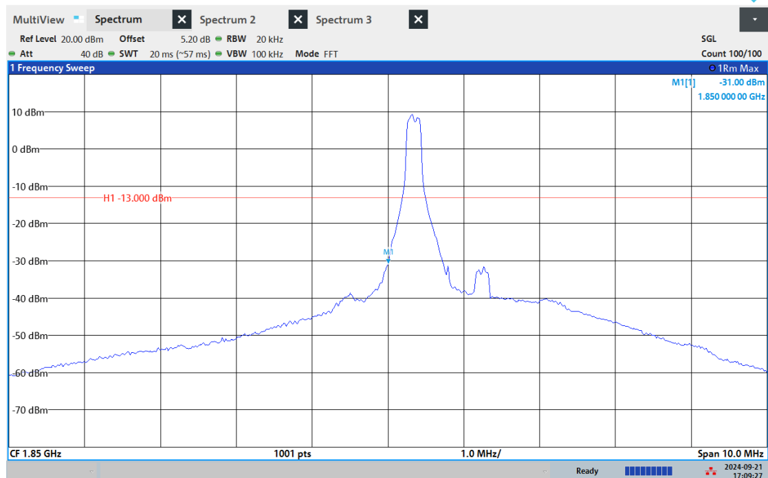
Band2-5MHz-QPSK-18625-6RB#0
