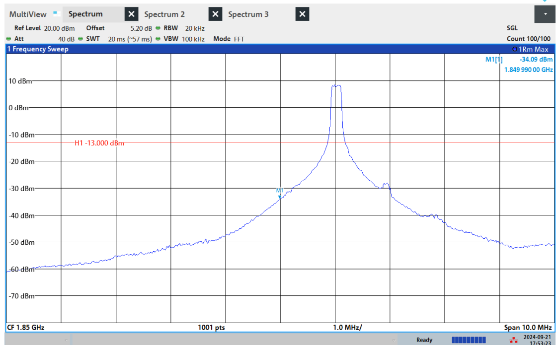
Band2-15MHz-16QAM-18675-6RB#0
