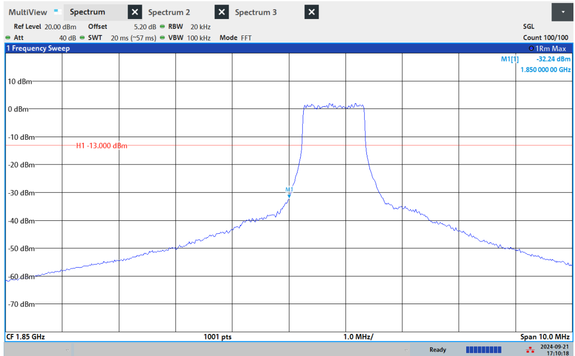
Band2-5MHz-QPSK-19175-1RB#5
