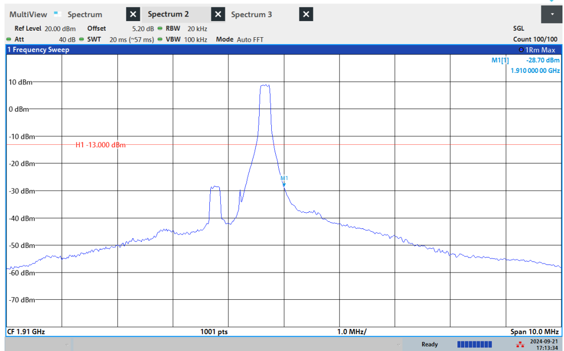
Band2-5MHz-16QAM-19175-6RB#0
