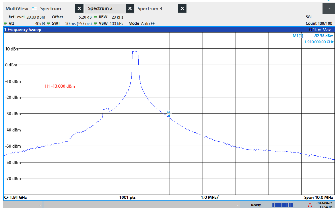
Band2-15MHz-16QAM-19125-6RB#0
