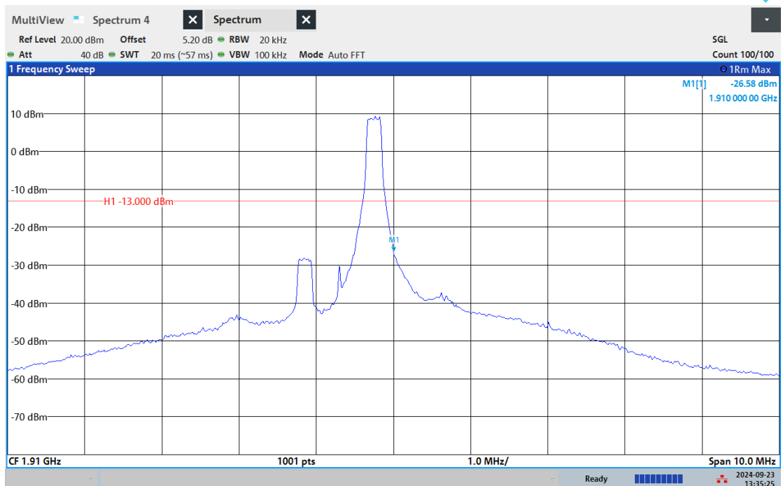
Band2-1.4MHz-16QAM-19193-6RB#0
