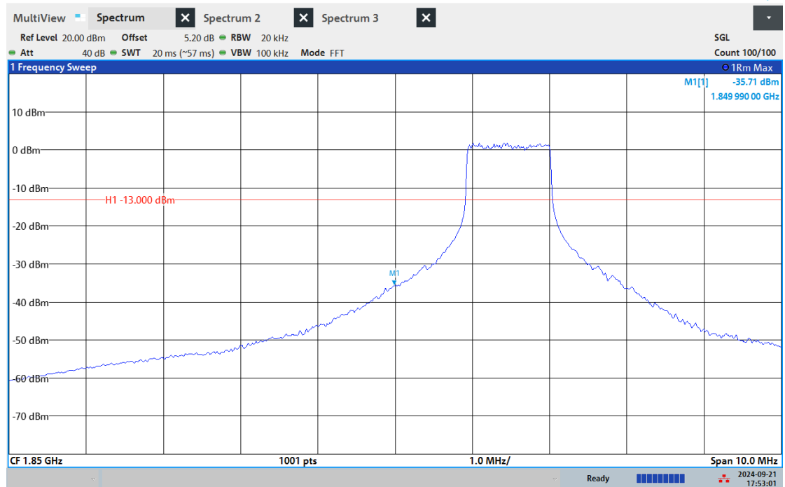
Band2-15MHz-16QAM-19125-1RB#5
