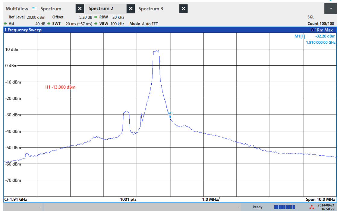
Band2-3MHz-16QAM-19185-6RB#0
