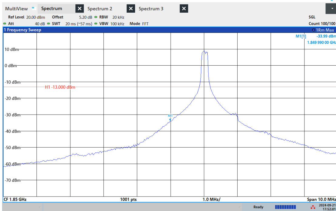
Band2-15MHz-QPSK-18675-6RB#0
