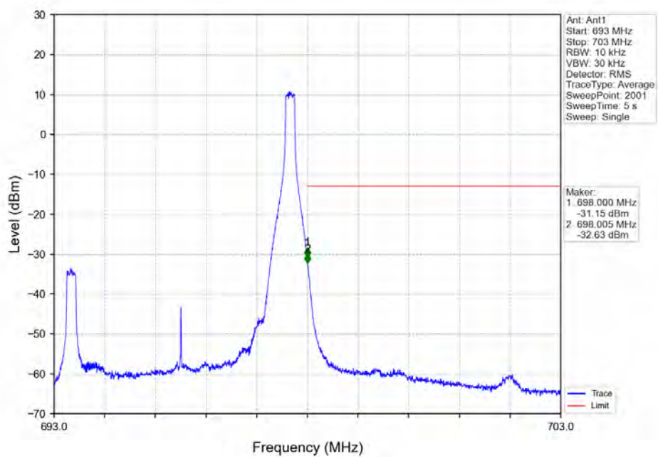
Band71_5MHz_16QAM_HCH_695.5MHz_RB_25_0_NTNV
