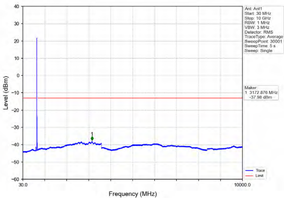
Band71_15MHz_16QAM_LCH_670.5MHz_RB_75_0_NTNV
