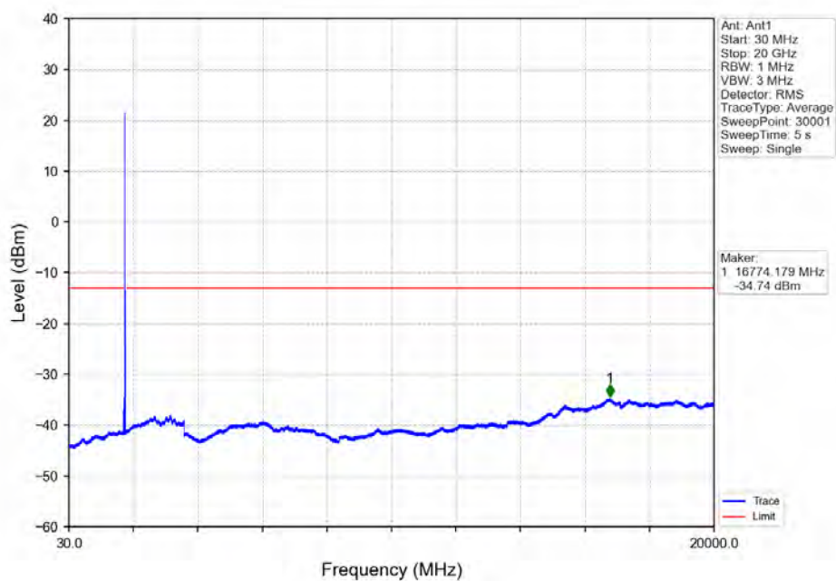
Band66_20MHz_16QAM_HCH_1770MHz_RB_1_0_NTNV
