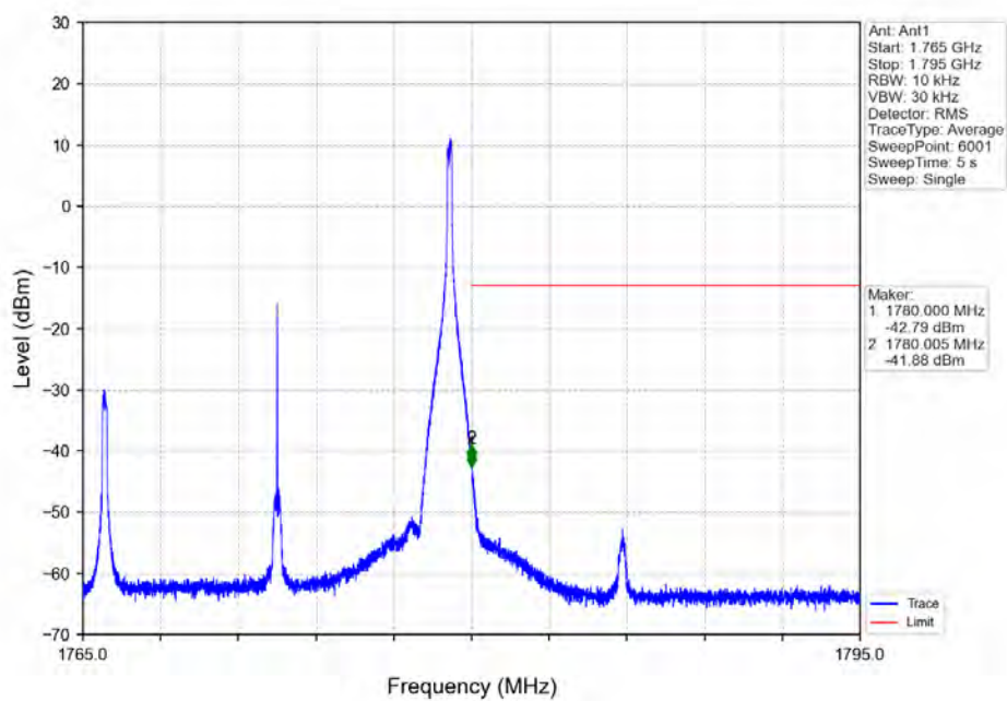
Band66_15MHz_16QAM_HCH_1772.5MHz_RB_75_0_NTNV
