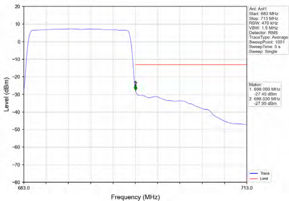
Band71_15MHz_16QAM_HCH_690.5MHz_RB_75_0_NTNV
