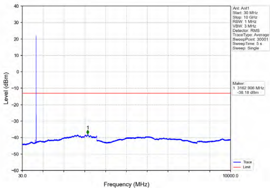
Band71_5MHz_16QAM_HCH_695.5MHz_RB_1_0_NTNV
