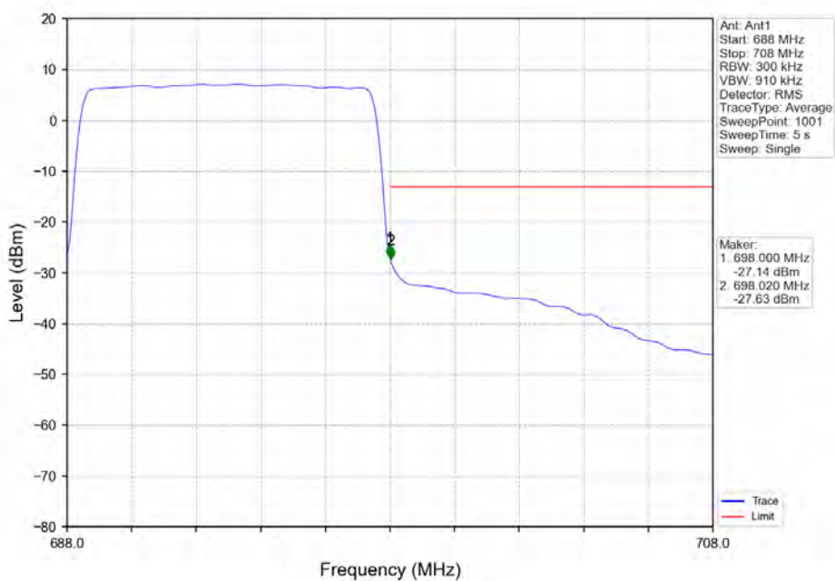
Band71_10MHz_16QAM_HCH_693MHz_RB_50_0_NTNV
