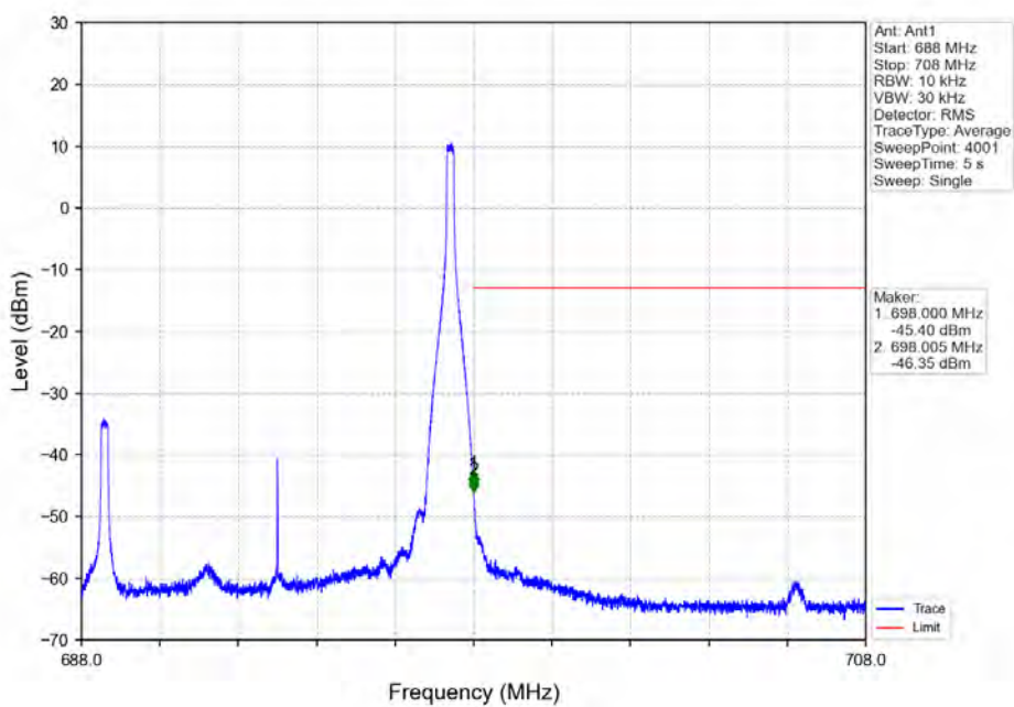
Band71_10MHz_16QAM_HCH_693MHz_RB_50_0_NTNV
