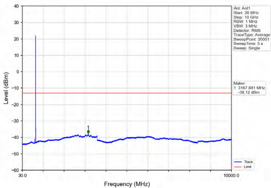
Band71_5MHz_16QAM_LCH_665.5MHz_RB_25_0_NTNV
