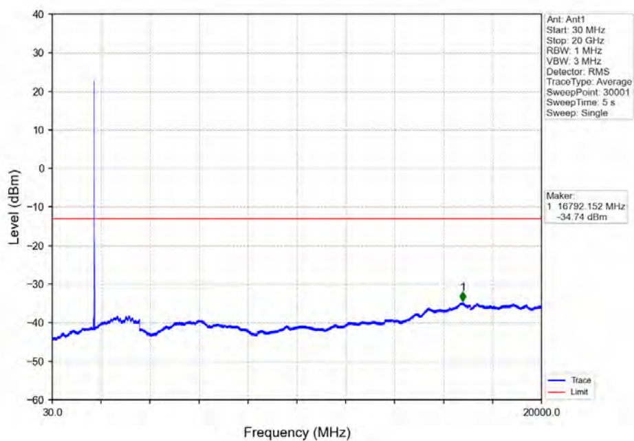
Band66_15MHz_QPSK_MCH_1745MHz_RB_1_0_NTNV
