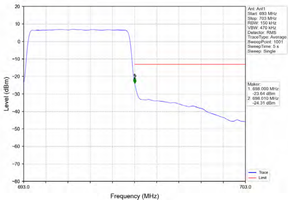
Band71_5MHz_16QAM_HCH_695.5MHz_RB_25_0_NTNV
