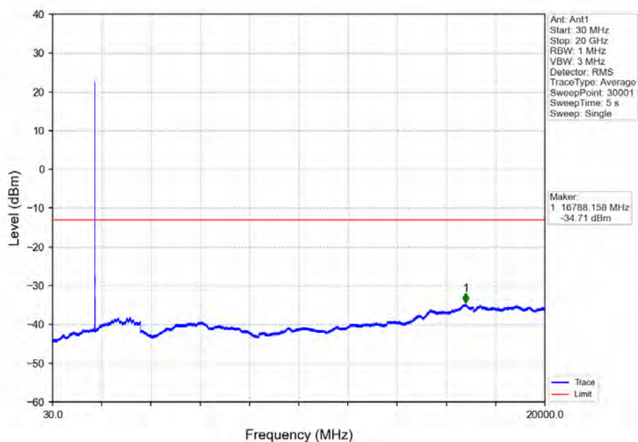
Band66_5MHz_16QAM_HCH_1777.5MHz_RB_1_0_NTNV
