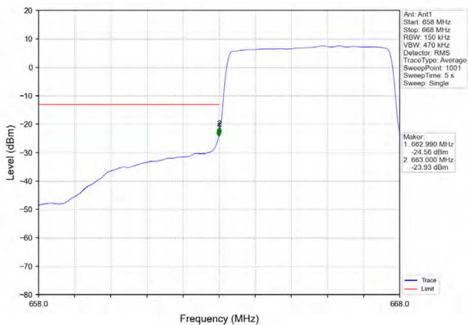
Band71_5MHz_16QAM_LCH_665.5MHz_RB_25_0_NTNV
