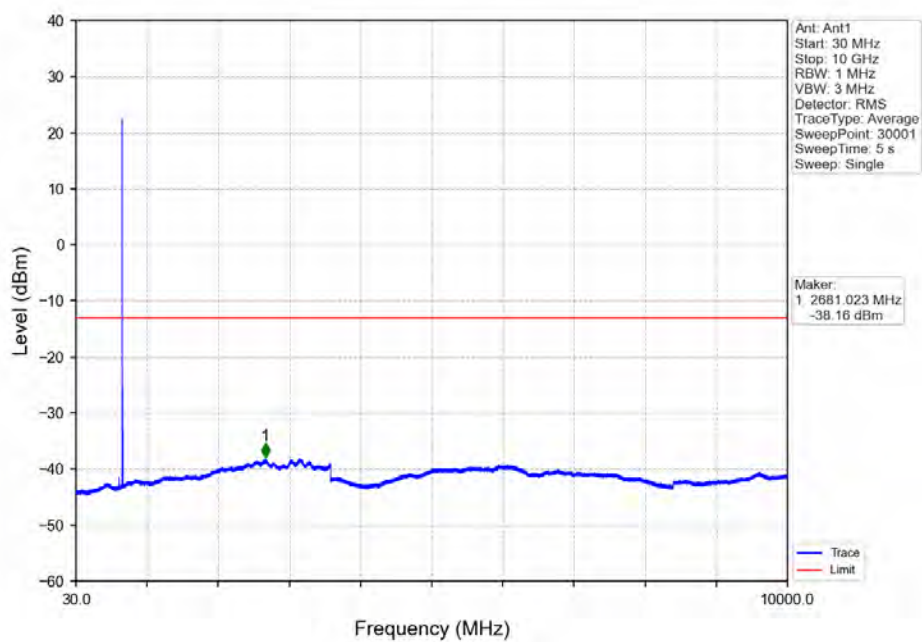
Band71_5MHz_16QAM_HCH_695.5MHz_RB_1_0_NTNV
