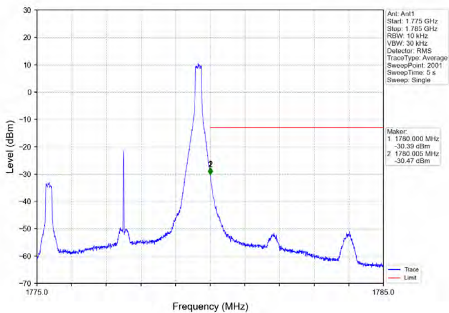
Band66_5MHz_16QAM_HCH_1777.5MHz_RB_25_0_NTNV
