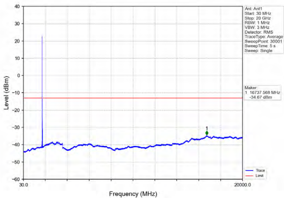
Band66_20MHz_16QAM_HCH_1770MHz_RB_1_0_NTNV
