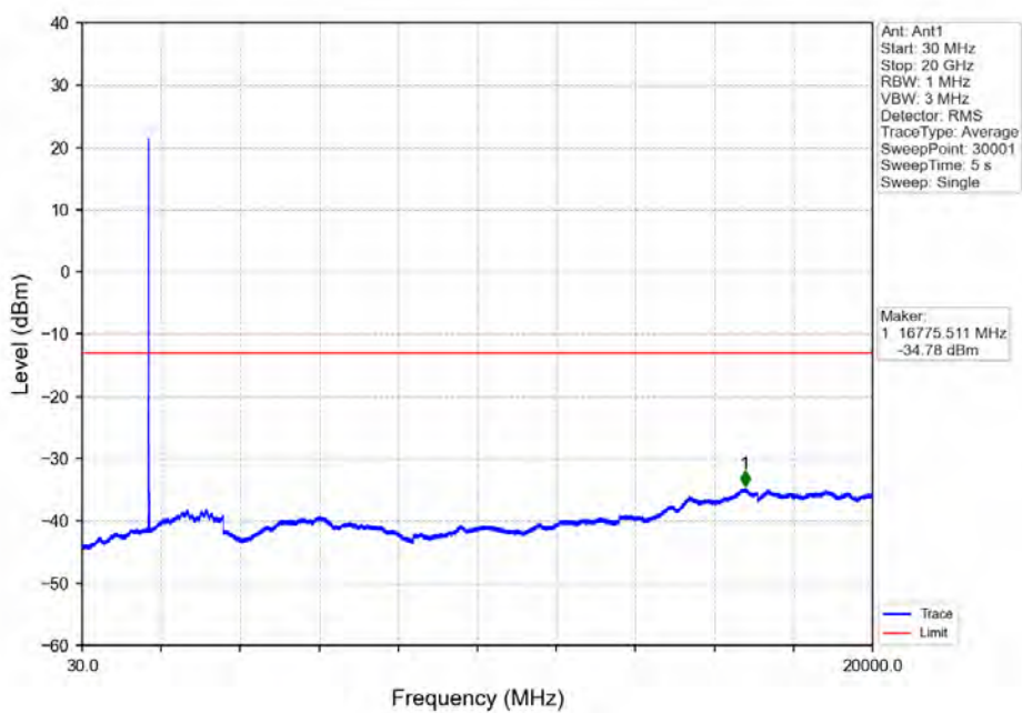
Band66_10MHz_16QAM_LCH_1715MHz_RB_50_0_NTNV
