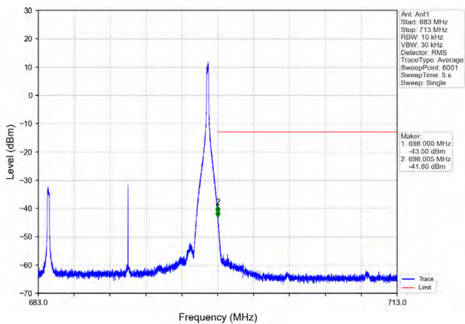
Band71_15MHz_16QAM_HCH_690.5MHz_RB_75_0_NTNV
