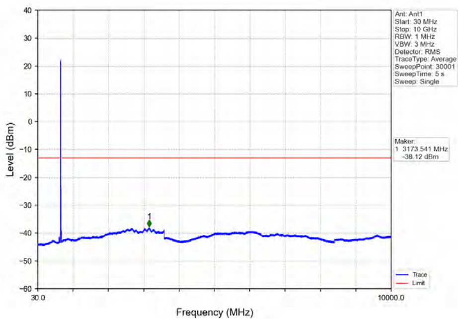
Band71_15MHz_16QAM_HCH_690.5MHz_RB_1_0_NTNV
