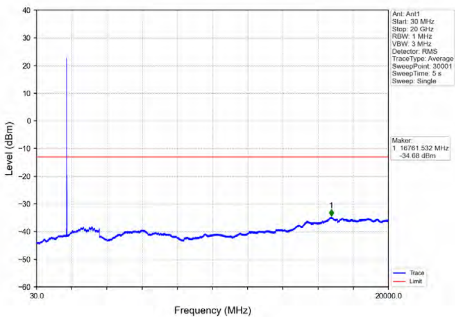
Band66_10MHz_16QAM_HCH_1775MHz_RB_1_0_NTNV
