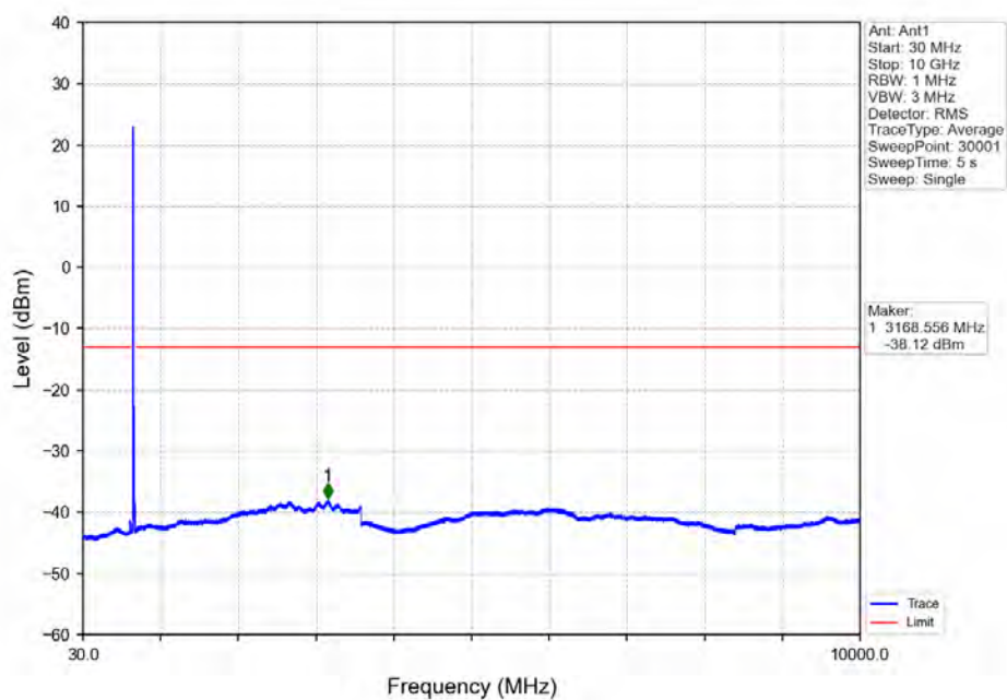
Band71_15MHz_QPSK_MCH_680.5MHz_RB_1_0_NTNV
