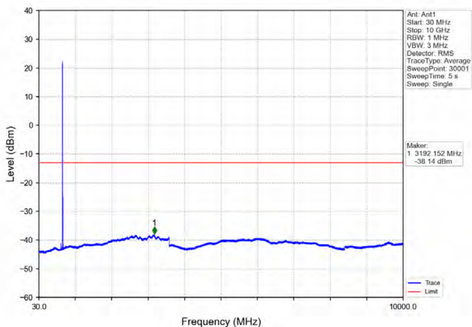
Band71_10MHz_16QAM_HCH_693MHz_RB_1_0_NTNV
