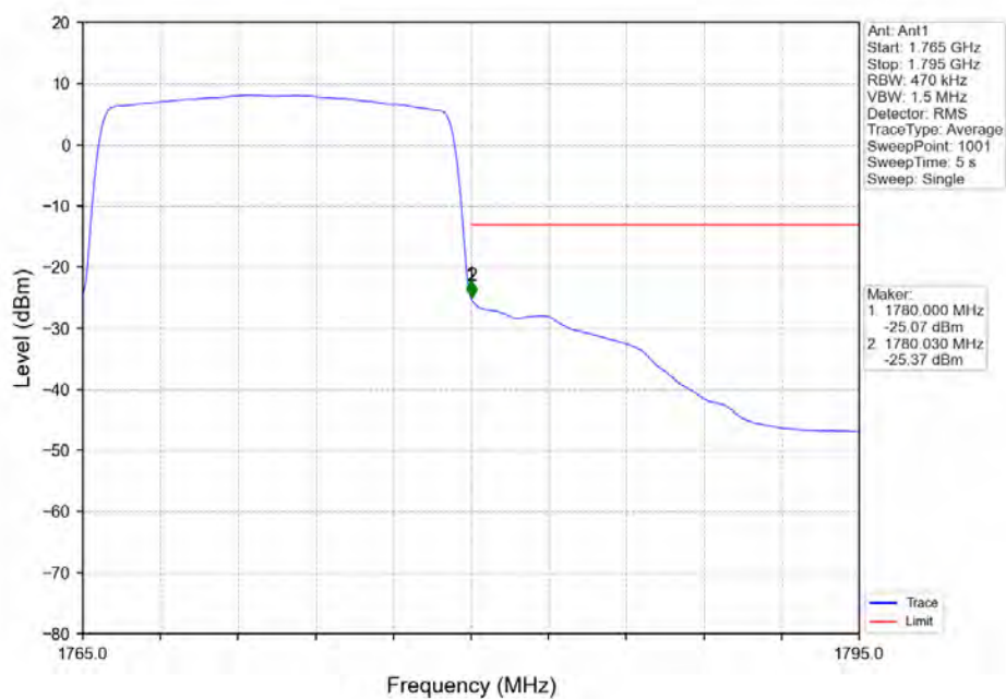
Band66_15MHz_16QAM_HCH_1772.5MHz_RB_75_0_NTNV
