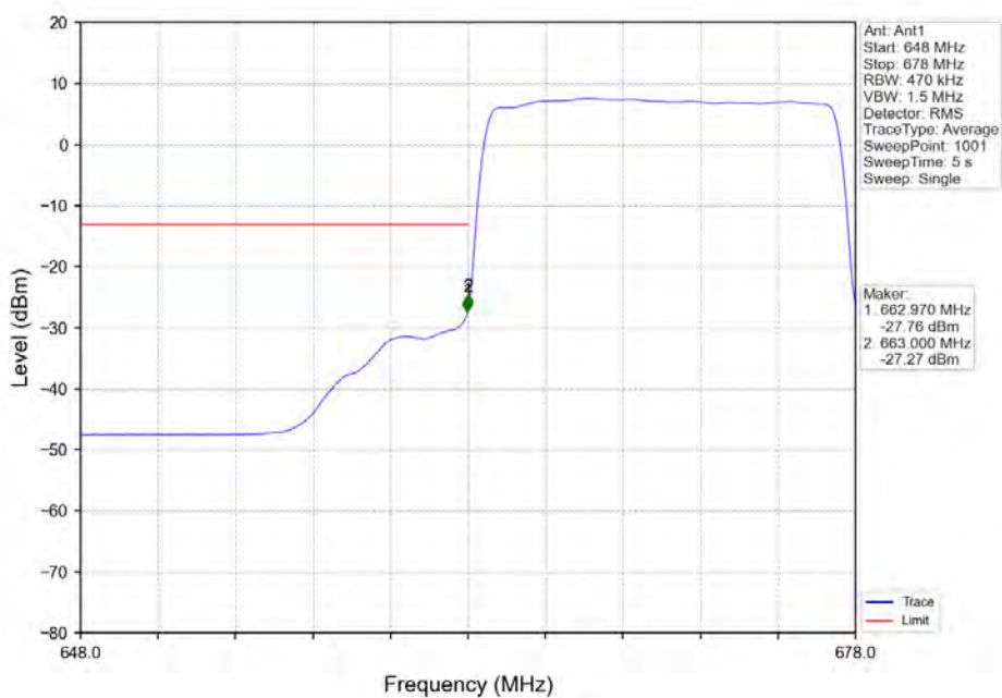
Band71_15MHz_16QAM_LCH_670.5MHz_RB_75_0_NTNV
