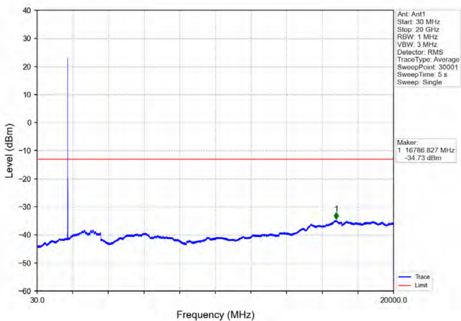
Band66_10MHz_QPSK_MCH_1745MHz_RB_1_0_NTNV
