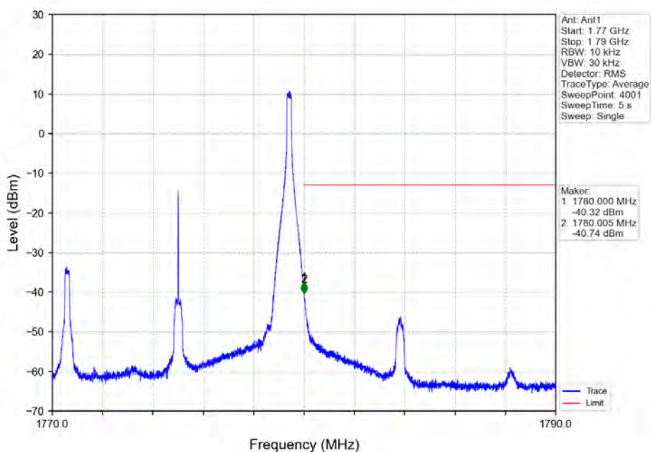
Band66_10MHz_16QAM_HCH_1775MHz_RB_50_0_NTNV
