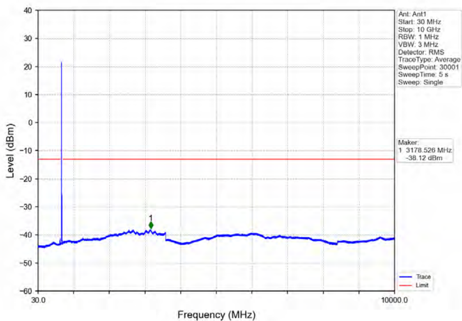
Band71_15MHz_16QAM_HCH_690.5MHz_RB_1_0_NTNV
