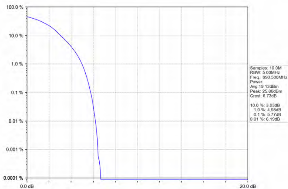
Band71_15MHz_QPSK_HCH_690.5MHz_RB_75_0_NTNV
