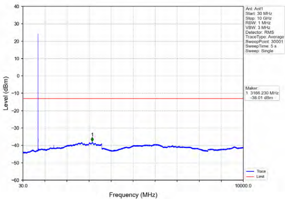
Band12_3MHz_QPSK_HCH_714.5MHz_RB_1_14_NTNV
