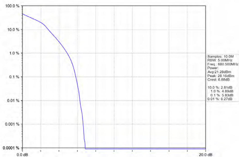
Band71_5MHz_16QAM_MCH_680.5MHz_RB_25_0_NTNV
