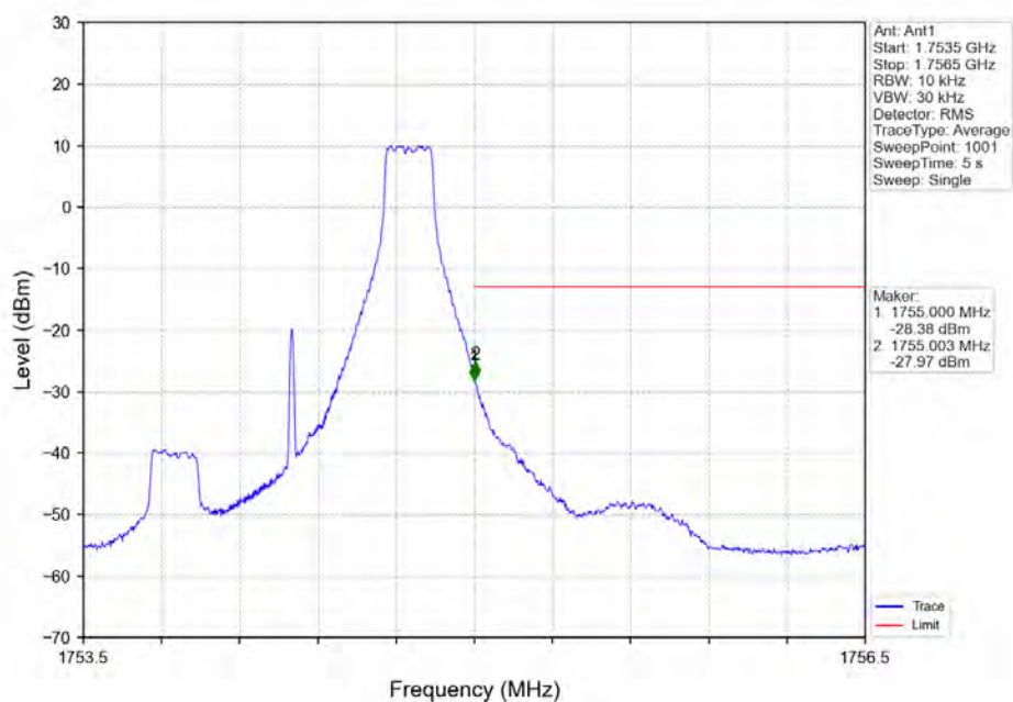
Band4_1.4MHz_16QAM_HCH_1754.3MHz_RB_6_0_NTNV
