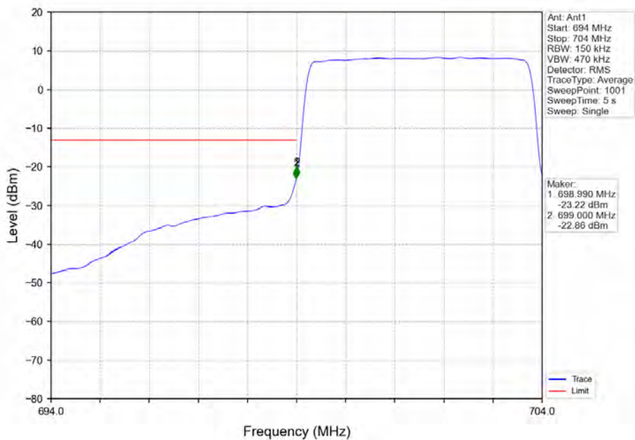
Band12_5MHz_16QAM_LCH_701.5MHz_RB_25_0_NTNV
