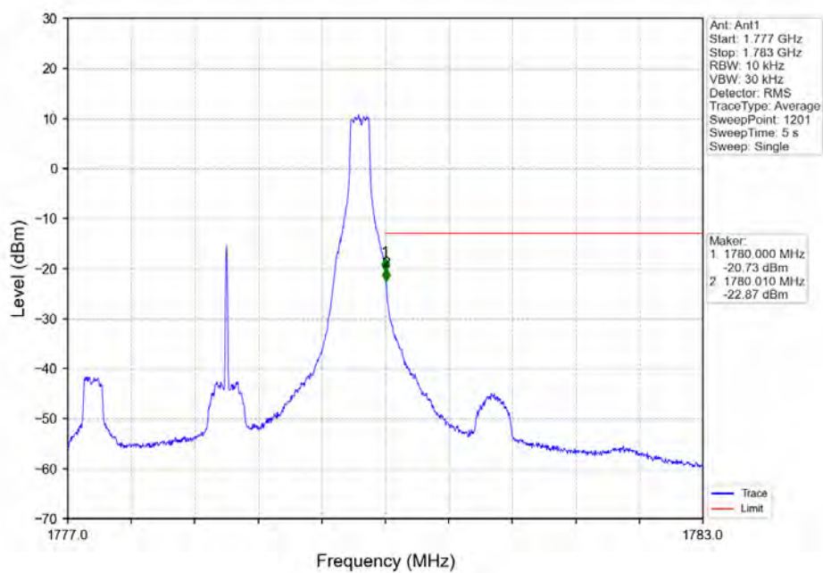
Band66_3MHz_16QAM_HCH_1778.5MHz_RB_15_0_NTNV
