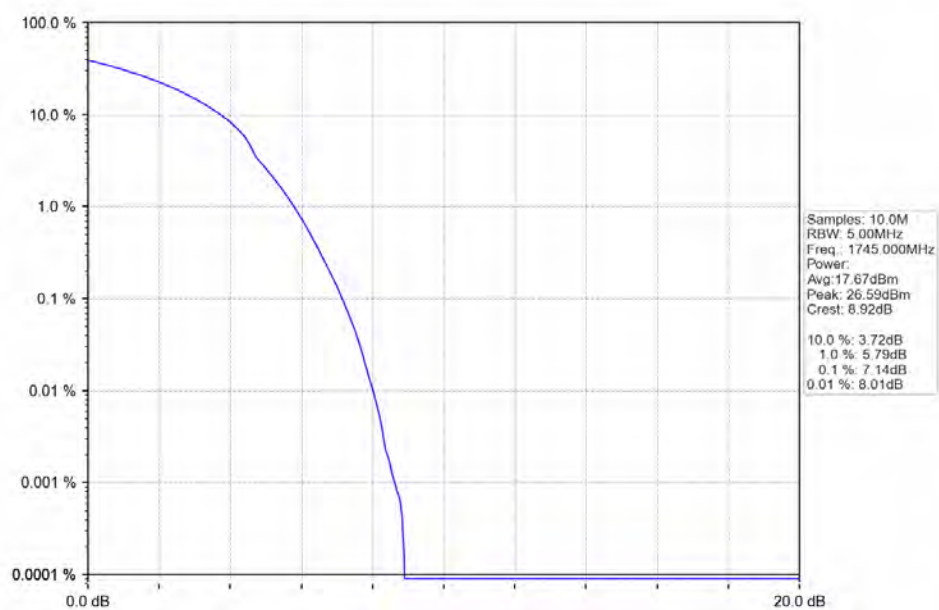
Band66_20MHz_16QAM_MCH_1745MHz_RB_100_0_NTNV
