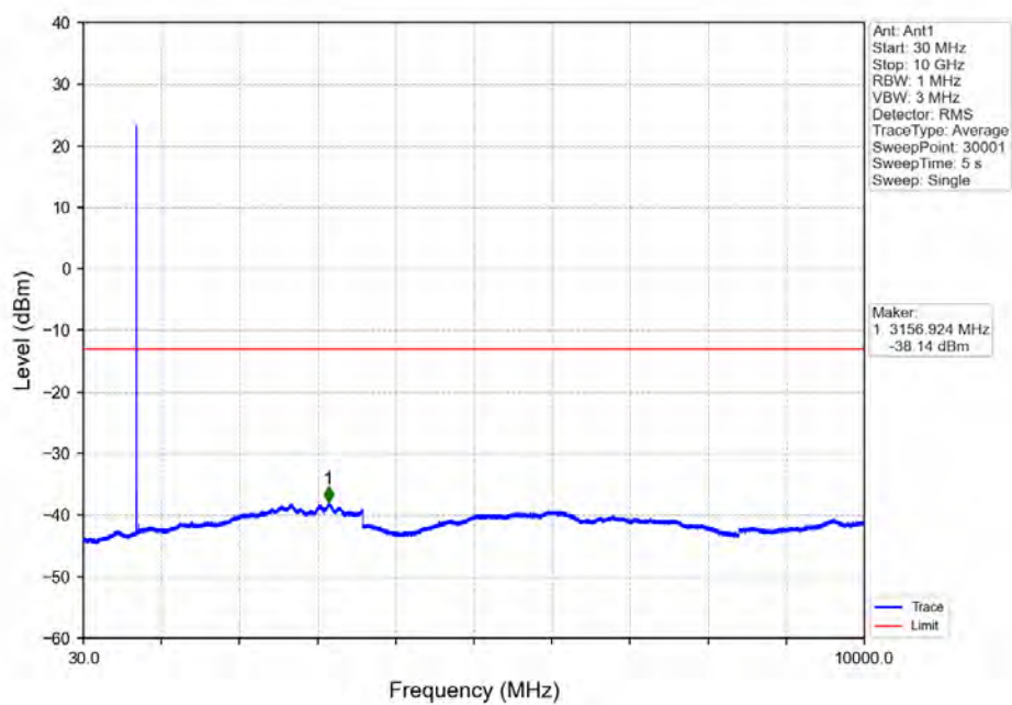
Band12_3MHz_16QAM_HCH_714.5MHz_RB_1_0_NTNV
