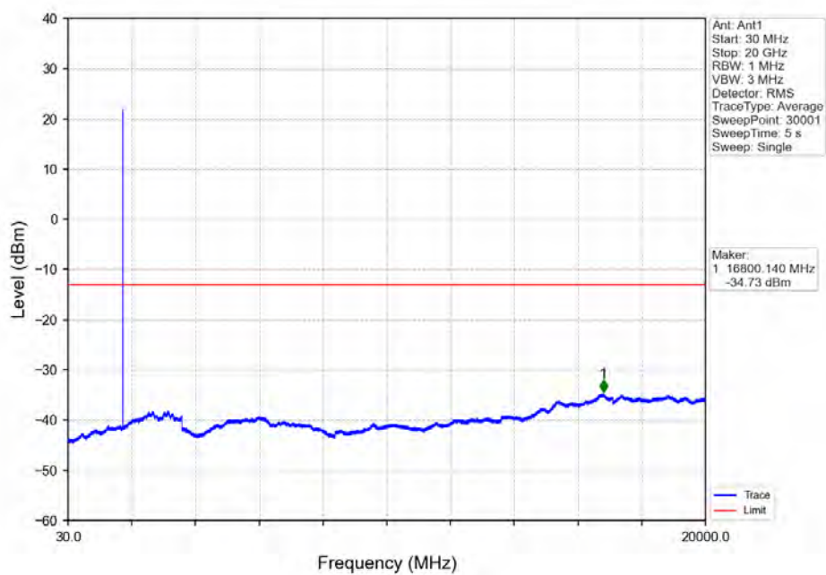
Band66_1.4MHz_16QAM_HCH_1779.3MHz_RB_1_0_NTNV
