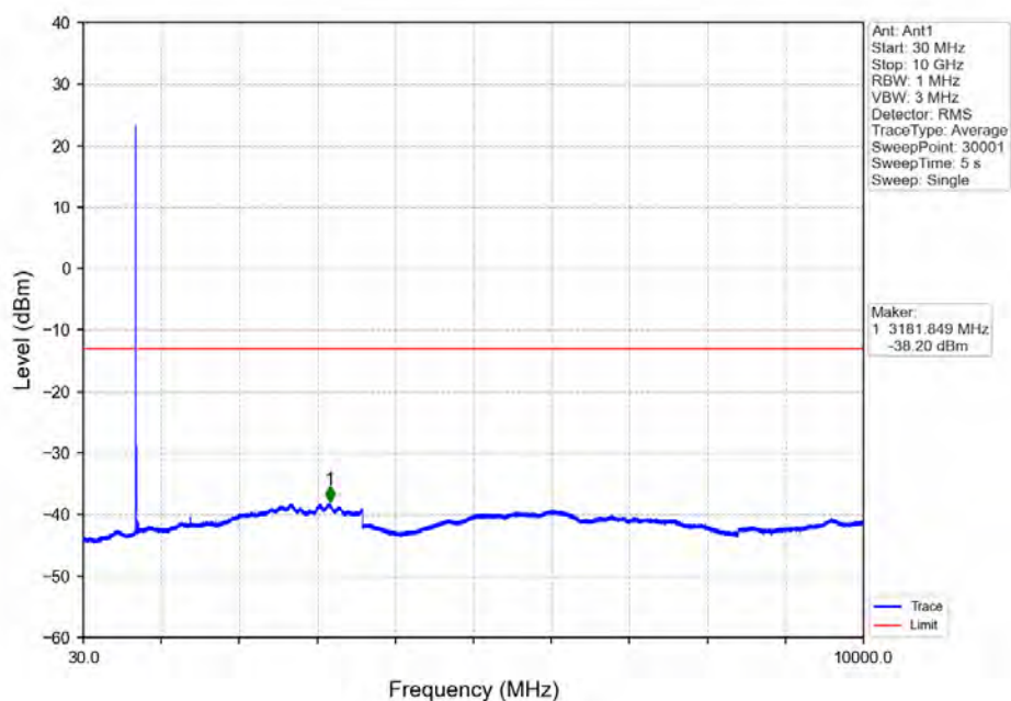
Band12_10MHz_16QAM_LCH_704MHz_RB_50_0_NTNV
