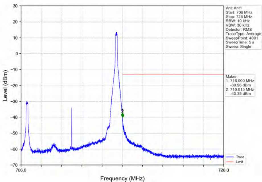
Band12_10MHz_QPSK_HCH_711MHz_RB_1_49_NTNV
