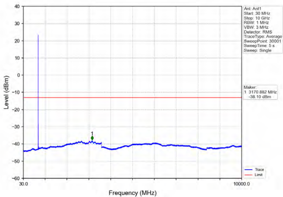
Band12_5MHz_16QAM_HCH_713.5MHz_RB_1_0_NTNV
