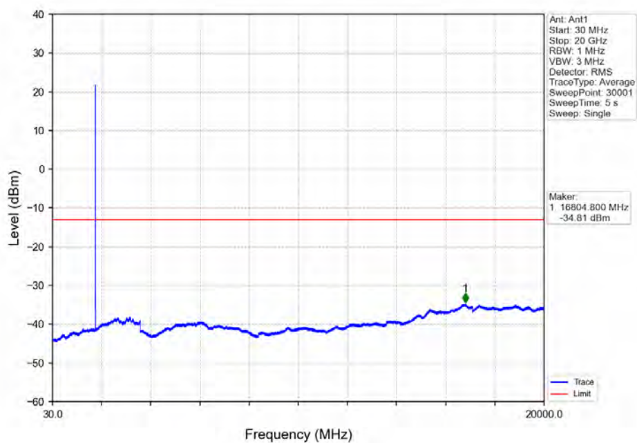
Band66_3MHz_16QAM_HCH_1778.5MHz_RB_1_0_NTNV
