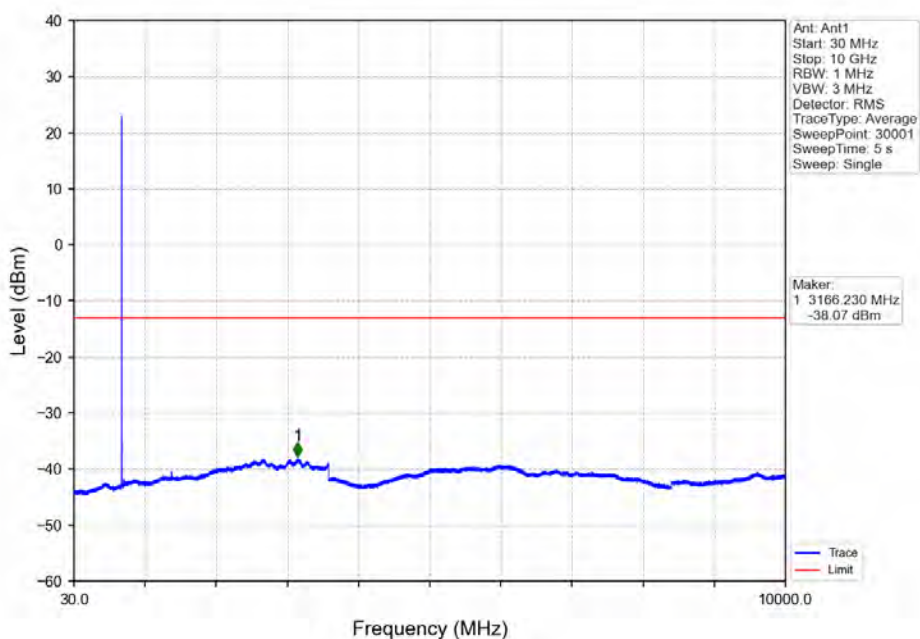
Band12_3MHz_16QAM_LCH_700.5MHz_RB_15_0_NTNV
