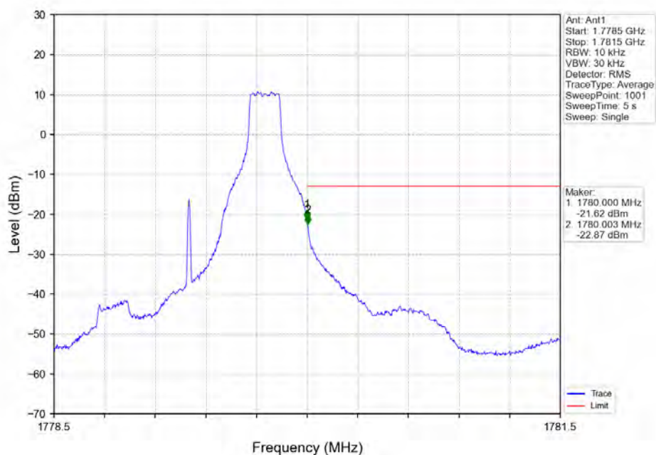
Band66_1.4MHz_16QAM_HCH_1779.3MHz_RB_6_0_NTNV
