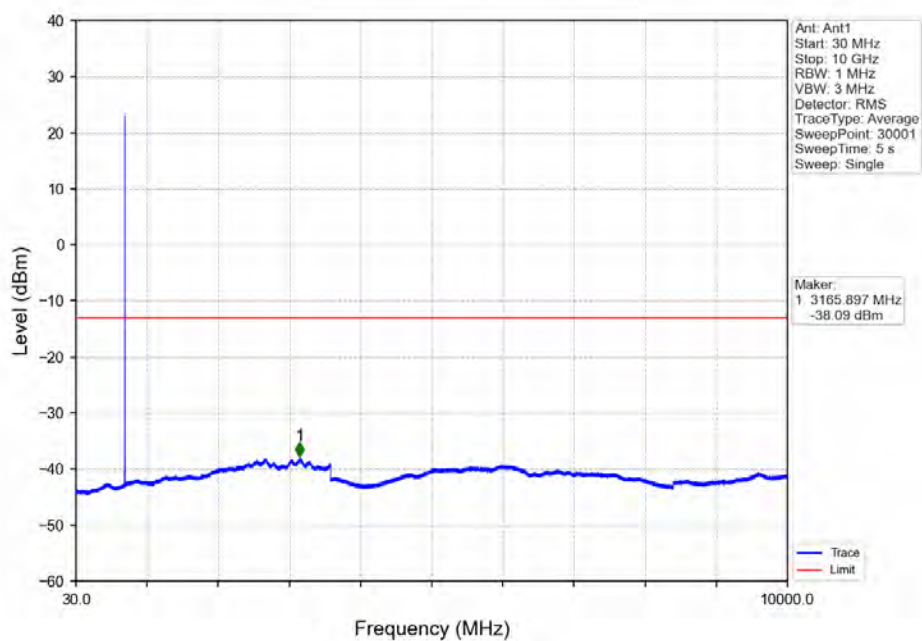
Band12_1.4MHz_16QAM_HCH_715.3MHz_RB_1_0_NTNV
