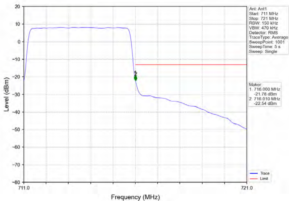
Band12_5MHz_16QAM_HCH_713.5MHz_RB_25_0_NTNV
