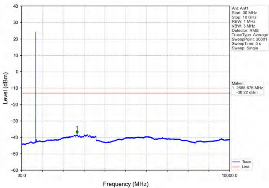
Band12_10MHz_QPSK_HCH_711MHz_RB_1_49_NTNV
