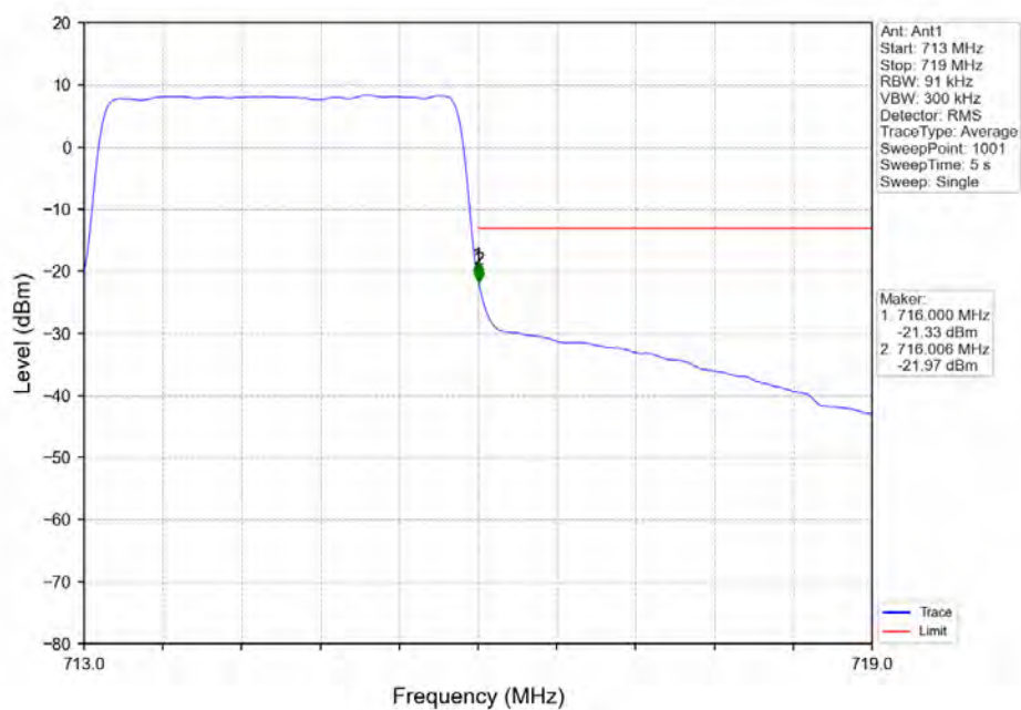
Band12_3MHz_16QAM_HCH_714.5MHz_RB_15_0_NTNV
