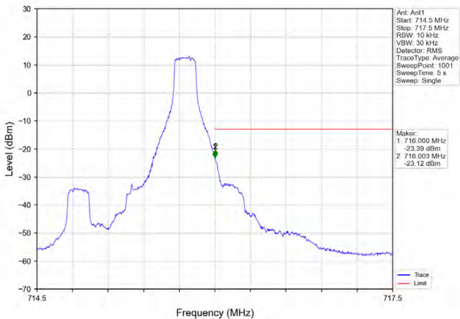
Band12_1.4MHz_QPSK_HCH_715.3MHz_RB_1_5_NTNV
