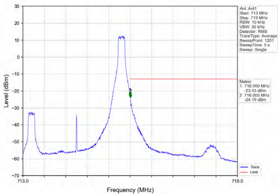
Band12_3MHz_16QAM_HCH_714.5MHz_RB_15_0_NTNV
