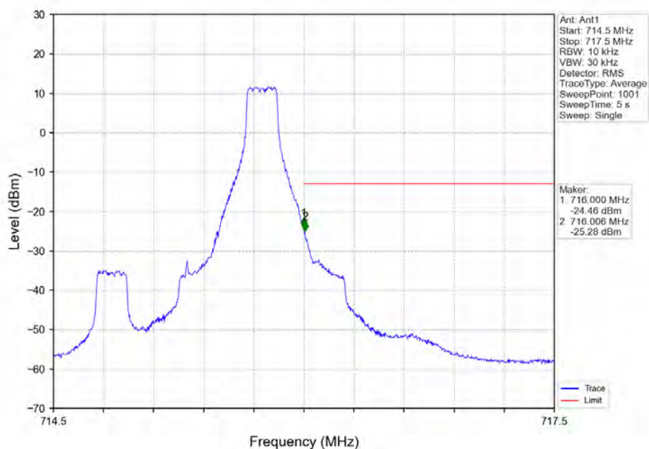
Band12_1.4MHz_16QAM_HCH_715.3MHz_RB_6_0_NTNV
