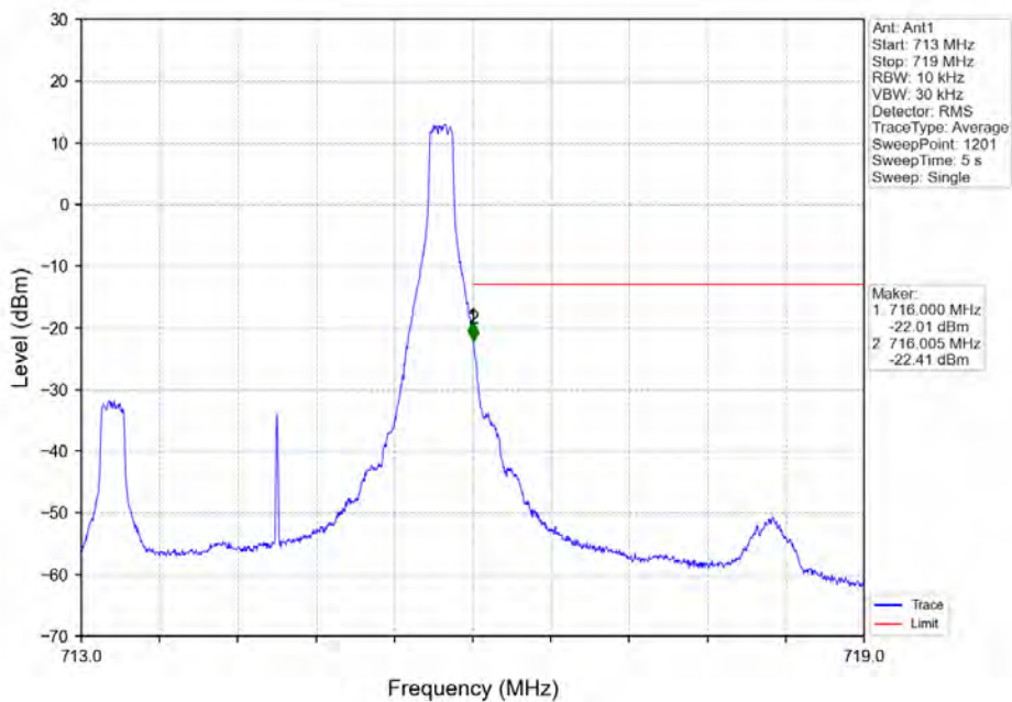
Band12_3MHz_QPSK_HCH_714.5MHz_RB_1_14_NTNV
