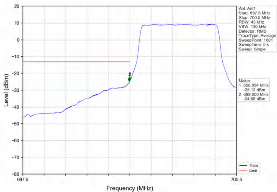
Band12_1.4MHz_16QAM_LCH_699.7MHz_RB_6_0_NTNV
