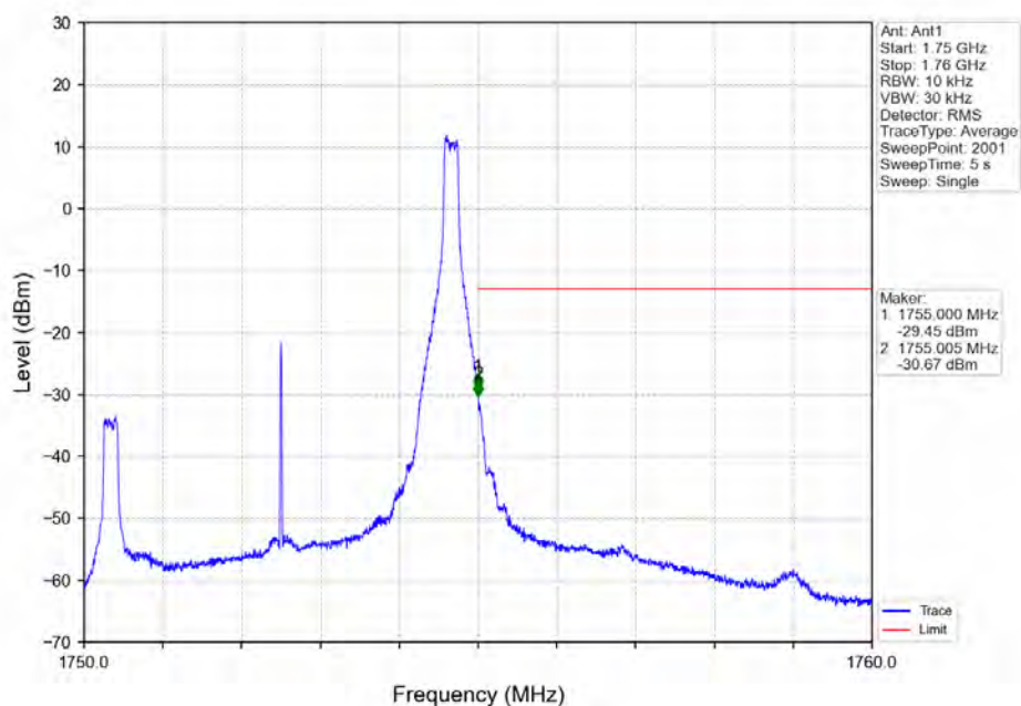
Band4_5MHz_QPSK_HCH_1752.5MHz_RB_1_24_NTNV
