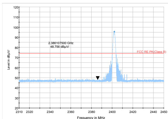
3DH5-Channel 0: Peak
