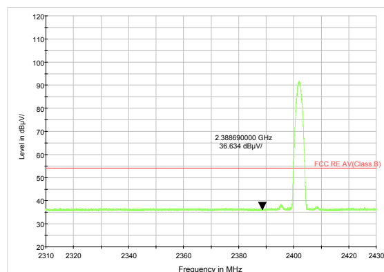
3DH5-Channel 0: Average
