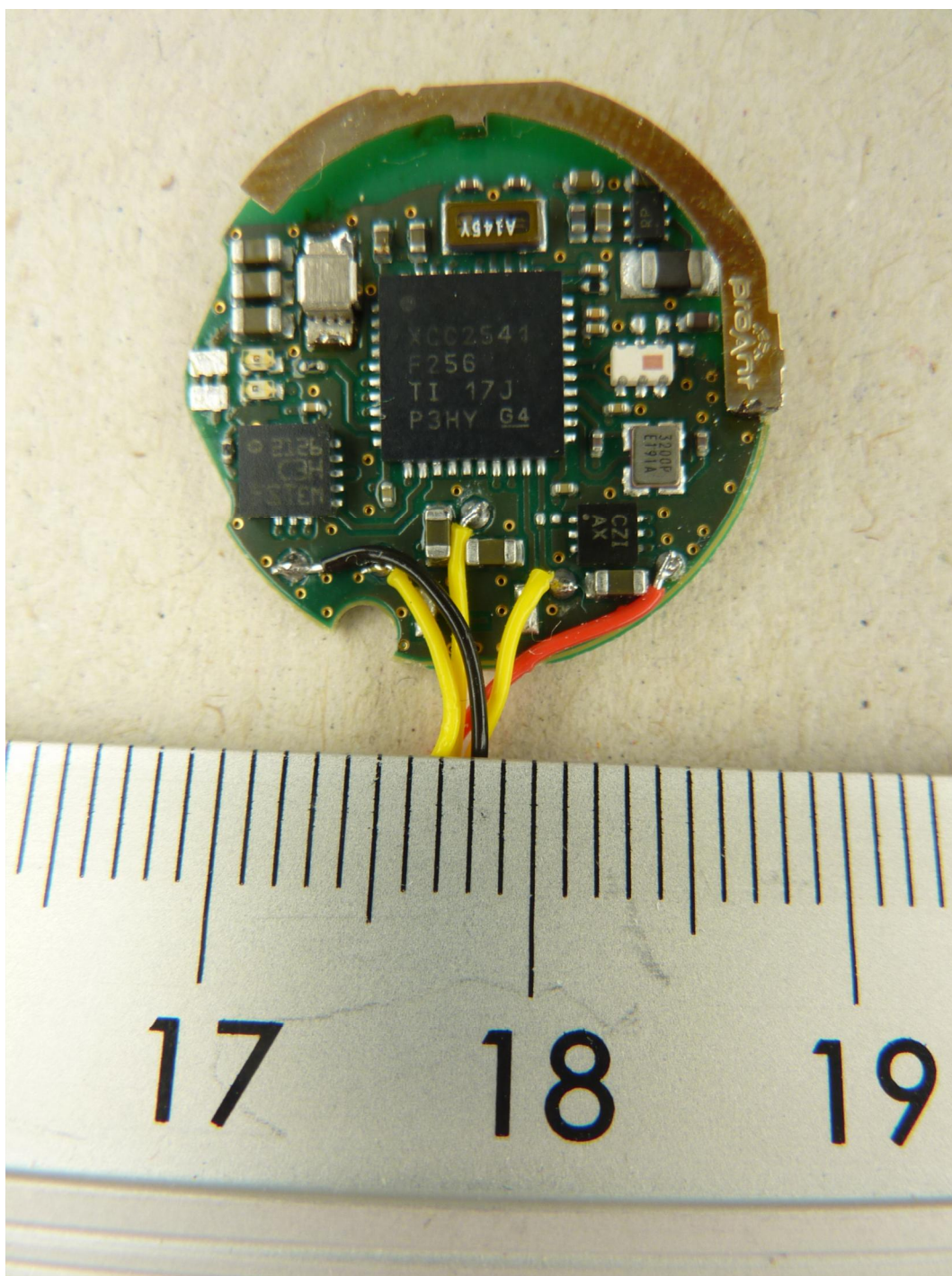
120795_13.JPG: EUT w. internal antenna, w. programming interface, top view
