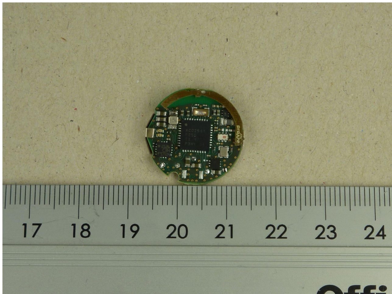
120795_15.JPG: EUT w. internal antenna, top view
