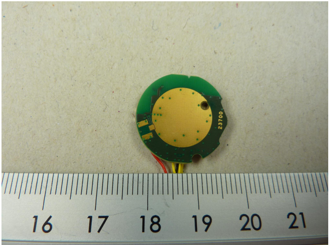
120795_11.JPG: EUT w. internal antenna, w. programming interface, bottom view
