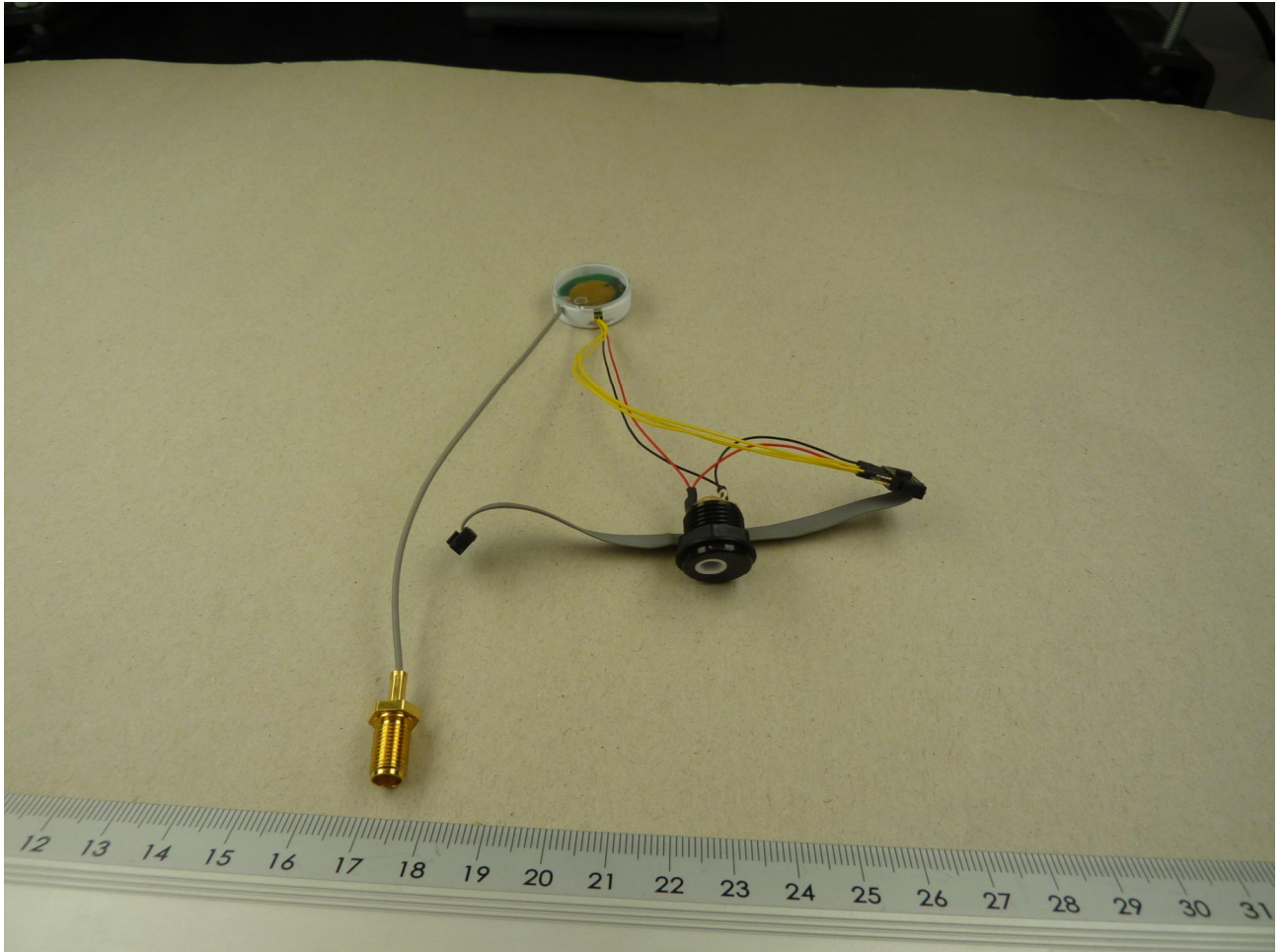
120795_9.JPG: EUT w. antenna connector, w. dc line / programming interface, bottom view
