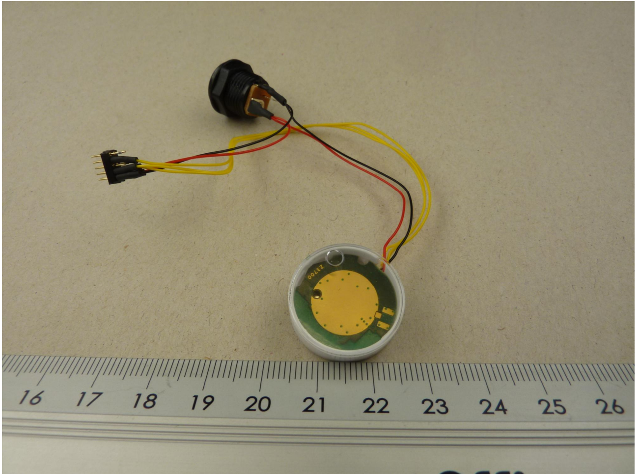
120795_7.JPG: EUT w. internal Antenna, w. dc line / programming interface, bottom view
