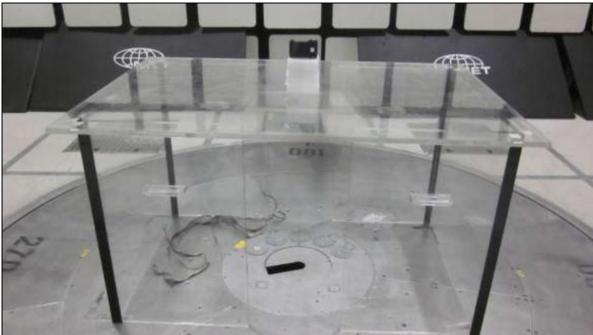
Photograph 12. Radiated Emissions, Test Setup, Front View
