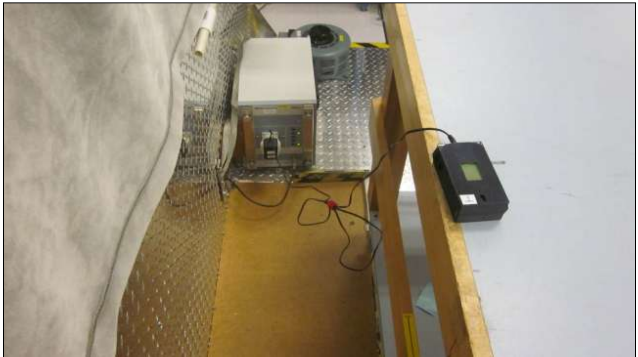
Photograph 6. 15.207 Conducted Emissions, Test Setup
