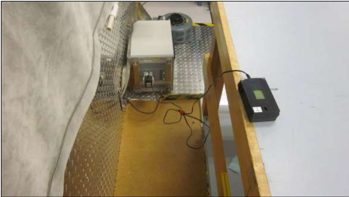
Photograph 2. Conducted Emissions, Test Setup, Rear View
