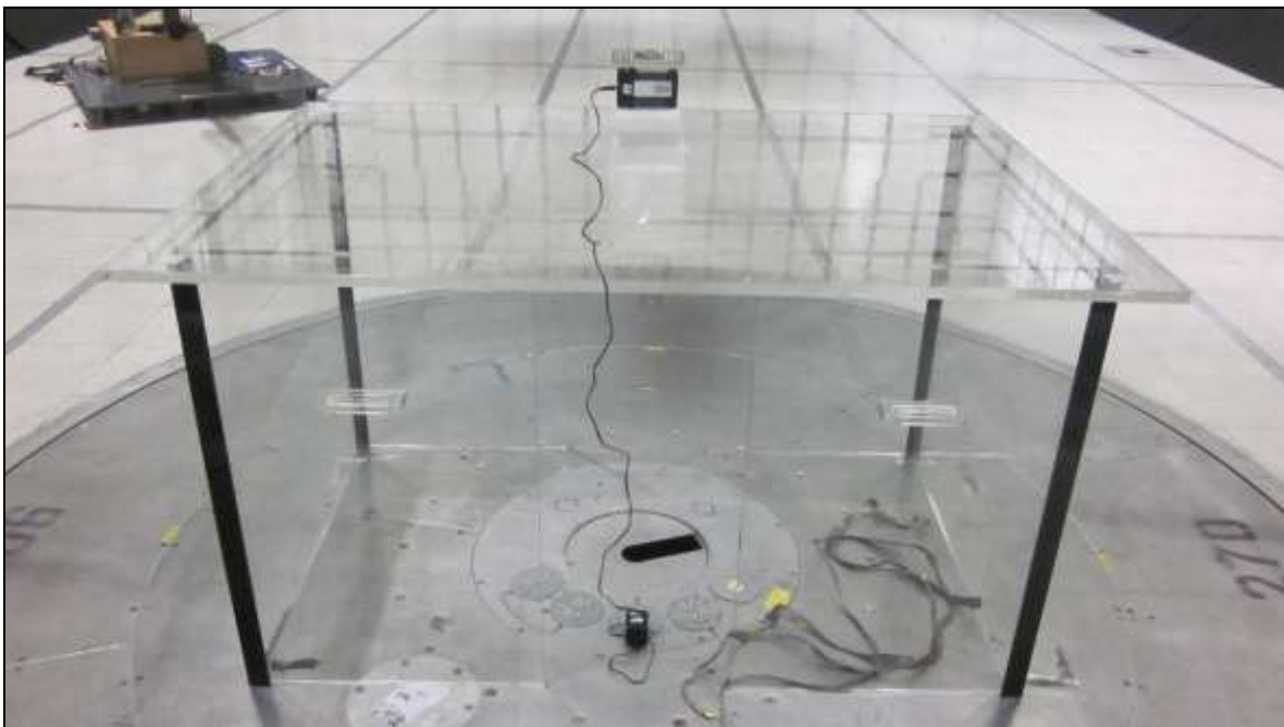
Photograph 4. Radiated Emissions, Test Setup, Rear View
