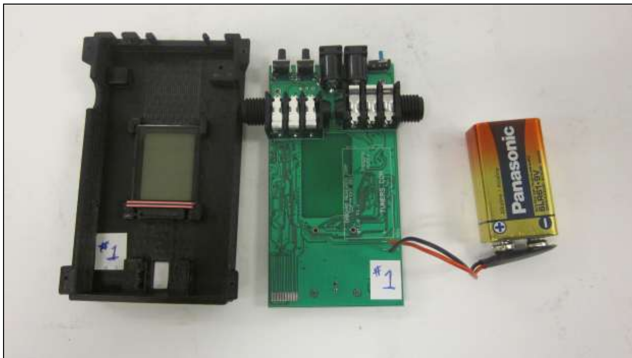
Photograph 3. battery, internal top housing with bottom of PCB
