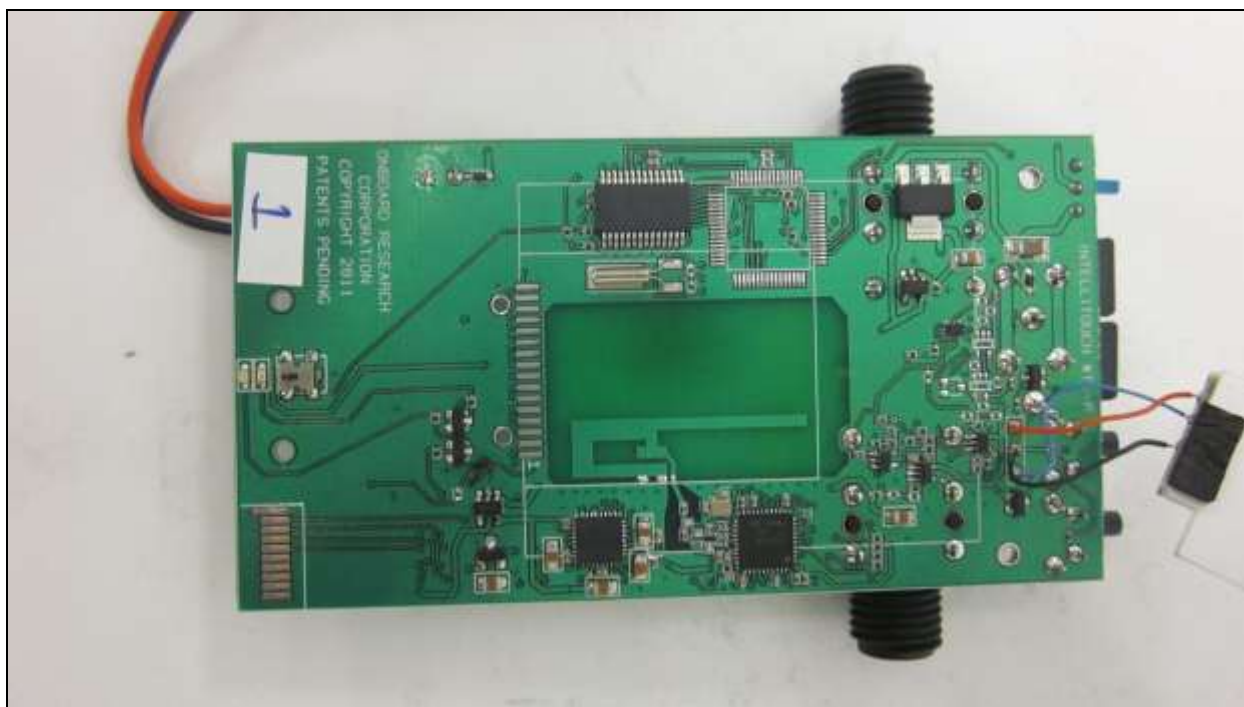
Photograph 9. Top of PCB with antenna exposed
