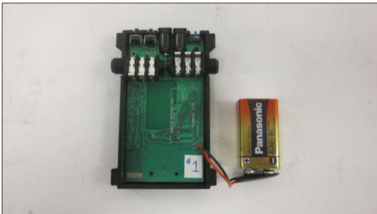
Photograph 4. bottom of PCB with Battery wout lower housing
