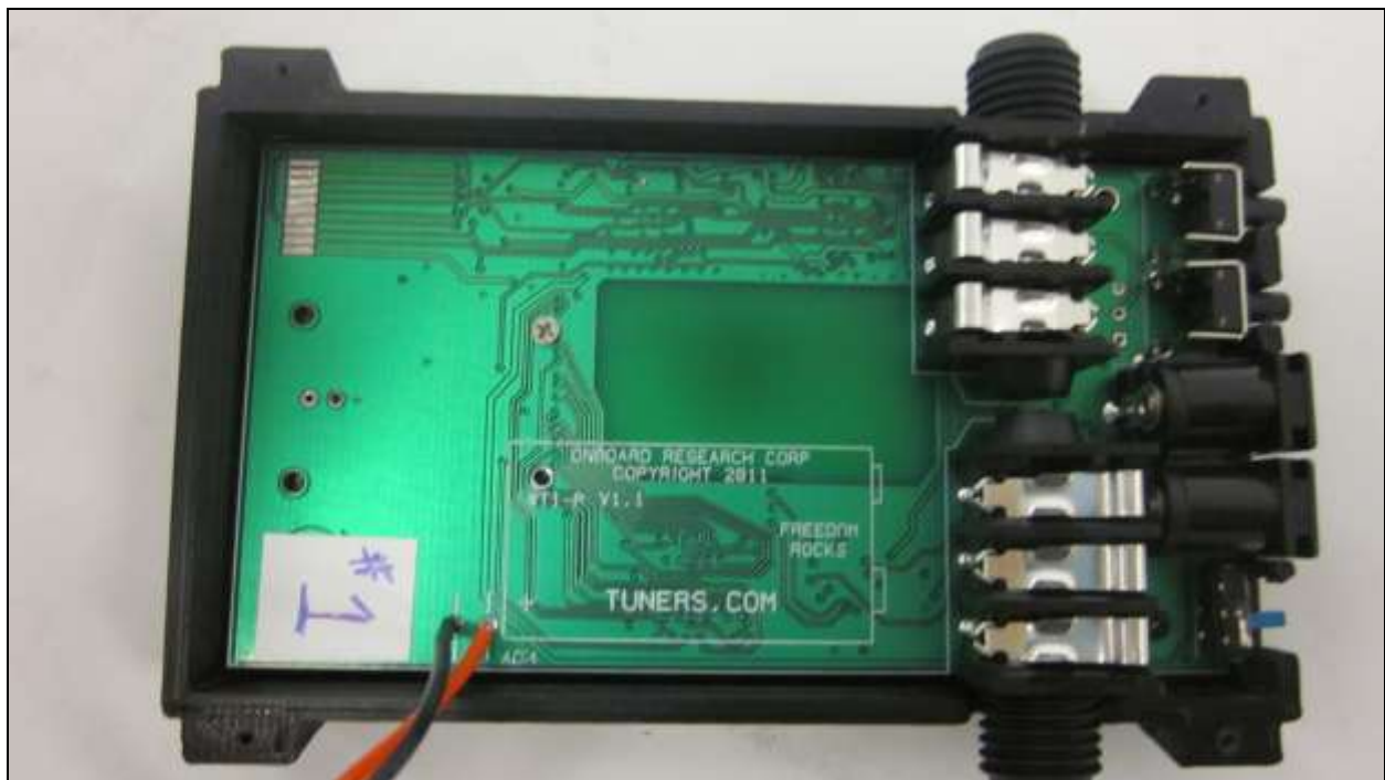
Photograph 6. bottom of PCB
