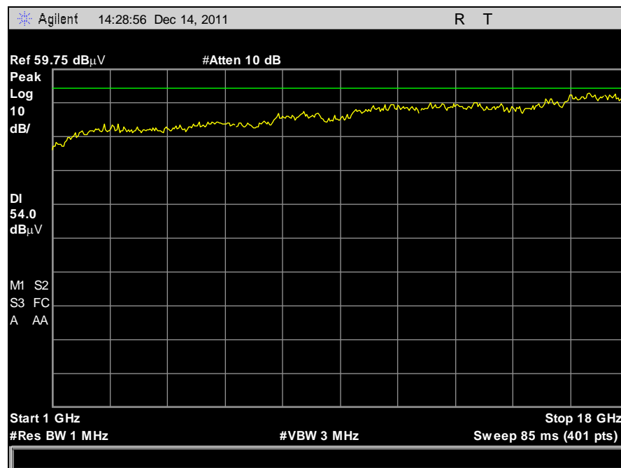
Plot 36. Receiver Spurious Emission, 1 GHz – 18 GHz
