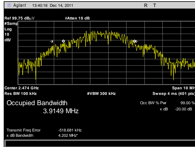
Plot 22. 99% Occupied Bandwidth, High Channel
