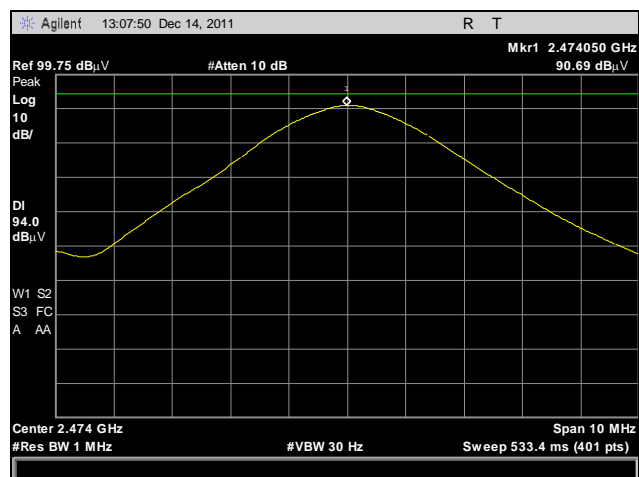
Plot 15. Field Strength of Fundamental, High Channel, Average
