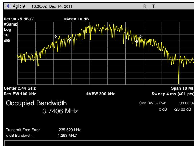
Plot 21. 99% Occupied Bandwidth, Mid Channel
