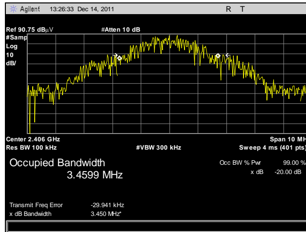
Plot 20. 99% Occupied Bandwidth, Low Channel
