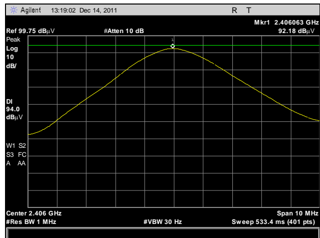
Plot 11. Field Strength of Fundamental, Low Channel, Average
