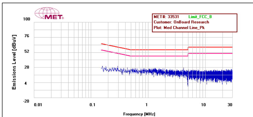
Plot 7. 15.207 Conducted Emissions, Mid Channel Line
