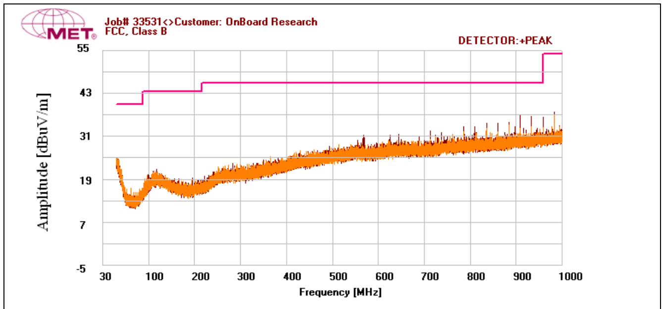
Plot 3. Radiated Emissions, Pre-Scan, 30 MHz – 1 GHz, FCC Limits
