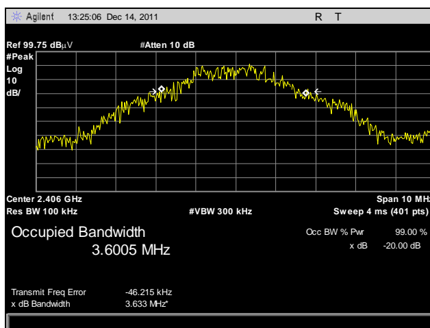
Plot 17. Occupied Bandwidth, Low Channel
