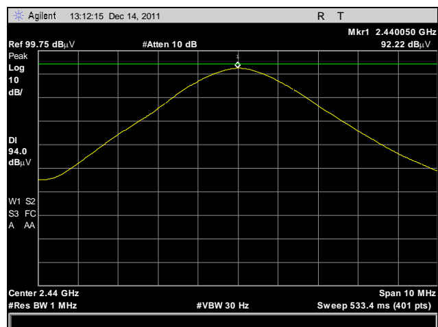
Plot 13. Field Strength of Fundamental, Mid Channel, Average
