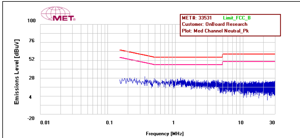
Plot 8. 15.207 Conducted Emissions, Mid Channel Neutral
