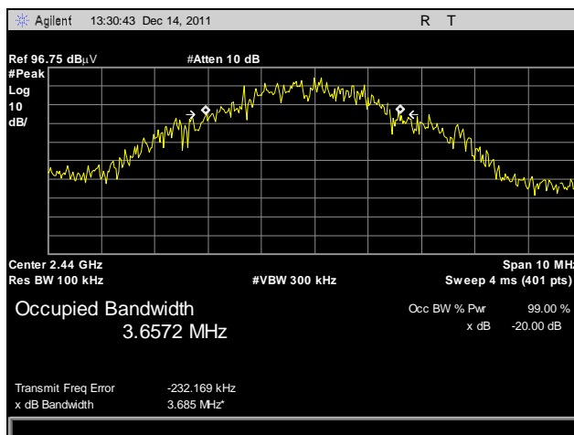
Plot 18. Occupied Bandwidth, Mid Channel
