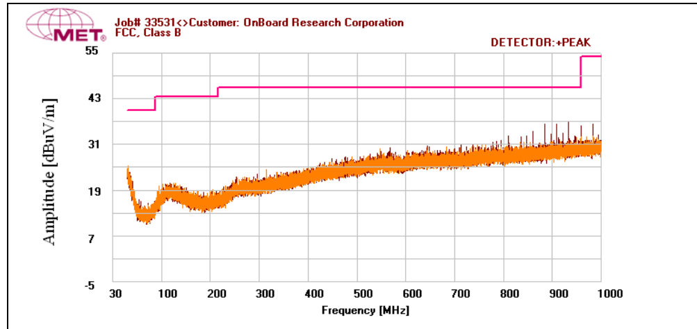
Plot 26. Radiated Spurious Emissions, Mid Channel, 30 MHz – 1 GHz, Peak Detector, Average Limit
