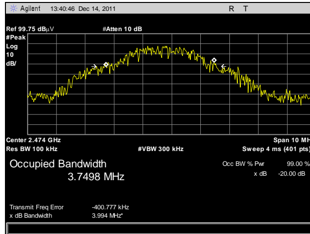
Plot 19. Occupied Bandwidth, High Channel
