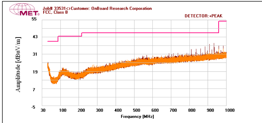
Plot 23. Radiated Spurious Emissions, Low Channel, 30 MHz – 1 GHz
