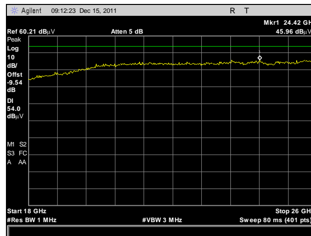
Plot 30. Radiated Spurious Emissions, High Channel, 18 GHz – 26 GHz, Peak Detector, Average Limit
