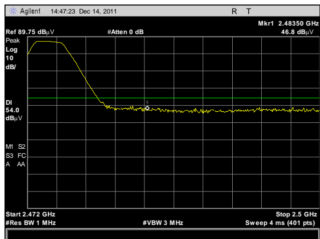
Plot 34. Restricted Band Emissions, High Channel, Peak Detector, Average Limit
