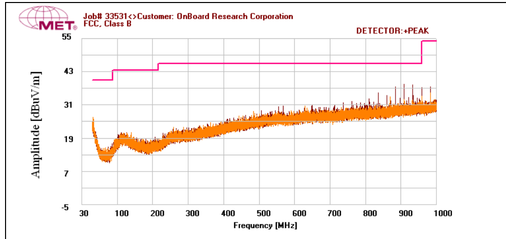
Plot 29. Radiated Spurious Emissions, High Channel, 30 MHz – 1 GHz, Peak Detector, Average Limit
