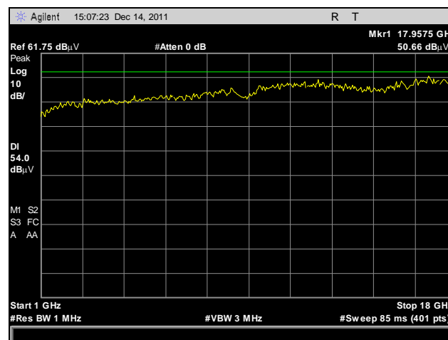
Plot 25. Radiated Spurious Emissions, Low Channel, 1-18GHz, Peak Detector, Average Limit
