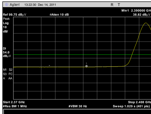
Plot 32. Restricted Band Emissions, Low Channel, Average Detector, Average Limit
