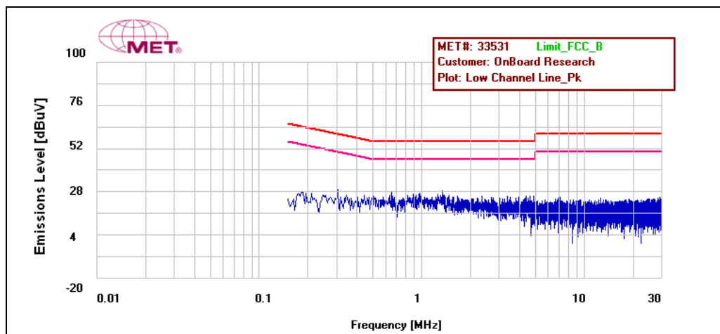
Plot 5. 15.207 Conducted Emissions, Low Channel Line
