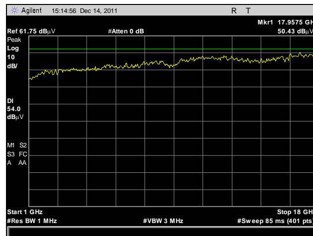
Plot 28. Radiated Spurious Emissions, Mid Channel, 1-18GHz, Peak Detector, Average Limit
