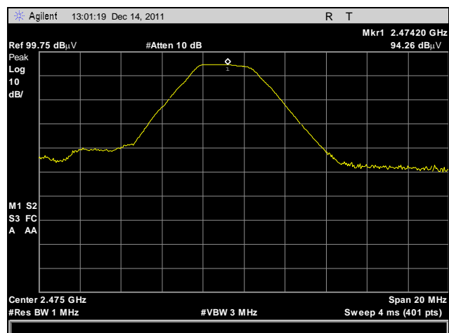
Plot 16. Field Strength of Fundamental, High Channel, Peak
