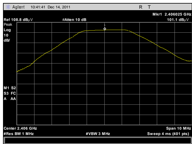
Plot 12. Field Strength of Fundamental, Low Channel, Peak Detector
