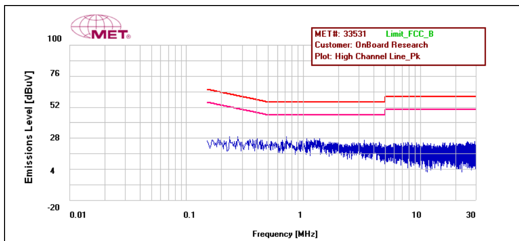
Plot 9. 15.207 Conducted Emissions, High Channel Line
