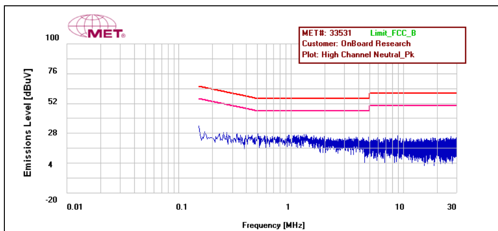
Plot 10. 15.207 Conducted Emissions, High Channel Neutral
