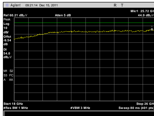
Plot 24. Radiated Spurious Emissions, Low Channel, 18 GHz – 26 GHz, Peak Detector, Average Limit
