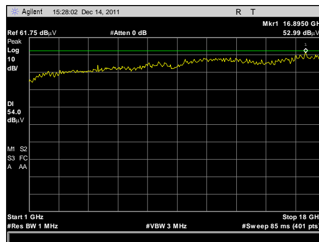
Plot 31. Radiated Spurious Emissions, High Channel, 1-18GHz, Peak Detector, Average Limit
