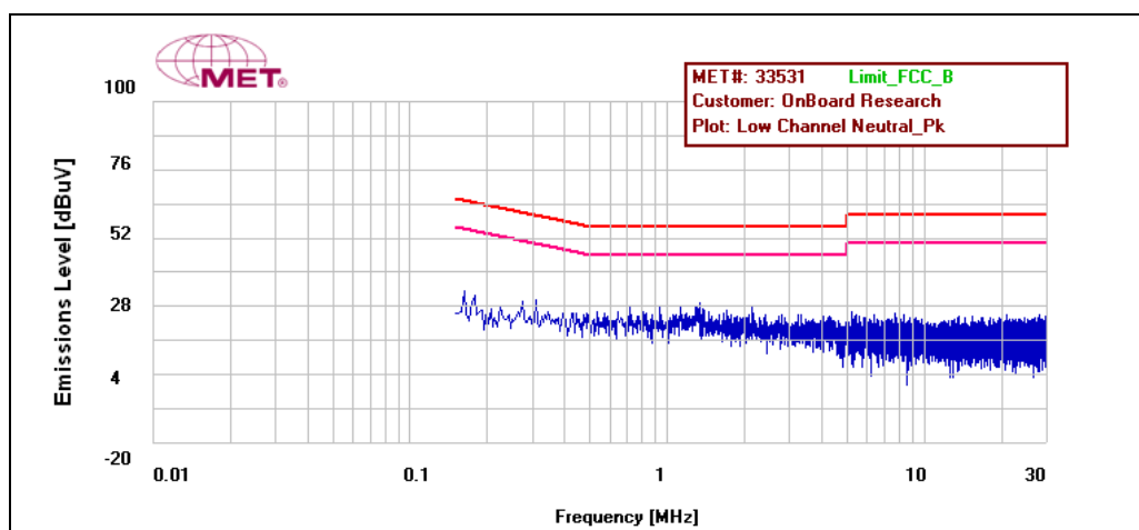
Plot 6. 15.207 Conducted Emissions, Low Channel Neutral
