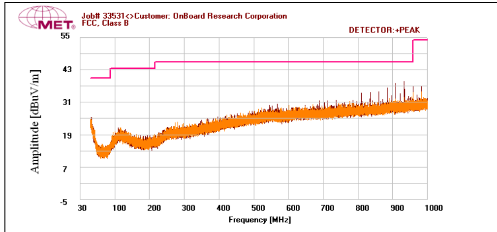
Plot 35. Receiver Spurious Emission, 30 MHz – 1 GHz
