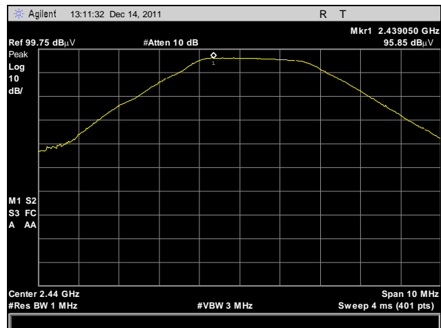
Plot 14. Field Strength of Fundamental, Mid Channel, Peak
