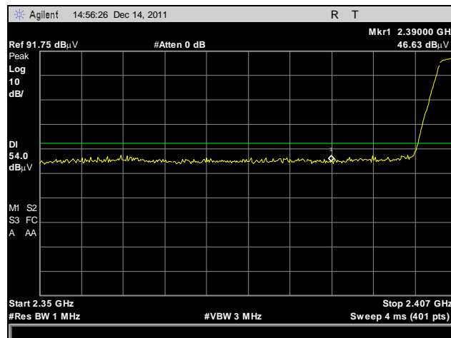
Plot 33. Restricted Band Emissions, Low Channel, Peak Detector, Average Limit
