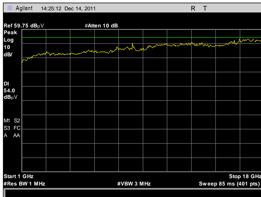
Plot 34. Receiver Spurious Emission, 1 GHz – 18 GHz
