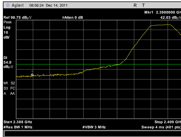
Plot 29. Restricted Band Emissions, Low Channel, Lower Span, Peak Detector, Average Limit
