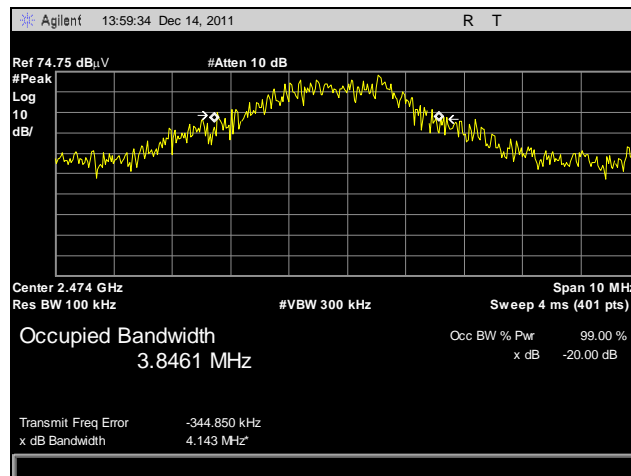
Plot 11. Occupied Bandwidth, High Channel
