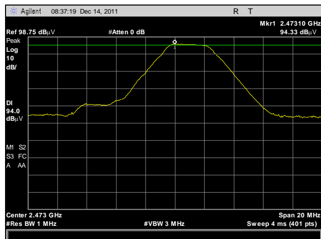
Plot 8. Field Strength of Fundamental, High Channel, Peak Detector, Average Limit
