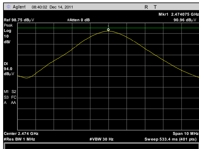
Plot 7. Field Strength of Fundamental, High Channel, Average Detector, Average Limit
