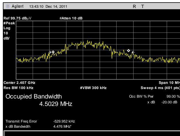
Plot 9. Occupied Bandwidth, Low Channel
