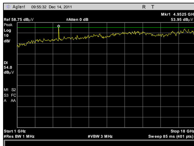
Plot 25. Radiated Spurious Emissions, High Channel, 1 GHz – 18 GHz, Peak Detector, Average Limit
