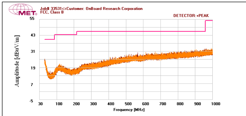
Plot 33. Receiver Spurious Emission, 30 MHz – 1 GHz
