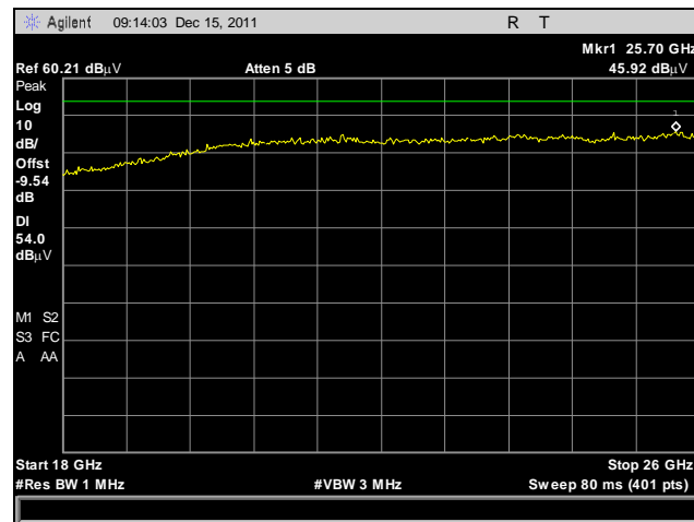
Plot 23. Radiated Spurious Emissions, Mid Channel, 18 GHz – 26 GHz, Peak Detector, Average Limit
