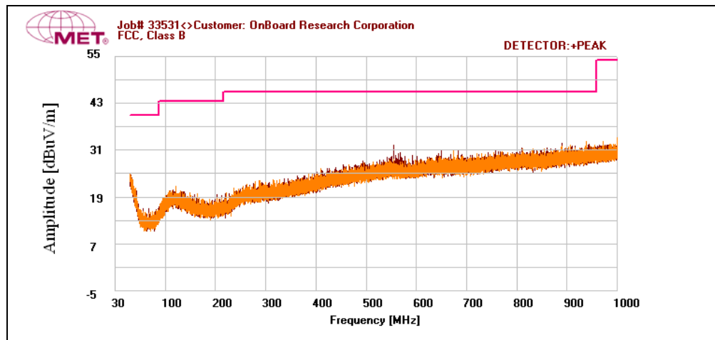
Plot 15. Radiated Spurious Emissions, Low Channel, 30 MHz – 1 GHz
