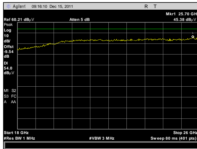
Plot 18. Radiated Spurious Emissions, Low Channel, 18 GHz – 26 GHz, Peak Detector, Average Limit
