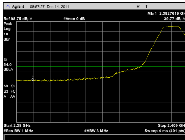
Plot 30. Restricted Band Emissions, Low Channel, Higher Span
