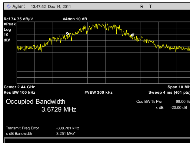
Plot 10. Occupied Bandwidth, Mid Channel
