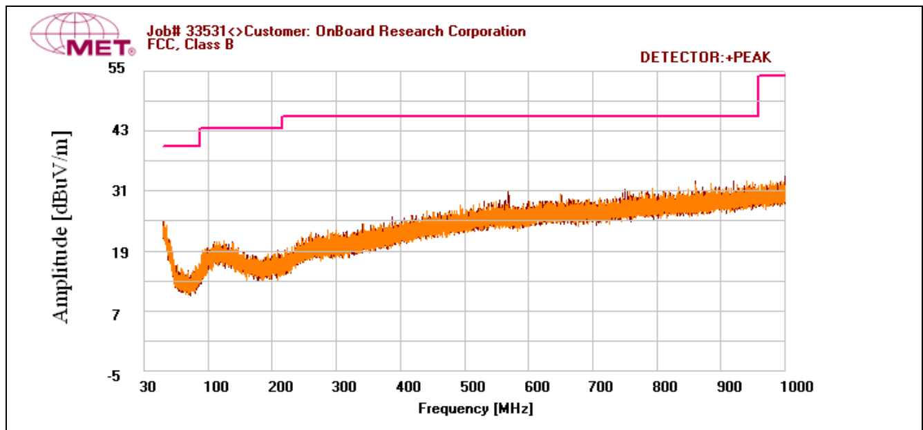
Plot 1. Radiated Emissions, Pre-Scan, 30 MHz – 1 GHz, FCC Limits
