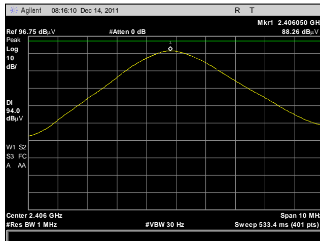
Plot 3. Field Strength of Fundamental, Low Channel, Average Detector, Average Limit
