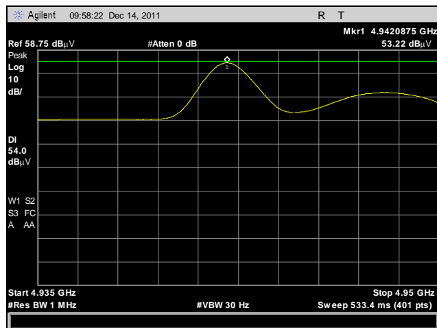
Plot 28. Radiated Spurious Emissions, High Channel, Average, 4.935 GHz – 4.950 GHz
