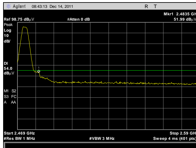
Plot 31. Restricted Band Emissions, High Channel, Peak Detector, Average Limit
