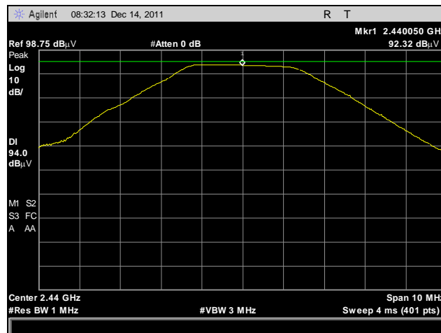
Plot 6. Field Strength of Fundamental, Mid Channel, Peak Detector, Average Limit
