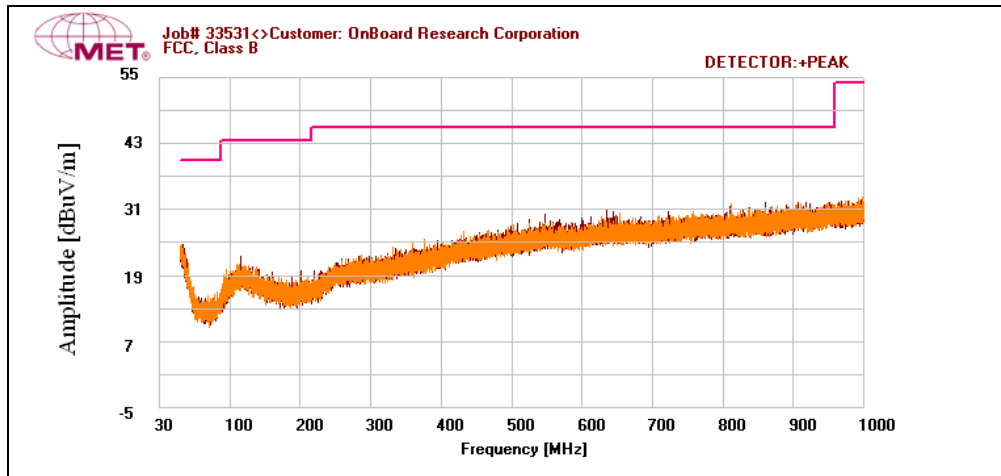
Plot 20. Radiated Spurious Emissions, Mid Channel, 30 MHz – 1 GHz
