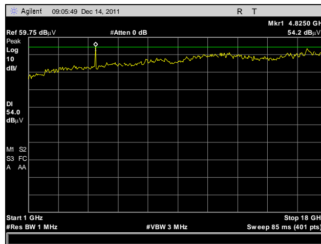
Plot 16. Radiated Spurious Emissions, Low Channel, 1 GHz – 18 GHz, Peak Detector, Average Limit
