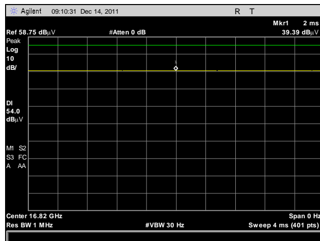
Plot 19. Radiated Spurious Emissions, Low Channel, Average Spurious @ 16.82 GHz
