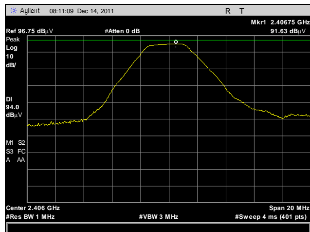
Plot 4. Field Strength of Fundamental, Low Channel, Peak Detector, Average Limit
