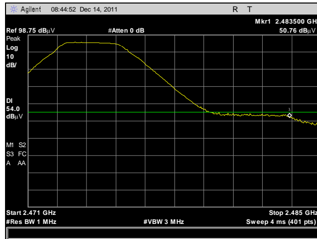
Plot 32. Restricted Band Emissions, High Channel, Lower Span
