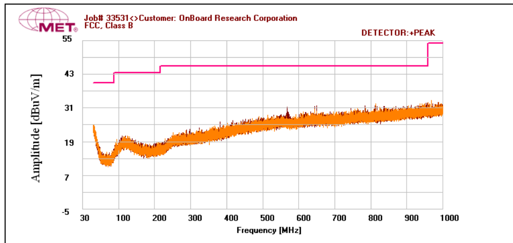
Plot 24. Radiated Spurious Emissions, High Channel, 30 MHz – 1 GHz
