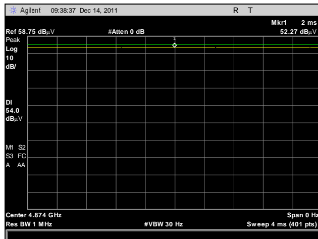
Plot 22. Radiated Spurious Emissions, Mid Channel, 2 nd Harmonic, Average Detector, Average Limit
