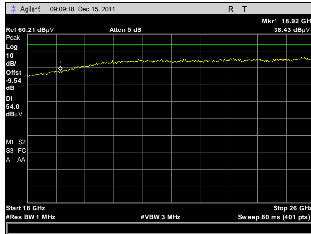
Plot 27. Radiated Spurious Emissions, High Channel, 18 GHz – 26 GHz, Peak Detector, Average Limit
