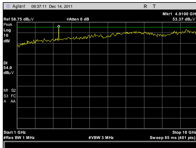
Plot 21. Radiated Spurious Emissions, Mid Channel, 1 GHz – 18 GHz, Peak Detector, Average Limit
