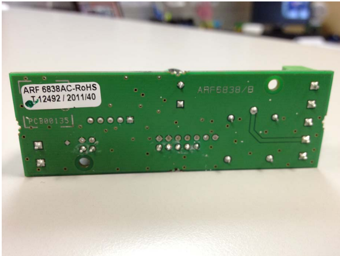
Receiver Board: Foil Side
