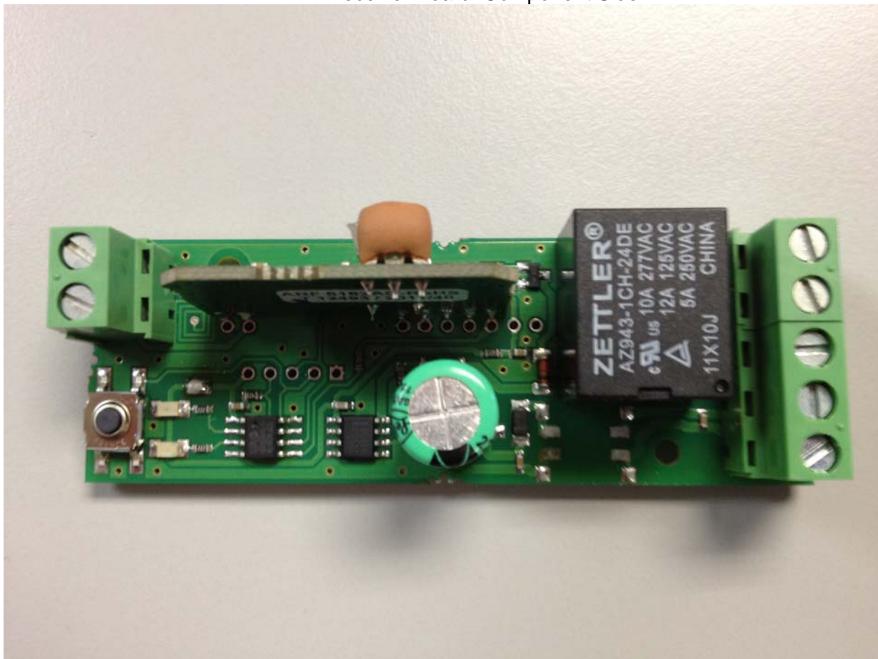
Receiver Board: Component Side
