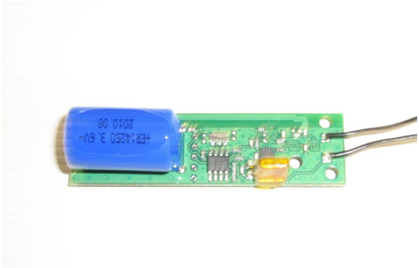
Photograph of Transmitter Board: Foil Side
