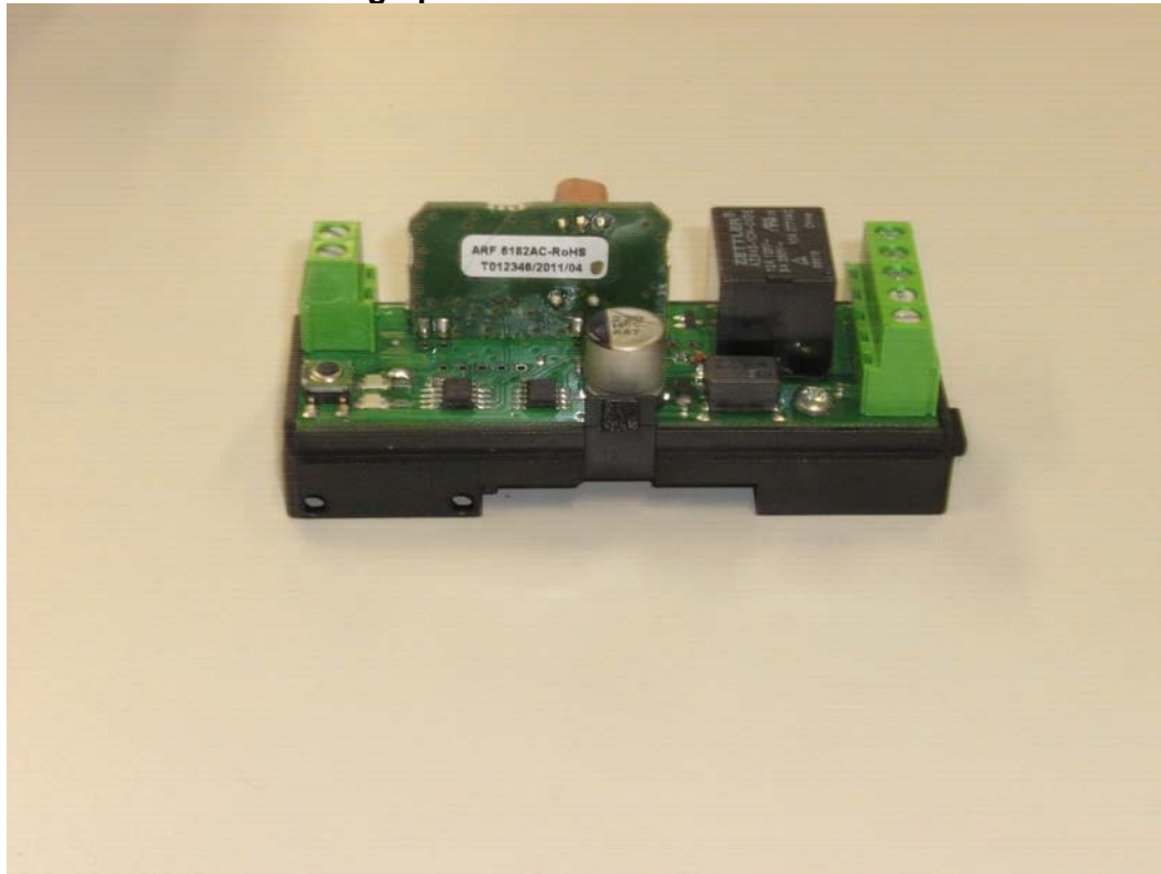
Receiver Board: Component Side
