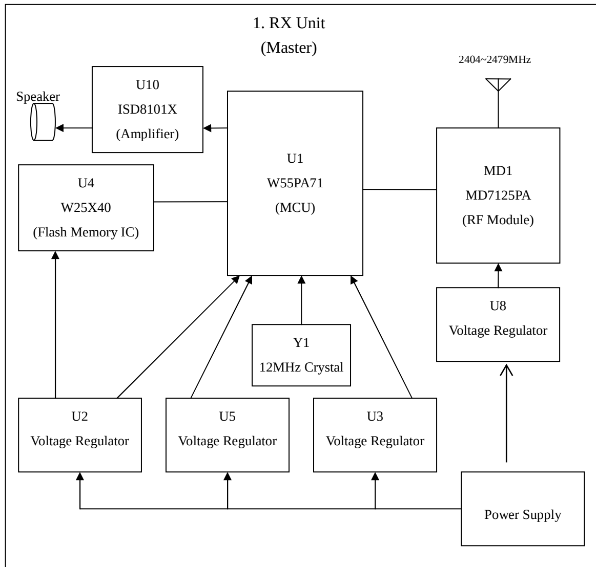
Security System Block Diagram
