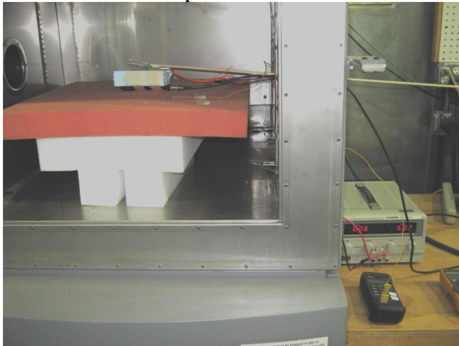
Temperature Chamber
